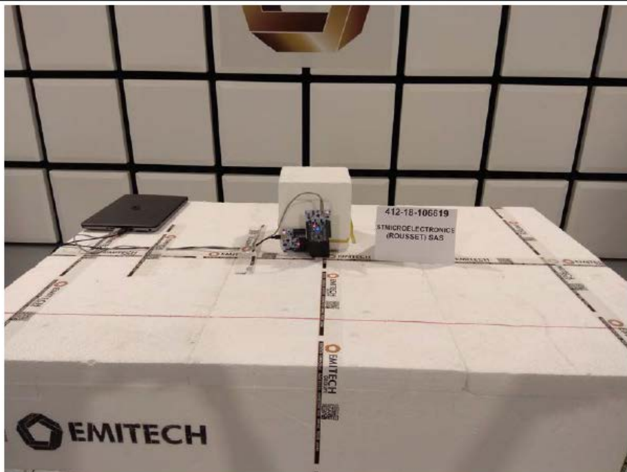
TEST SETUP PHOTO(S) RADIATED EMISSIONS (CARD EMUL)
