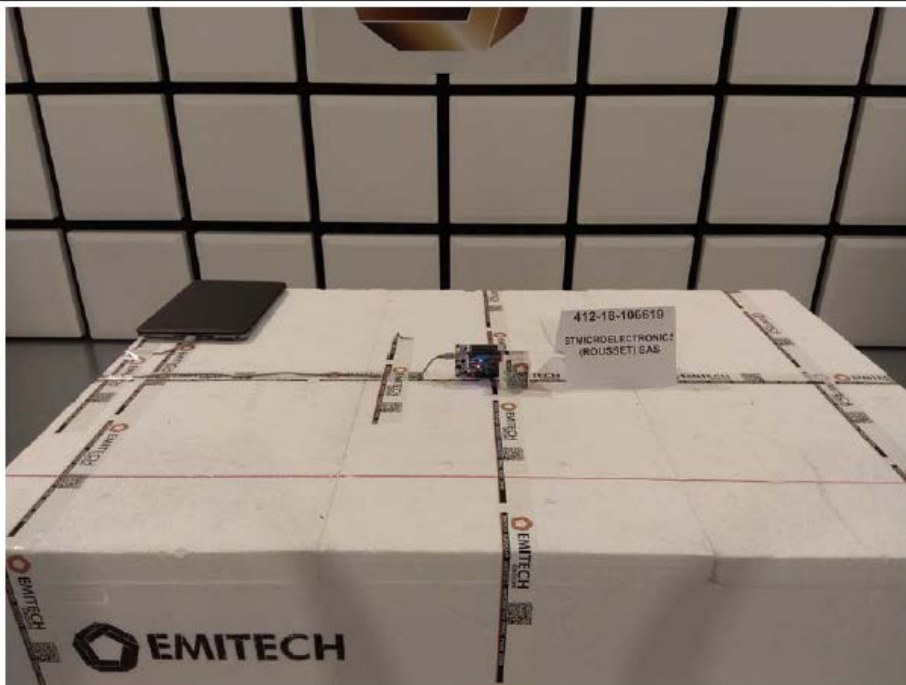
TEST SETUP PHOTO(S) RADIATED EMISSIONS (CONFIG TAG)
