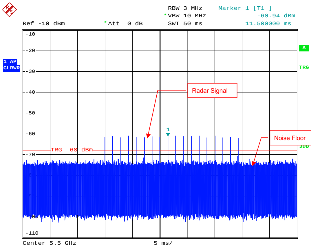
Radar Signal 1
