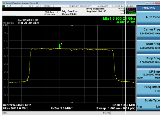
Plot 7-400. Power Spectral Density Plot Antenna WF7 LPI (80MHz 802.11ax (UNII Band 8) – Ch. 199, MCS4)
