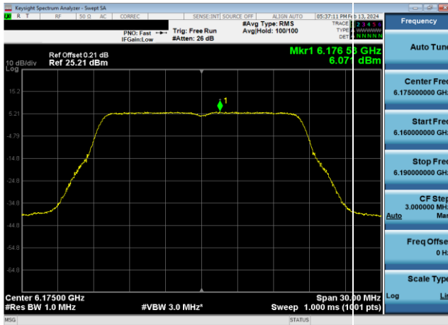
Plot 7-432. Power Spectral Density Plot Antenna WF7 Standard Power (20MHz 802.11a (UNII Band 5) – Ch. 45, 24Mbps)
