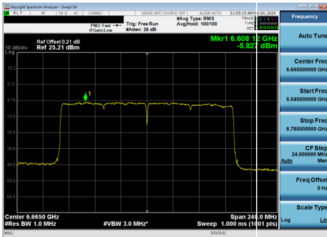
Plot 7-396. Power Spectral Density Plot Antenna WF7 LPI (160MHz 802.11ax (UNII Band 7) – Ch. 143, MCS4)
