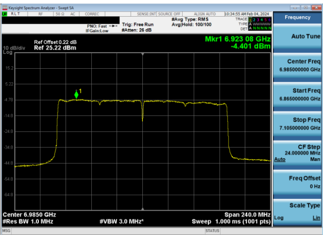
Plot 7-381. Power Spectral Density Plot Antenna WF7 LPI (160MHz 802.11ax (UNII Band 8) – Ch. 207, MCS2)
