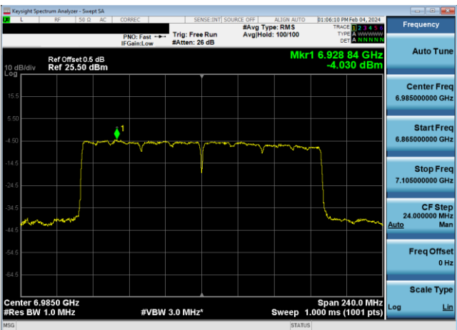
Plot 7-421. Power Spectral Density Plot Antenna WF7 LPI (160MHz 802.11ax (UNII Band 8) – Ch. 207, MCS11)
