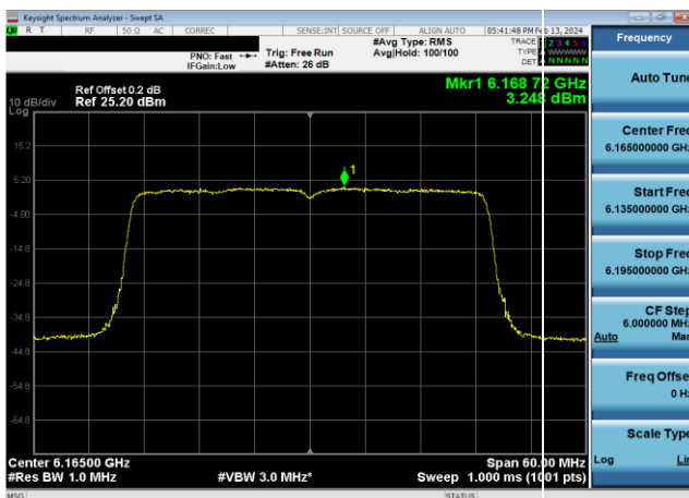
Plot 7-434. Power Spectral Density Plot Antenna WF7 Standard Power (40MHz 802.11ax (UNII Band 5) – Ch. 43, MCS4)
