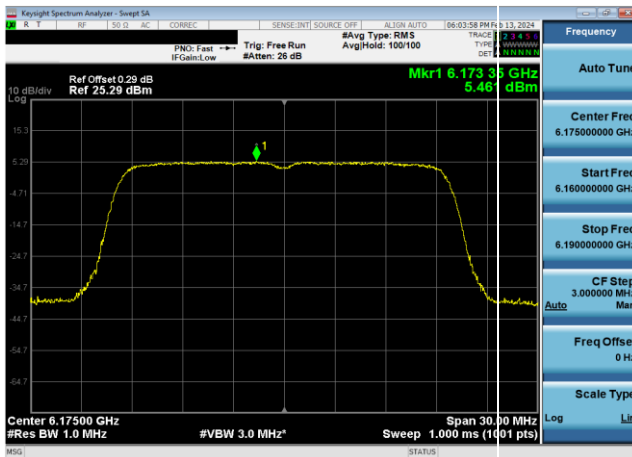
Plot 7-443. Power Spectral Density Plot Antenna WF7 Standard Power (20MHz 802.11ax (UNII Band 5) – Ch. 45, MCS11)
