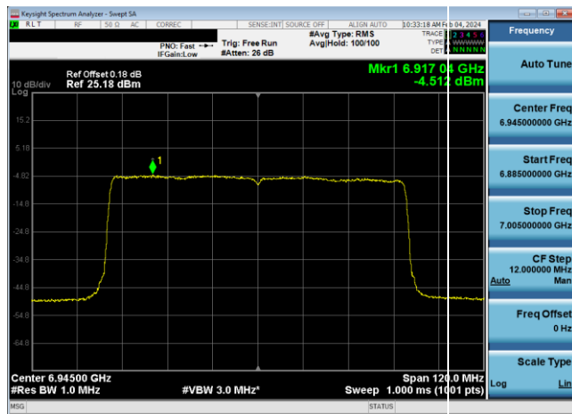
Plot 7-380. Power Spectral Density Plot Antenna WF7 LPI (80MHz 802.11ax (UNII Band 8) – Ch. 199, MCS2)
