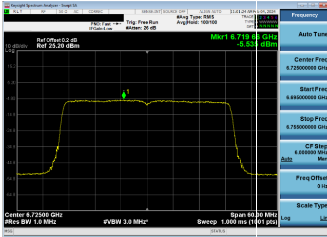
Plot 7-394. Power Spectral Density Plot Antenna WF7 LPI (40MHz 802.11ax (UNII Band 7) – Ch. 155, MCS4)
