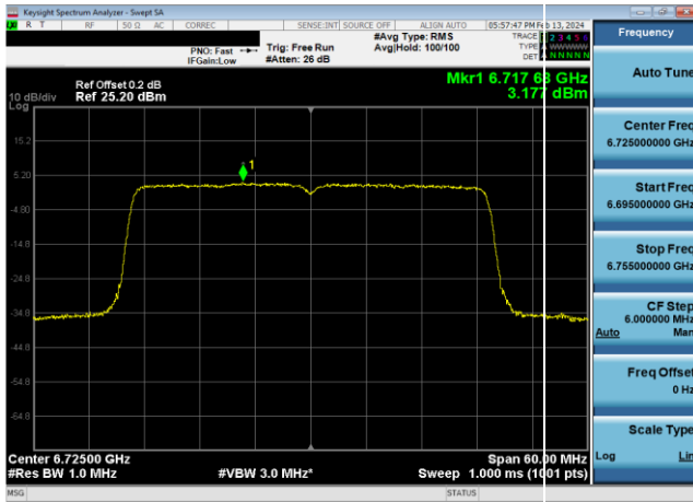
Plot 7-439. Power Spectral Density Plot Antenna WF7 Standard Power (40MHz 802.11ax (UNII Band 7) – Ch. 155, MCS4)
