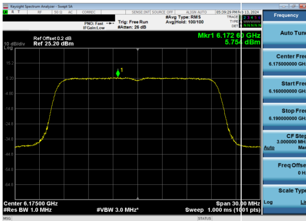
Plot 7-433. Power Spectral Density Plot Antenna WF7 Standard Power (20MHz 802.11ax (UNII Band 5) – Ch. 45, MCS4)
