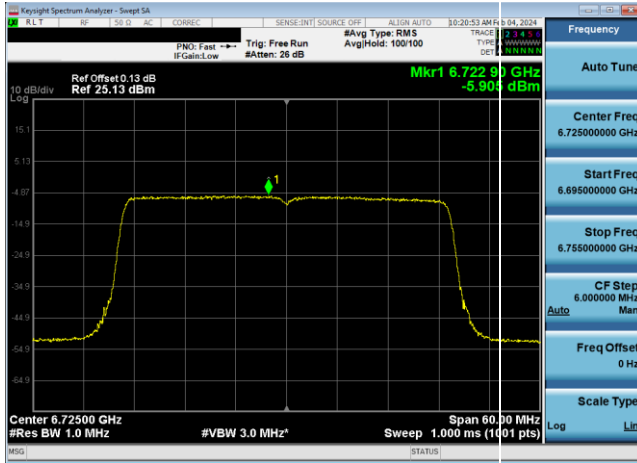
Plot 7-374. Power Spectral Density Plot Antenna WF7 LPI (40MHz 802.11ax (UNII Band 7) – Ch. 155, MCS2)
