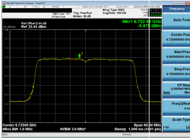
Plot 7-414. Power Spectral Density Plot Antenna WF7 LPI (40MHz 802.11ax (UNII Band 7) – Ch. 155, MCS11)
