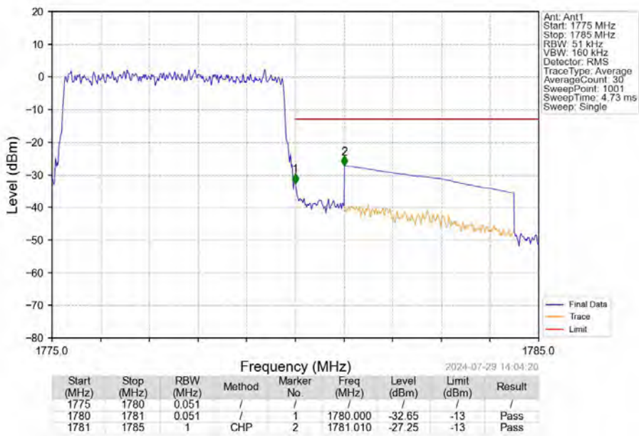
Band66_5MHz_16QAM_HCH_1777.5MHz_RB_25_0_NTNV
