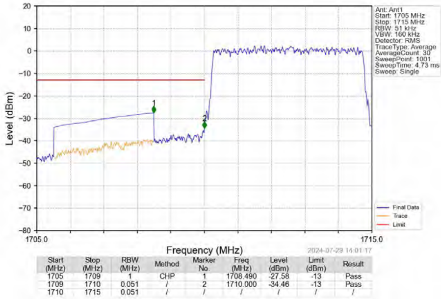
Band66_5MHz_16QAM_LCH_1712.5MHz_RB_25_0_NTNV
