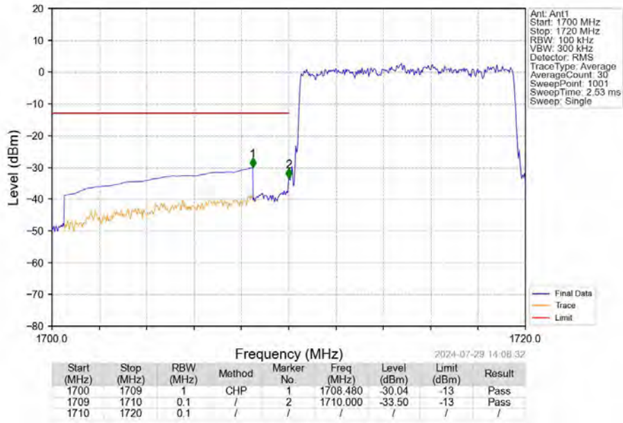
Band66_10MHz_16QAM_LCH_1715MHz_RB_50_0_NTNV
