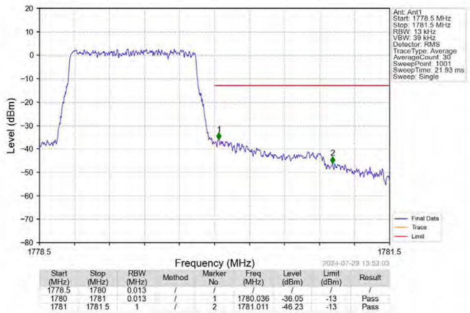
Band66 1.4MHz QPSK HCH 1779.3MHz RB 6 0 NTNV
