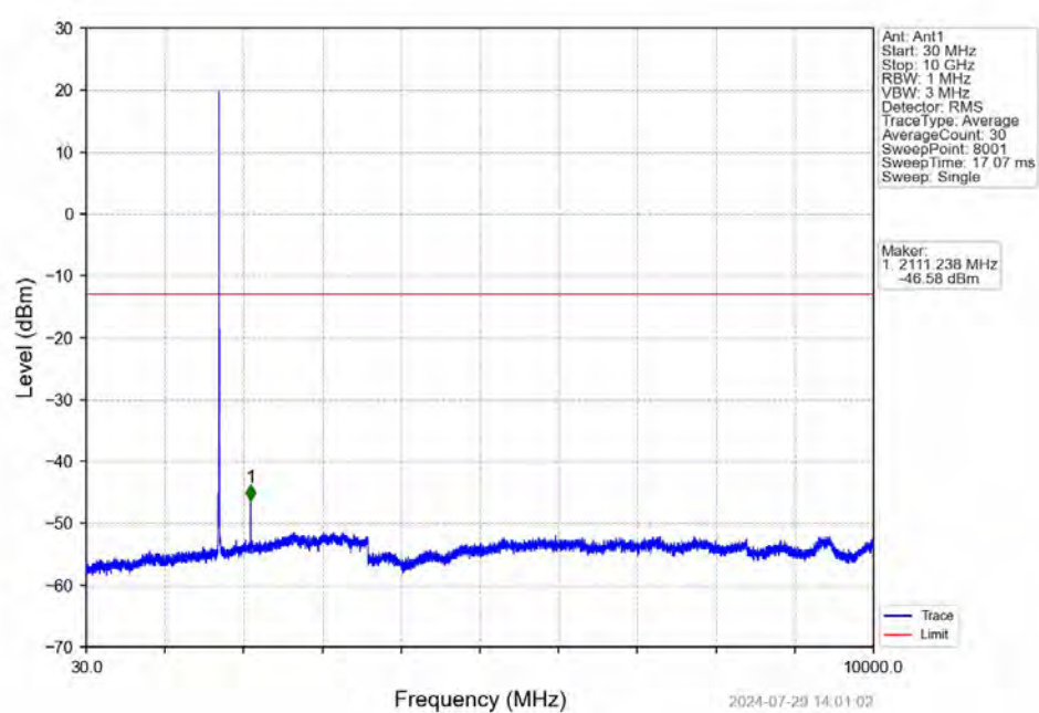
Band66_5MHz_16QAM_LCH_1712.5MHz_RB_1_0_NTNV
