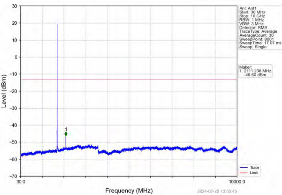
Band66_3MHz_16QAM_LCH_1711.5MHz_RB_1_0_NTNV
