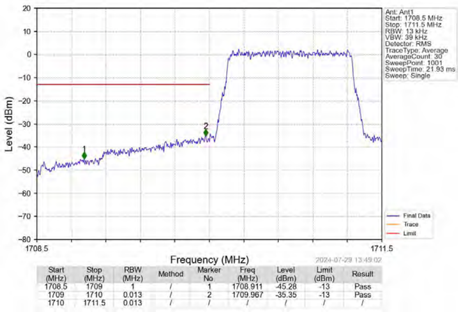
Band66_1.4MHz_16QAM_LCH_1710.7MHz_RB_6_0_NTNV
