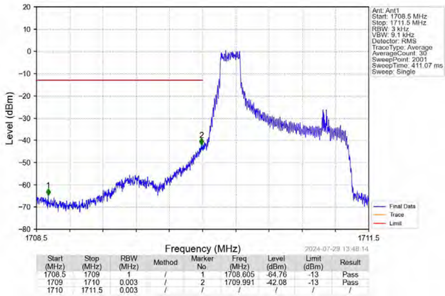
Band66_1.4MHz_16QAM_LCH_1710.7MHz_RB_1_0_NTNV
