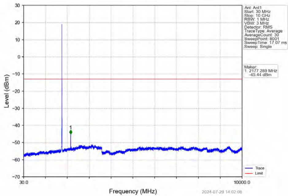
Band66_5MHz_QPSK_HCH_1777.5MHz_RB_1_0_NTNV
