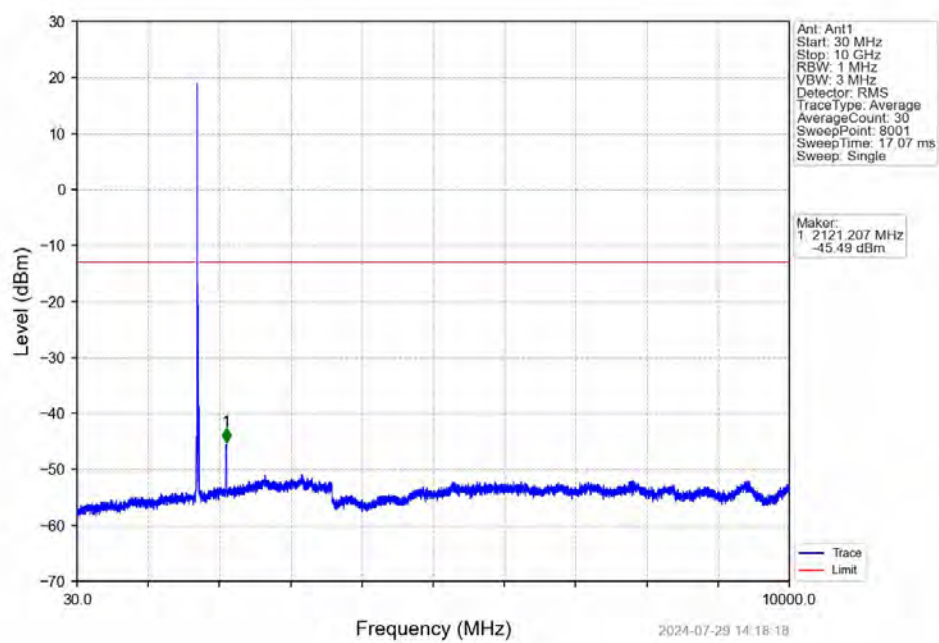
Band66_15MHz_16QAM_LCH_1717.5MHz_RB_1_0_NTNV
