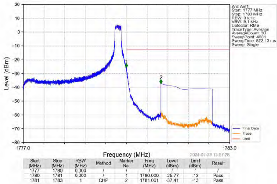
Band66_3MHz_QPSK_HCH_1778.5MHz_RB_1_14_NTNV
