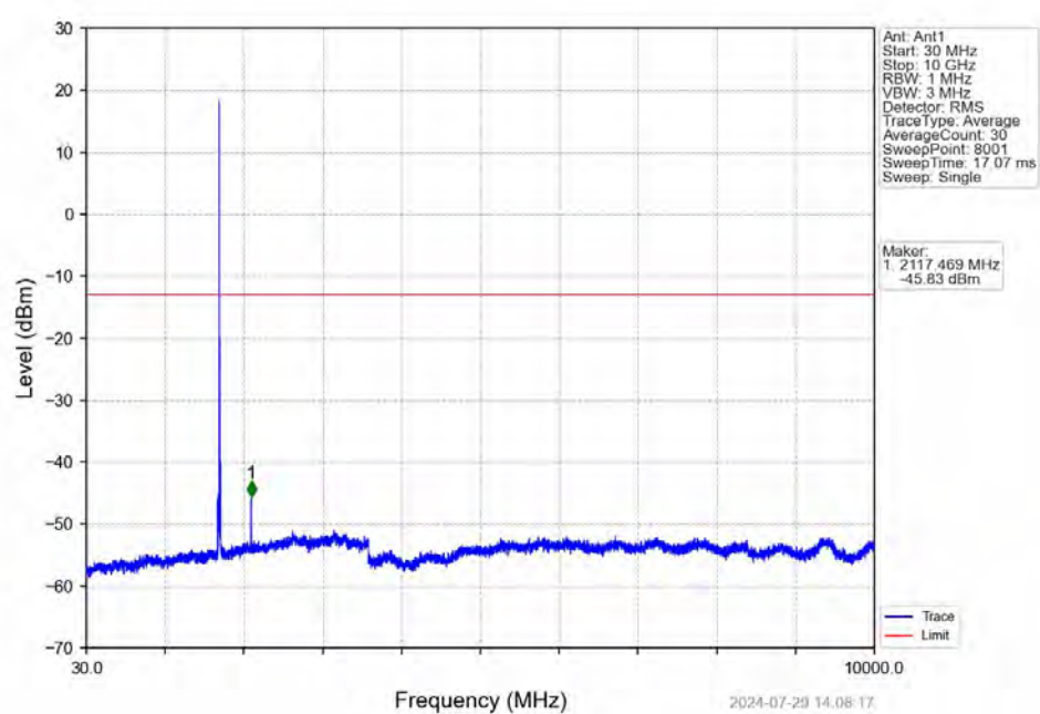
Band66_10MHz_16QAM_LCH_1715MHz_RB_1_0_NTNV
