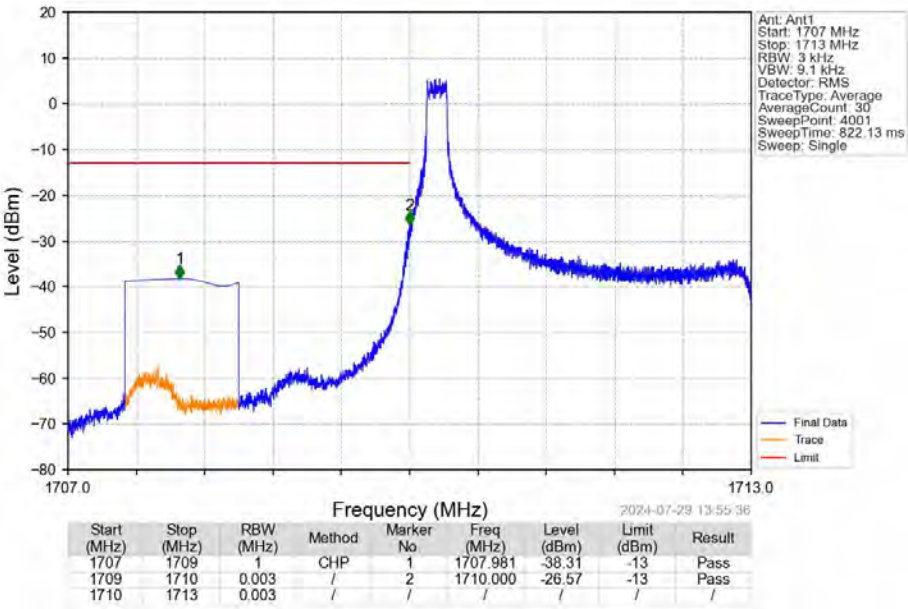
Band66_3MHz_16QAM_LCH_1711.5MHz_RB_1_0_NTNV
