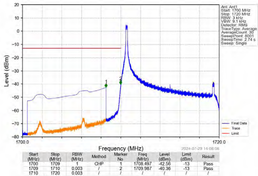
Band66_10MHz_16QAM_LCH_1715MHz_RB_1_0_NTNV
