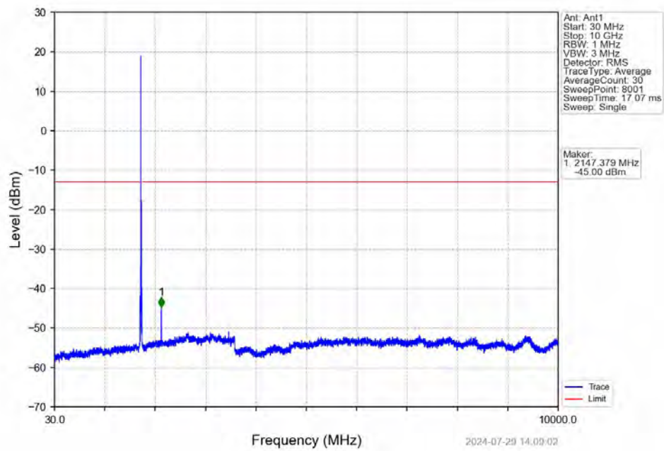
Band66_10MHz_16QAM_MCH_1745MHz_RB_1_0_NTNV
