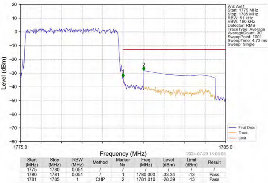
Band66_5MHz_QPSK_HCH_1777.5MHz_RB_25_0_NTNV
