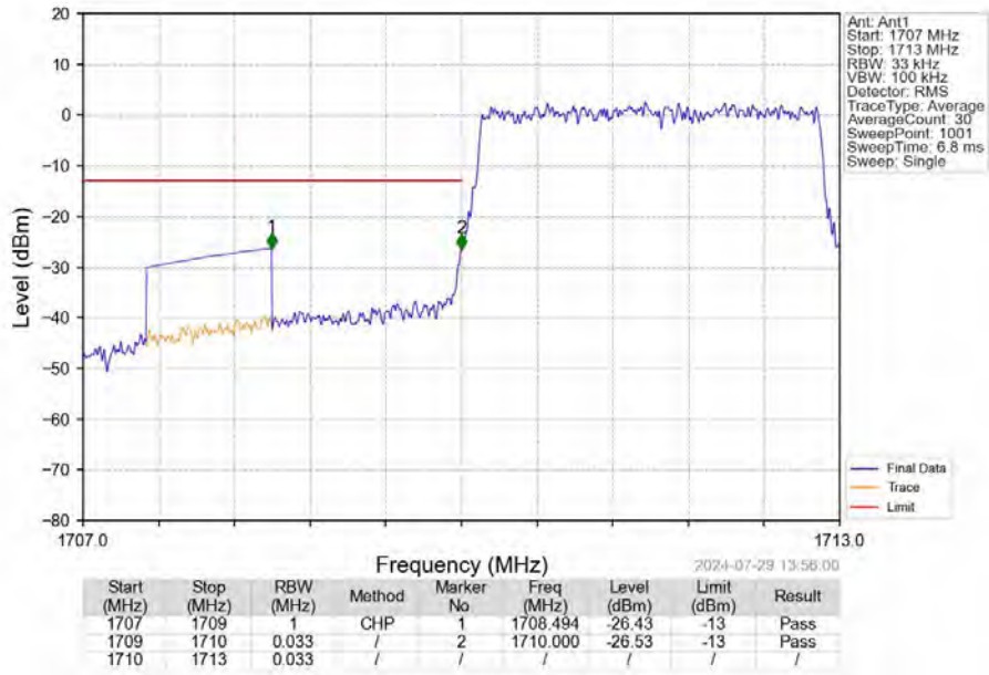
Band66_3MHz_16QAM_LCH_1711.5MHz_RB_15_0_NTNV
