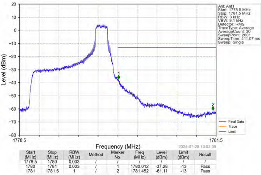
Band66_1.4MHz_16QAM_HCH_1779.3MHz_RB_1_5_NTNV
