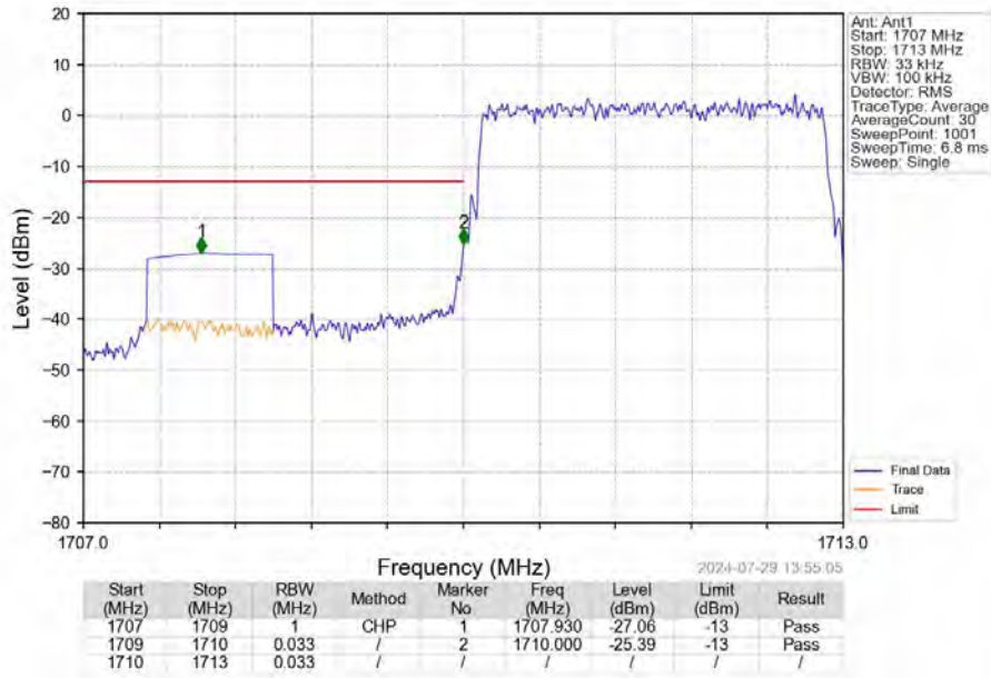
Band66_3MHz_QPSK_LCH_1711.5MHz_RB_15_0_NTNV
