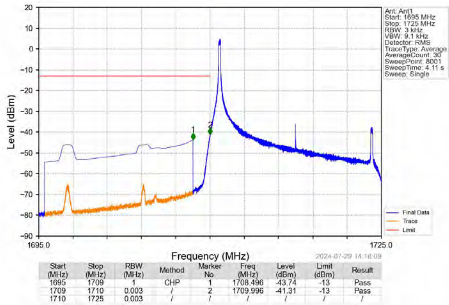
Band66_15MHz_16QAM_LCH_1717.5MHz_RB_1_0_NTNV
