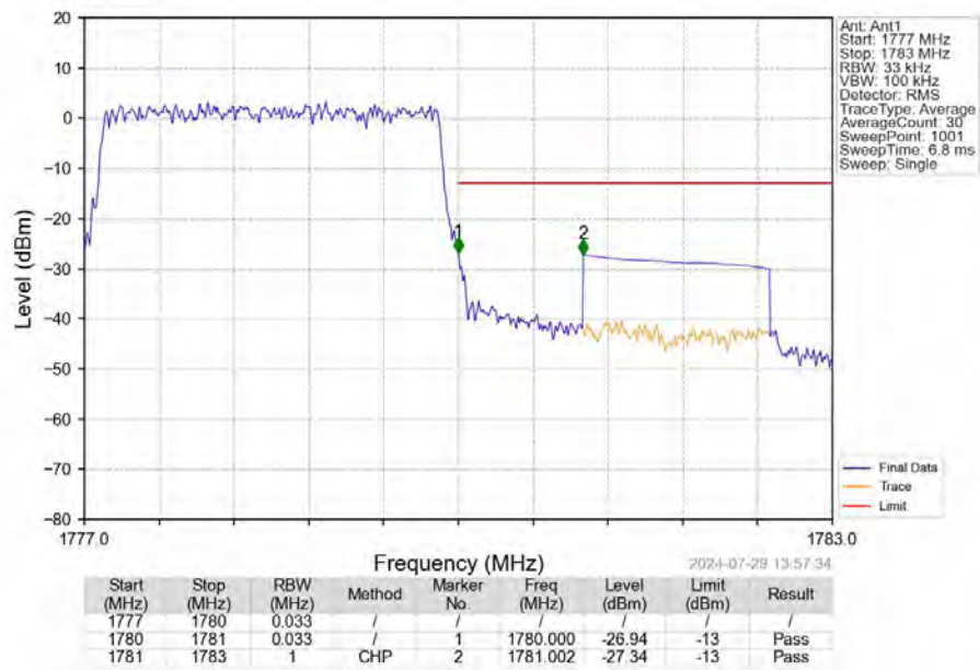
Band66_3MHz_QPSK_HCH_1778.5MHz_RB_15_0_NTNV
