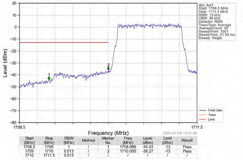
Band66_1.4MHz_QPSK_LCH_1710.7MHz_RB_6_0_NTNV
