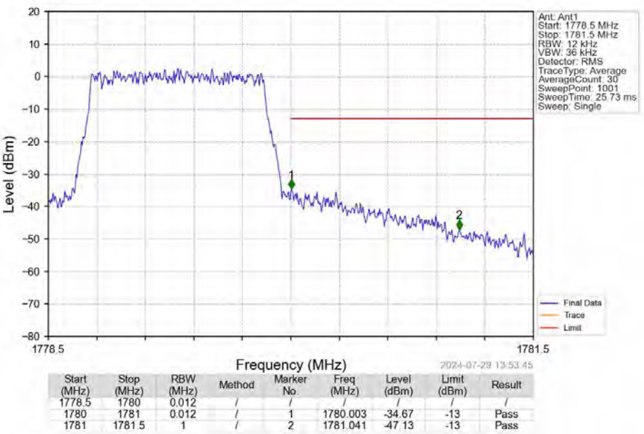
Band66_1.4MHz_16QAM_HCH_1779.3MHz_RB_6_0_NTNV
