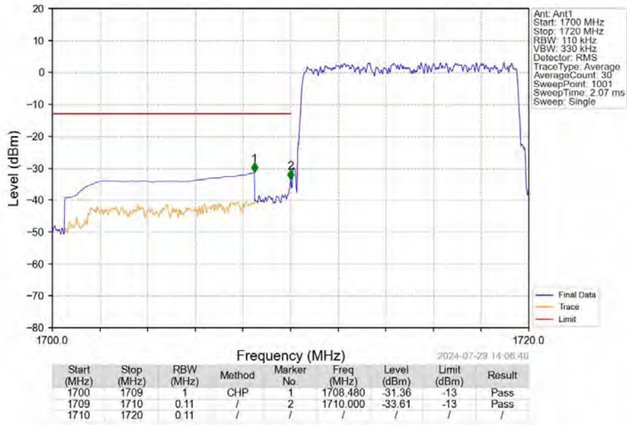
Band66_10MHz_QPSK_LCH_1715MHz_RB_50_0_NTNV
