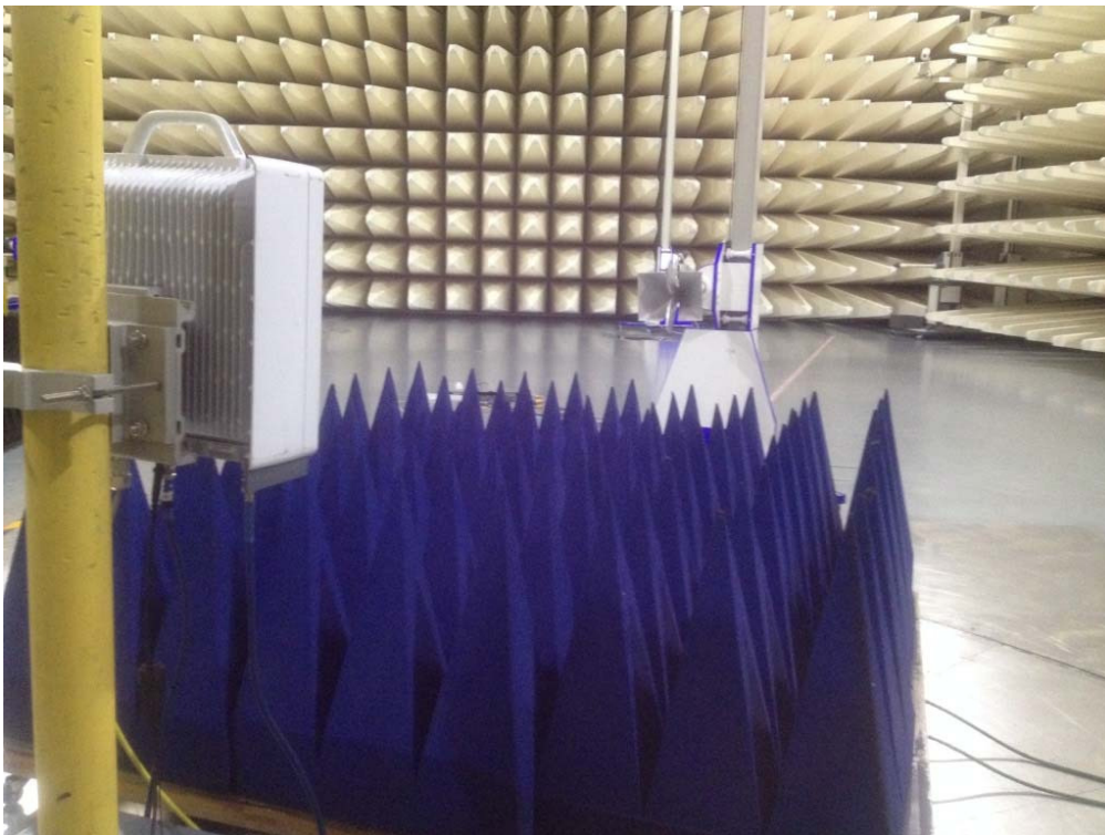
Radiated Emissions
