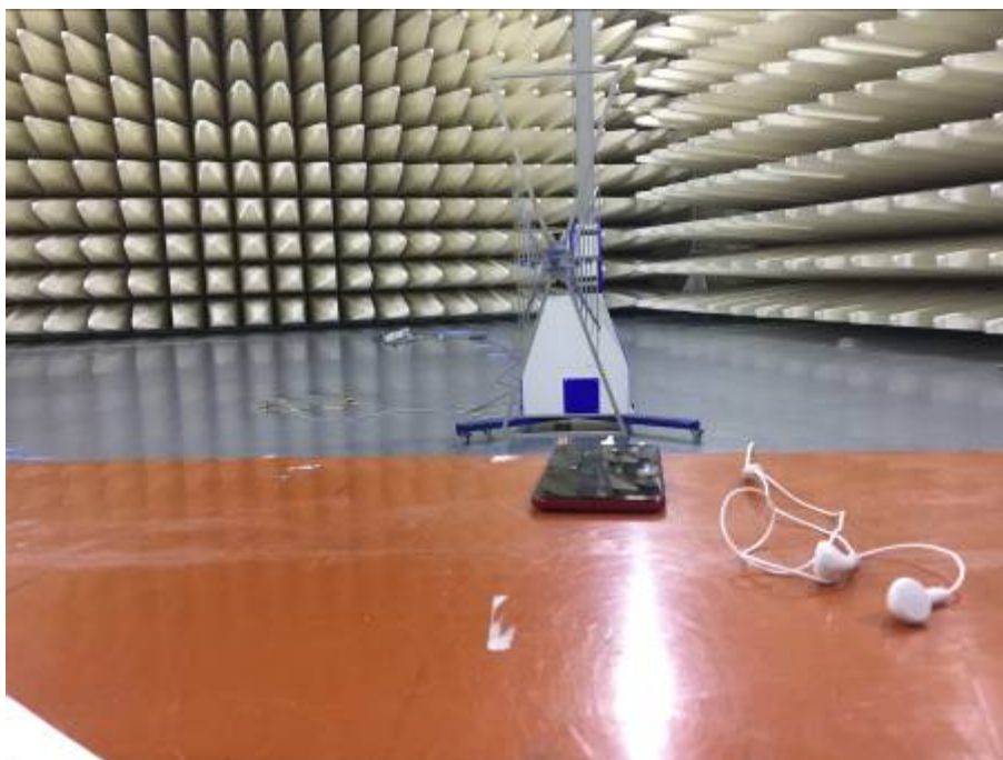
Spurious Radiated Emissions Test setup (with charger)
