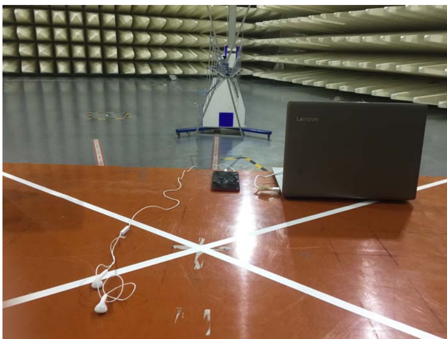
Spurious Radiated Emissions Test setup (with laptop)
