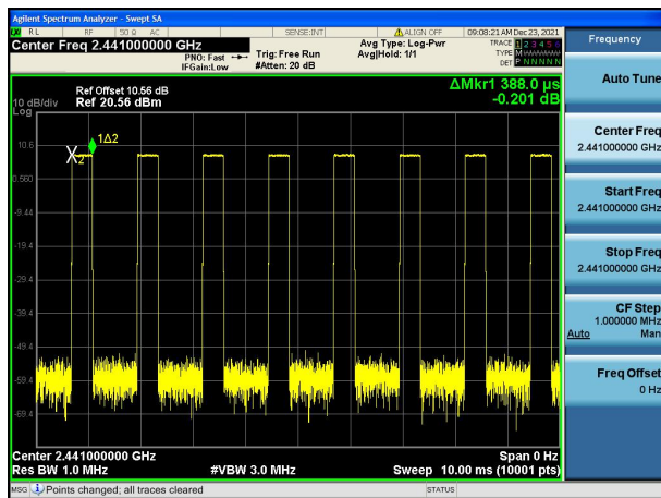
Modulation: GFSK DH1 2441MHz
