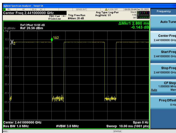
Modulation: GFSK DH5 2441MHz
