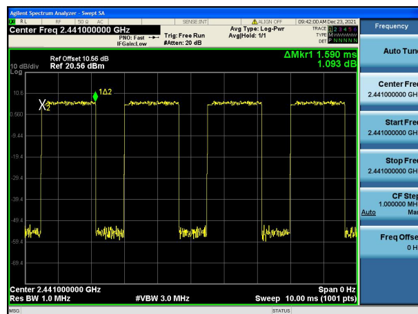
Modulation: 8DPSK 3DH3 2441MHz
