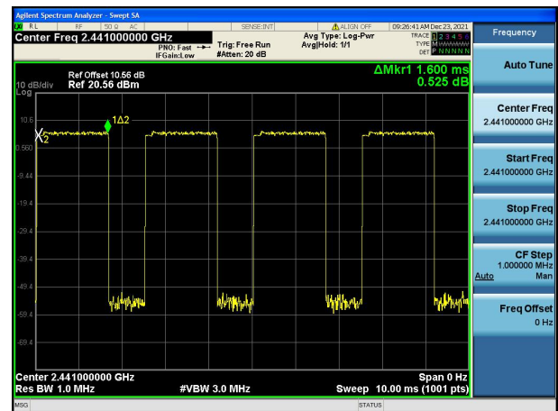
Modulation: \pi/4 DQPSK 2DH3 2441MHz
