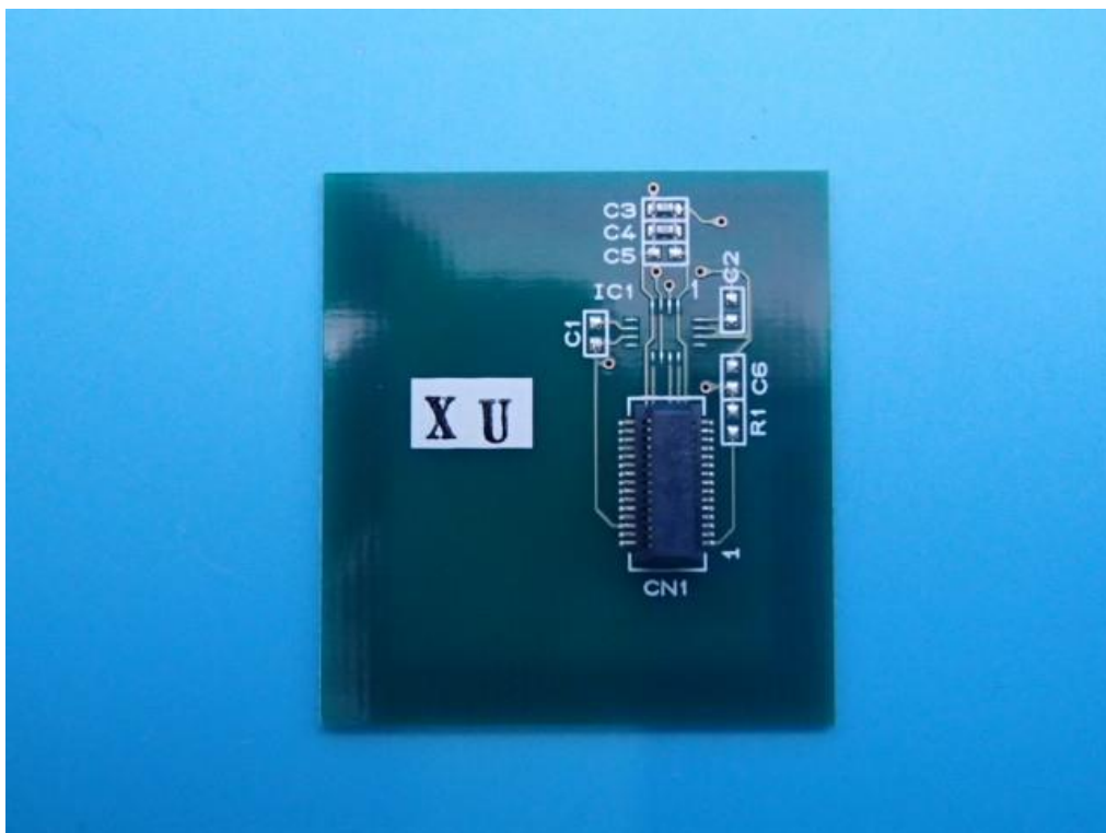
NFC antenna board assembly
