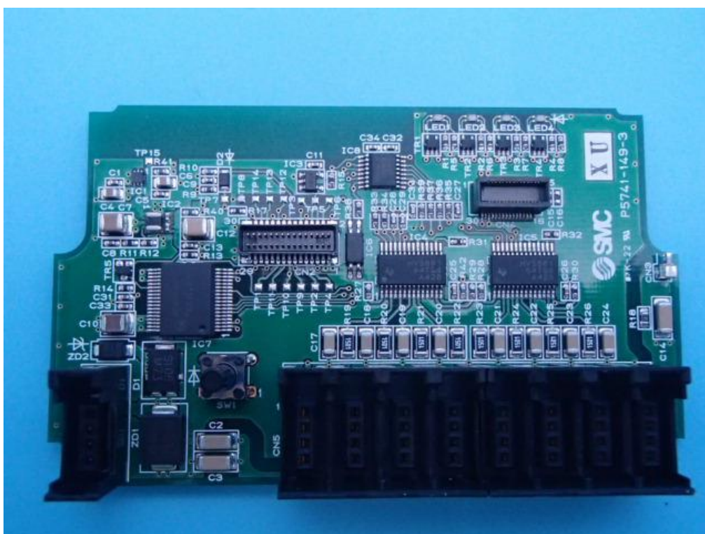
EX6000-WDXE1 Inside view
