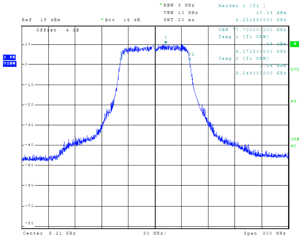
Figure 14 Plot of Transmitter Emissions (5150-5250 MHz Band, 80 MHz Chnl, Chain 0, 99% OBW)
