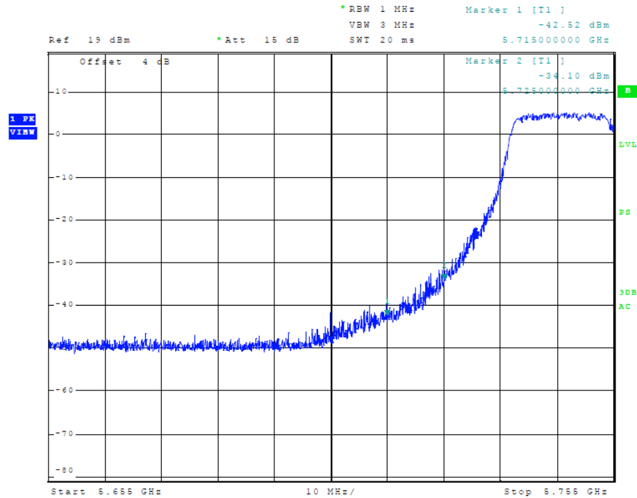
Figure 19 Plot of Transmitter Low Band Edge (5725-5850 MHz Band, 40 MHz Chnl, Chain 0)
