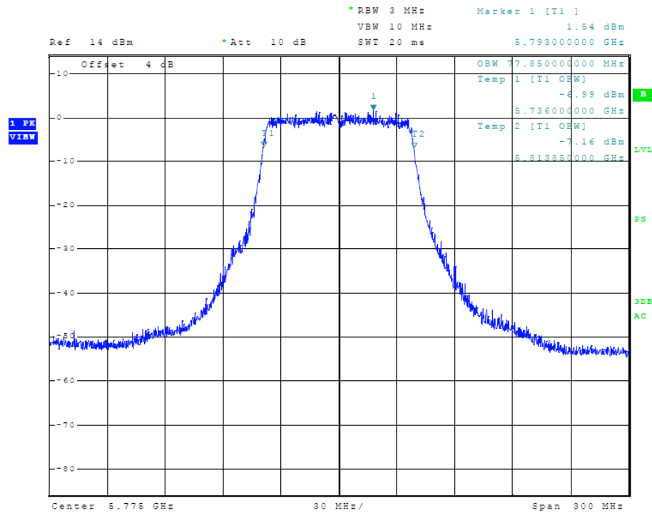
Figure 55 Plot of Transmitter Emissions (5725-5850 MHz Band, 80 MHz Chnl, Chain 1, 99% OBW)
