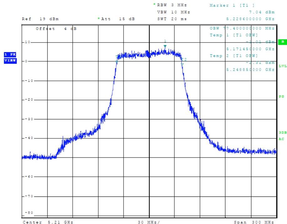
Figure 68 Plot of Transmitter Emissions (5150-5250 MHz Band, 80 MHz Chnl, Chain 2, 99% OBW)
