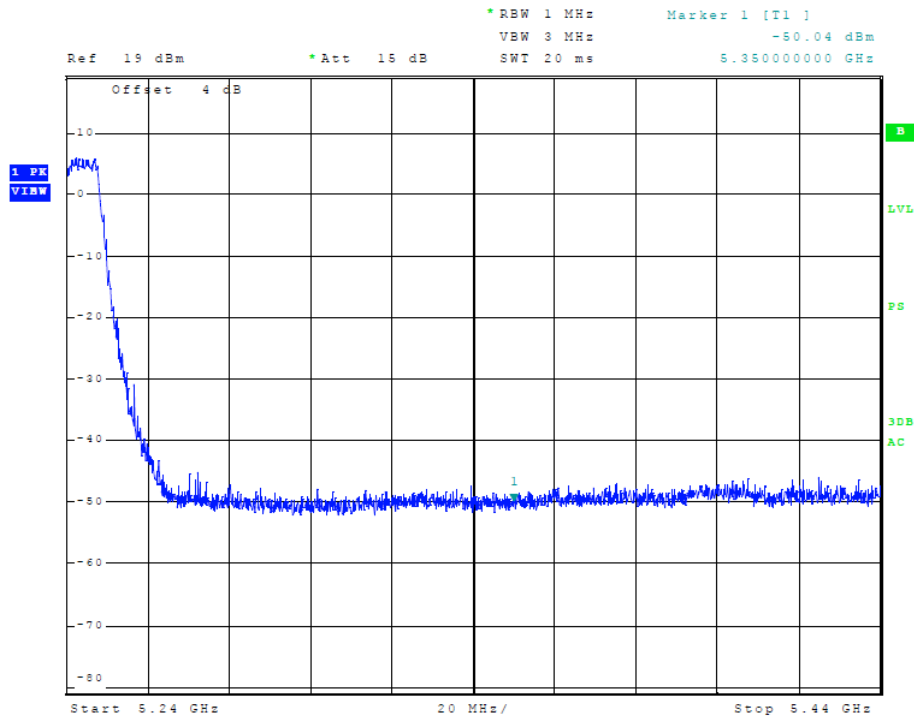
Figure 63 Plot of Transmitter High Band Edge (5150-5250 MHz Band, 20 MHz Chnl, Chain 2)
