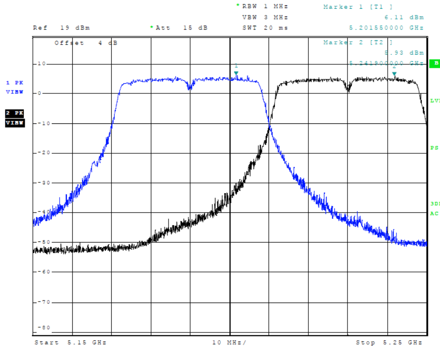
Figure 31 Plot of Transmitter Emissions (Across 5150-5250 MHz Band, 40 MHz Chnl, Chain 1)
