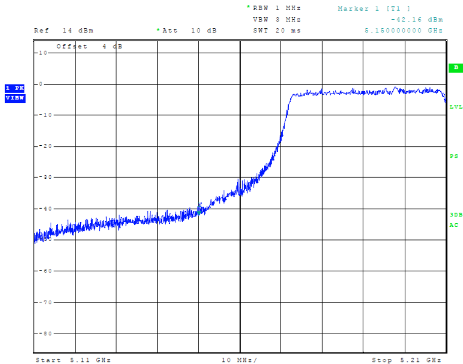
Figure 62 Plot of Transmitter Low Band Edge (5150-5250 MHz Band, 80 MHz Chnl, Chain 2)
