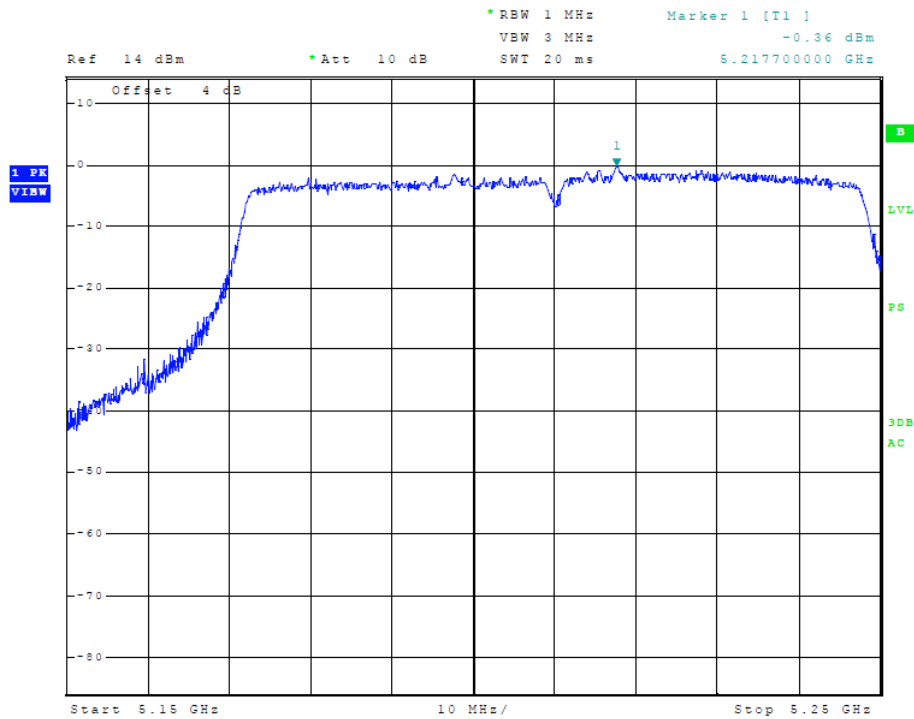
Figure 59 Plot of Transmitter Emissions (Across 5150-5250 MHz Band, 80 MHz Chnl, Chain 2)
