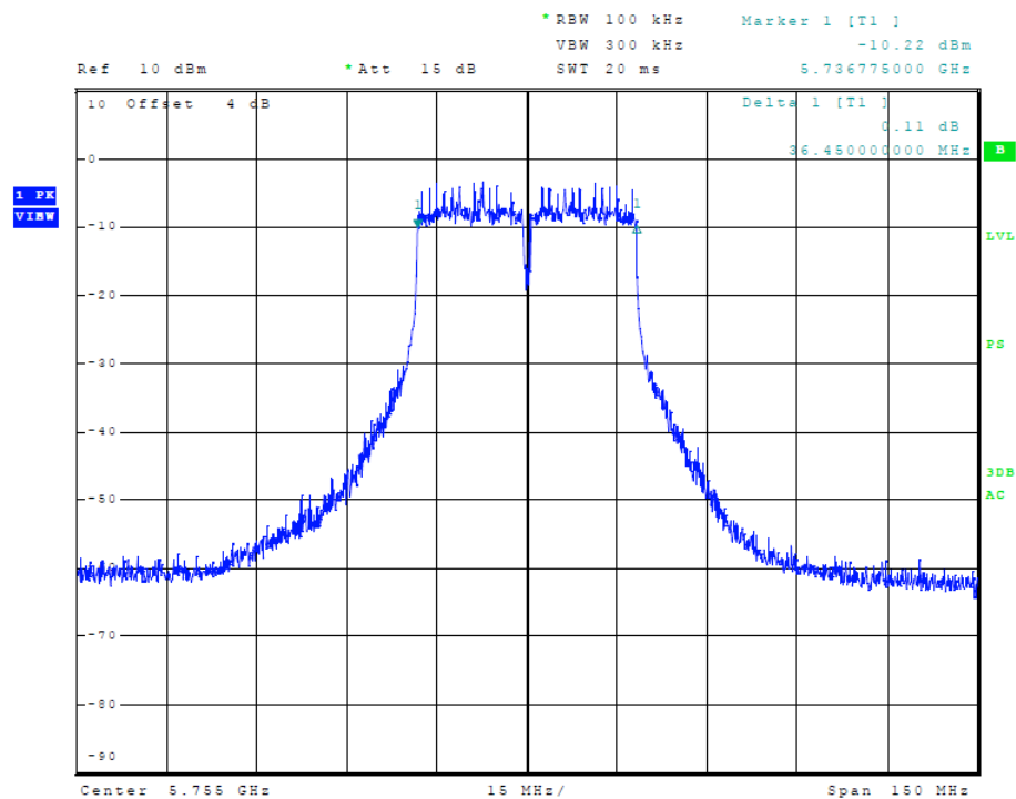
Figure 54 Plot of Transmitter Emissions (5725-5850 MHz Band, 40 MHz Chnl, Chain 1, 6-dB OBW)
