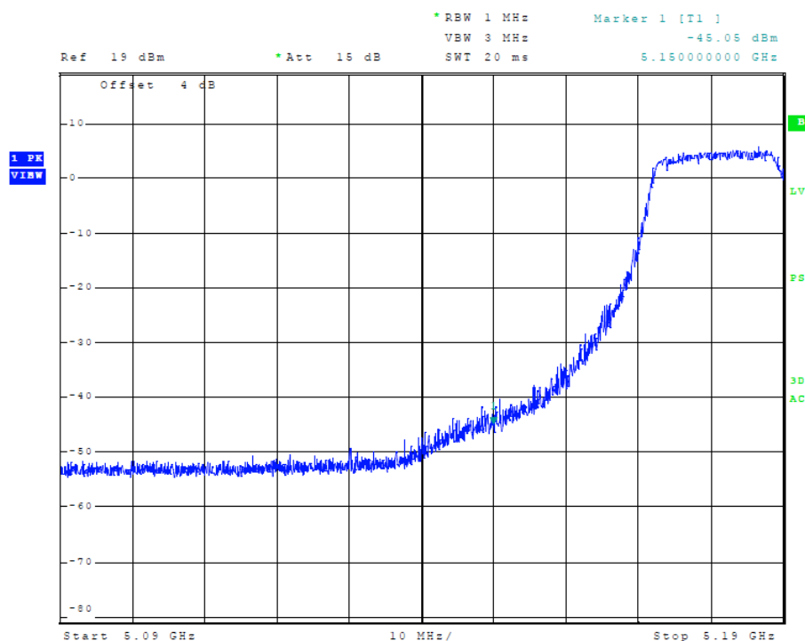
Figure 34 Plot of Transmitter Low Band Edge (5150-5250 MHz Band, 40 MHz Chnl, Chain 1)
