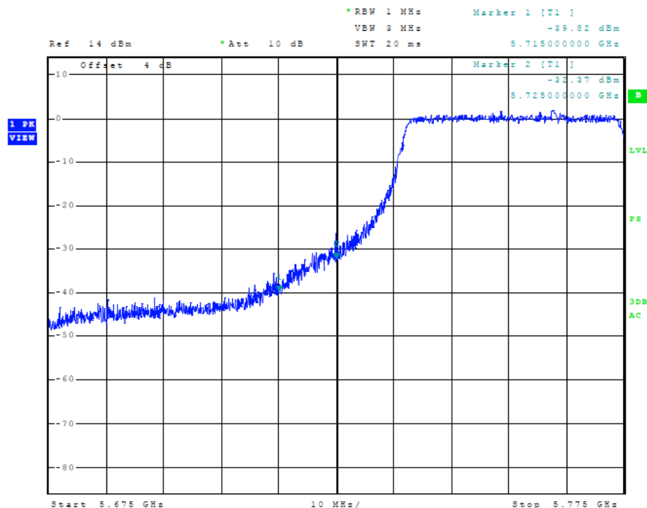
Figure 74 Plot of Transmitter Low Band Edge (5725-5850 MHz Band, 80 MHz Chnl, Chain 2)
