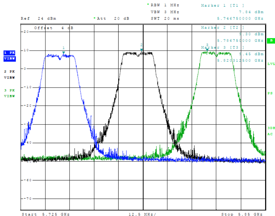
Figure 69 Plot of Transmitter Emissions (Across 5725-5850 MHz Band, 20 MHz Chnl, Chain 2)
