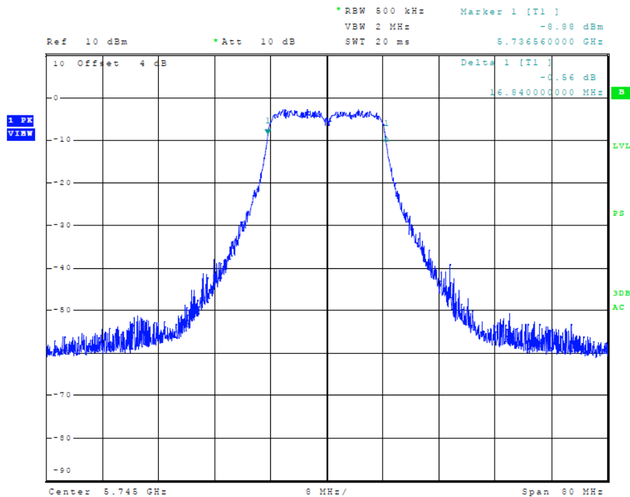
Figure 52 Plot of Transmitter Emissions (5725-5850 MHz Band, 20 MHz Chnl, Chain 1, 6-dB OBW)
