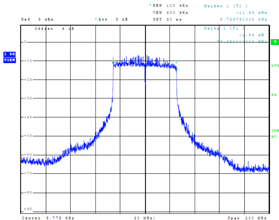
Figure 84 Plot of Transmitter Emissions (5725-5850 MHz Band, 80 MHz Chnl, Chain 2, 6-dB OBW)
