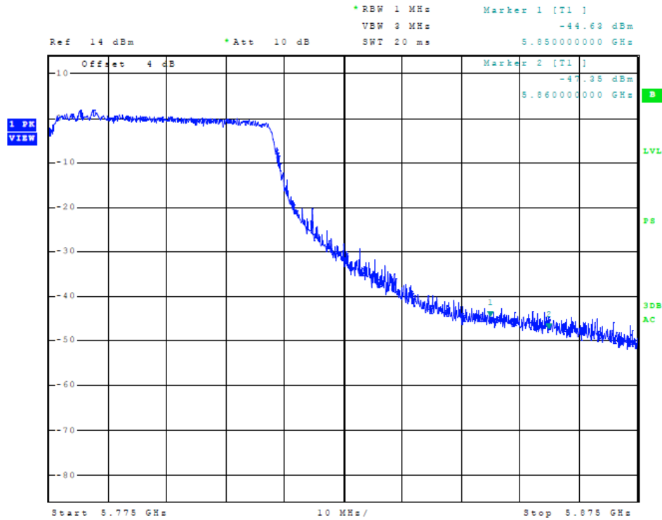
Figure 78 Plot of Transmitter High Band Edge (5725-5850 MHz Band, 80 MHz Chnl, Chain 2)
