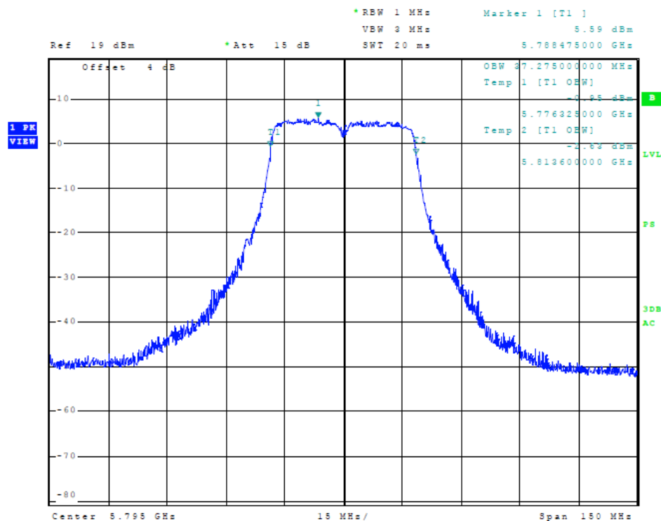
Figure 81 Plot of Transmitter Emissions (5725-5850 MHz Band, 40 MHz Chnl, Chain 2, 99% OBW)
