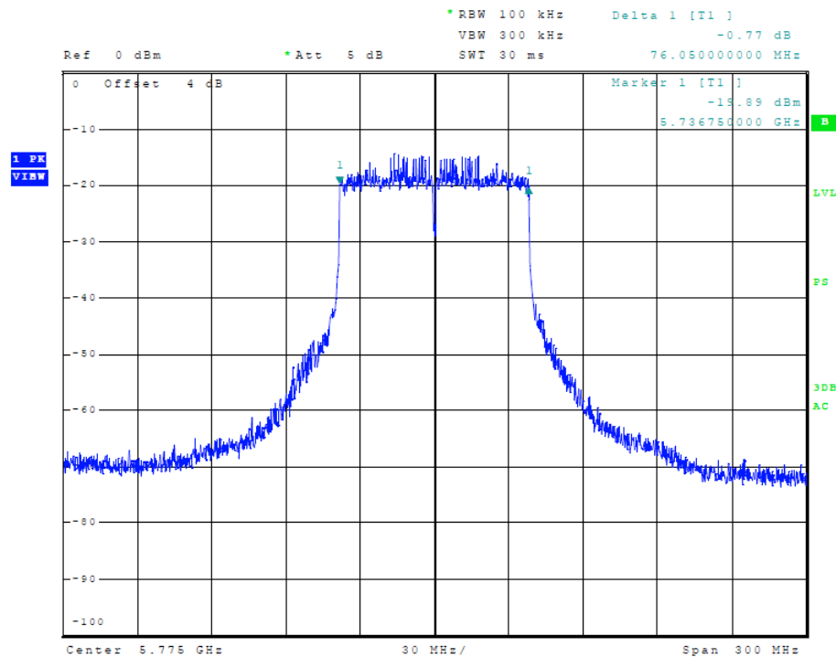
Figure 56 Plot of Transmitter Emissions (5725-5850 MHz Band, 80 MHz Chnl, Chain 1, 6-dB OBW)
