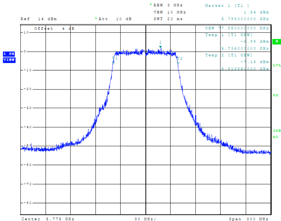
Figure 28 Plot of Transmitter Emissions (5725-5850 MHz Band, 80 MHz Chnl, Chain 0, 99% OBW)
