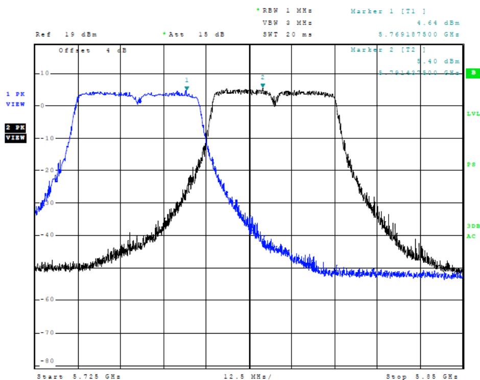
Figure 70 Plot of Transmitter Emissions (Across 5725-5850 MHz Band, 40 MHz Chnl, Chain 2)
