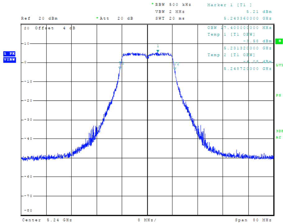
Figure 39 Plot of Transmitter Emissions (5150-5250 MHz Band, 20 MHz Chnl, Chain 1, 99% OBW)
