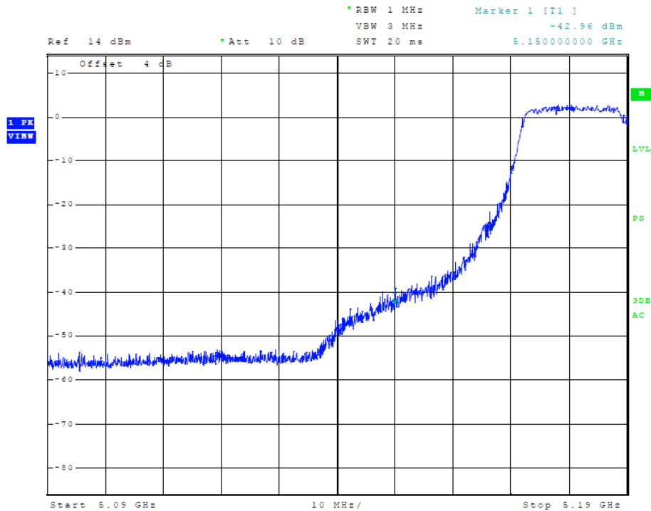
Figure 61 Plot of Transmitter Low Band Edge (5150-5250 MHz Band, 40 MHz Chnl, Chain 2)
