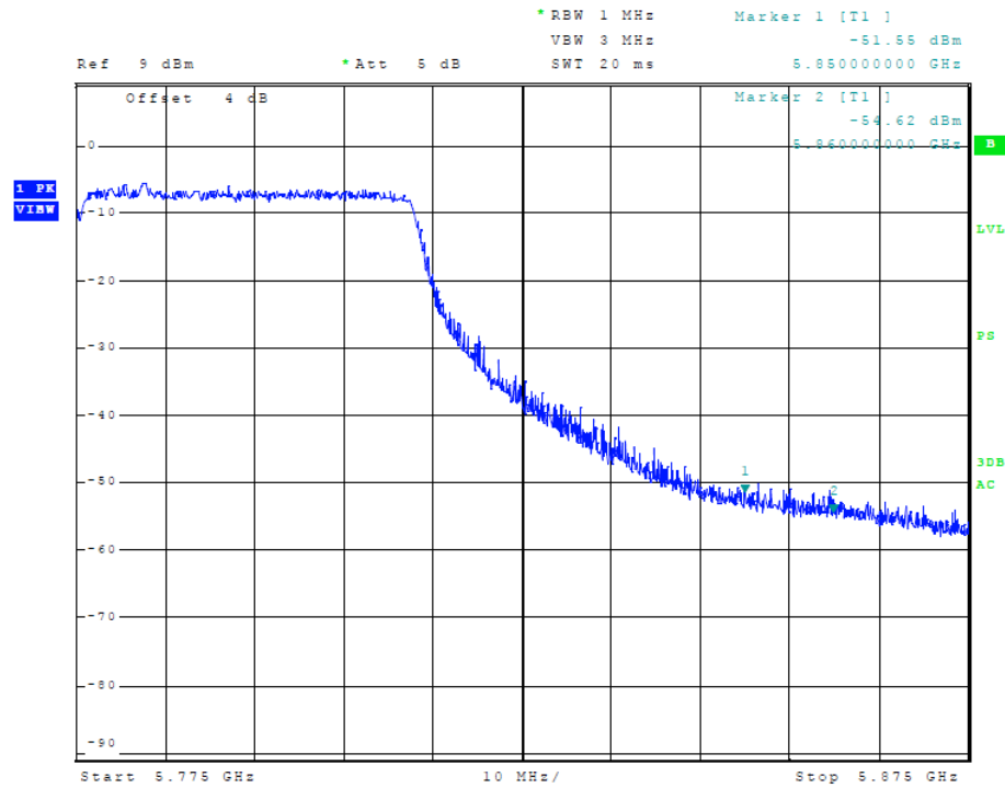
Figure 23 Plot of Transmitter High Band Edge (5725-5850 MHz Band, 80 MHz Chnl, Chain 0)
