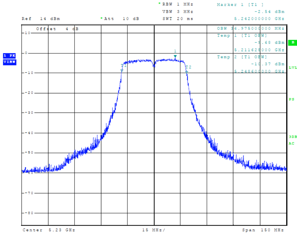
Figure 13 Plot of Transmitter Emissions (5150-5250 MHz Band, 40 MHz Chnl, Chain 0, 99% OBW)
