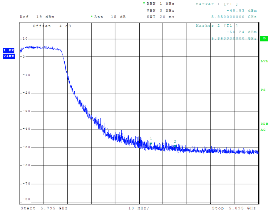
Figure 49 Plot of Transmitter High Band Edge (5725-5850 MHz Band, 40 MHz Chnl, Chain 1)
