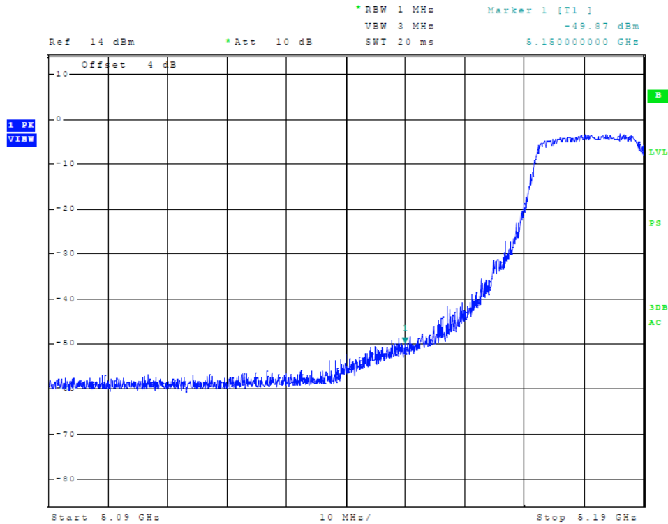
Figure 7 Plot of Transmitter Low Band Edge (5150-5250 MHz Band, 40 MHz Chnl, Chain 0)
