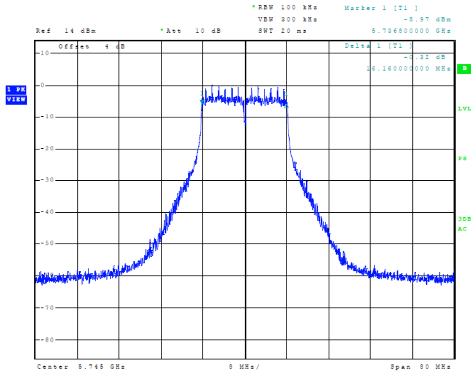
Figure 80 Plot of Transmitter Emissions (5725-5850 MHz Band, 20 MHz Chnl, Chain 2, 6-dB OBW)
