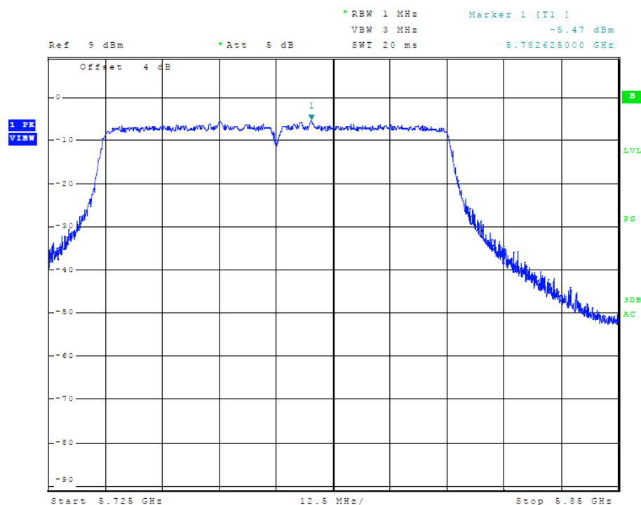
Figure 44 Plot of Transmitter Emissions (Across 5725-5850 MHz Band, 80 MHz Chnl, Chain 1)
