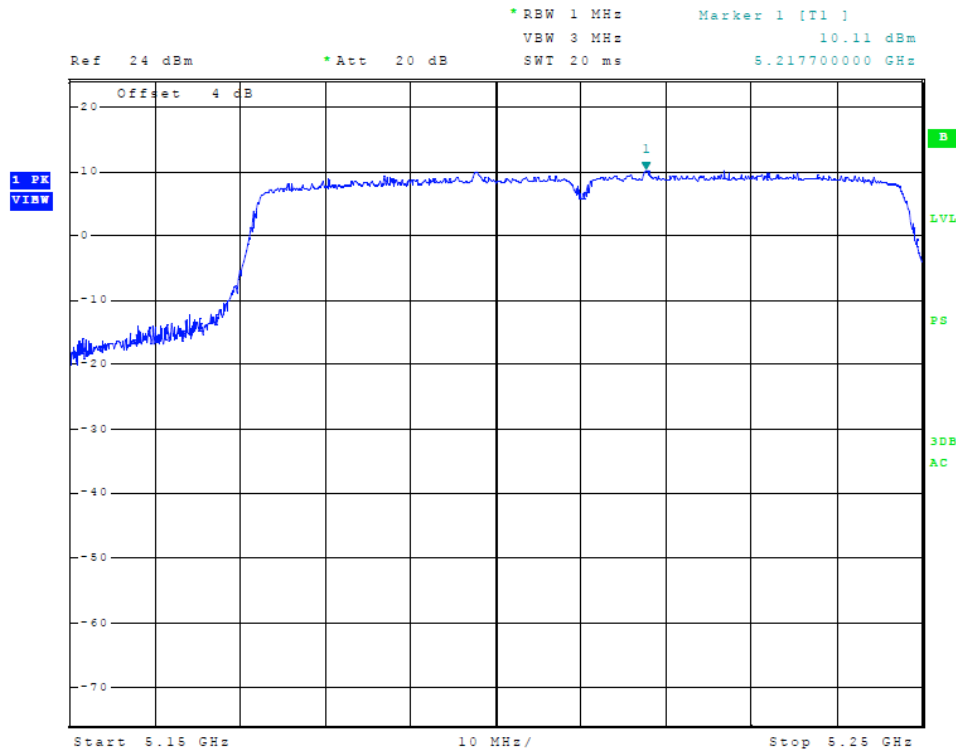
Figure 5 Plot of Transmitter Emissions (Across 5150-5250 MHz Band, 80 MHz Chnl, Chain 0)
