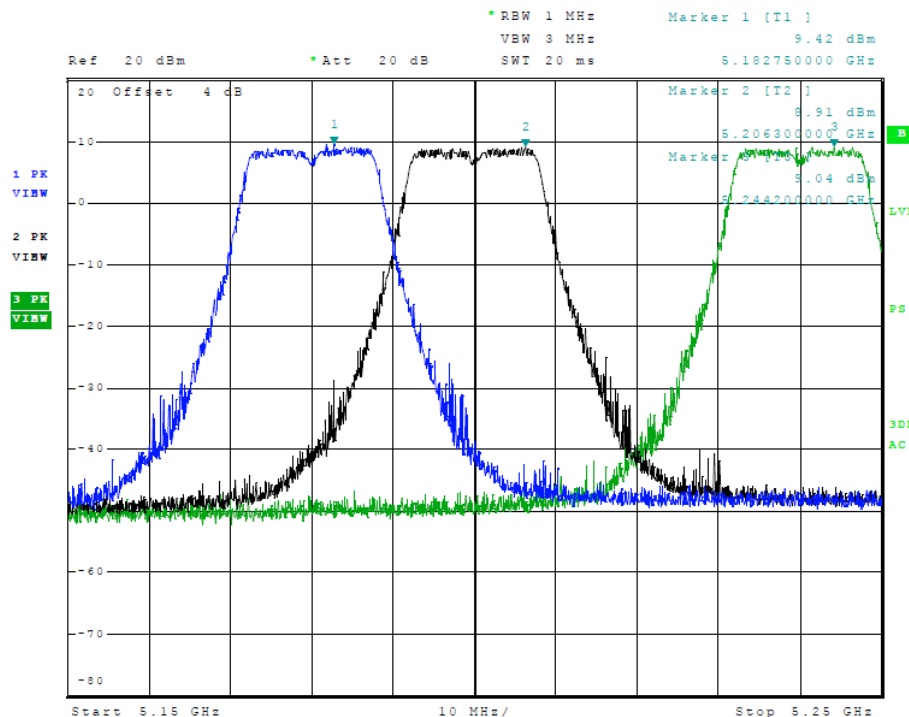
Figure 30 Plot of Transmitter Emissions (Across 5150-5250 MHz Band, 20 MHz Chnl, Chain 1)
