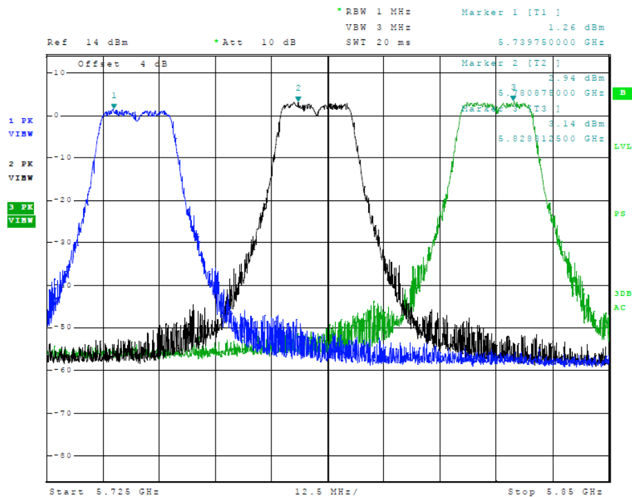
Figure 15 Plot of Transmitter Emissions (Across 5725-5850 MHz Band, 20 MHz Chnl, Chain 0)
