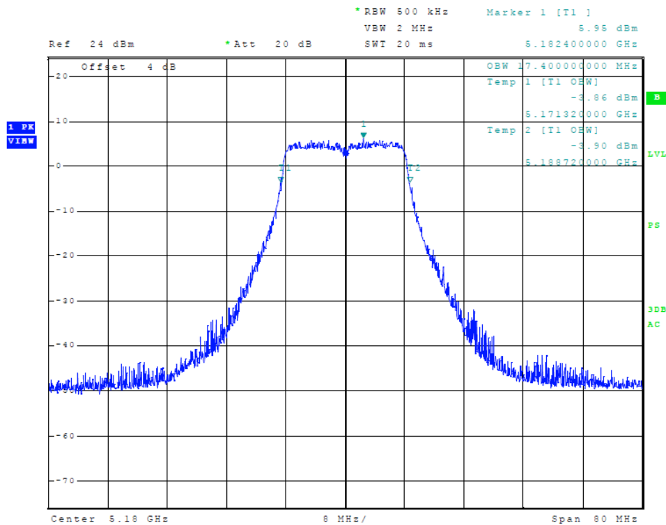
Figure 12 Plot of Transmitter Emissions (5150-5250 MHz Band, 20 MHz Chnl, Chain 0, 99% OBW)
