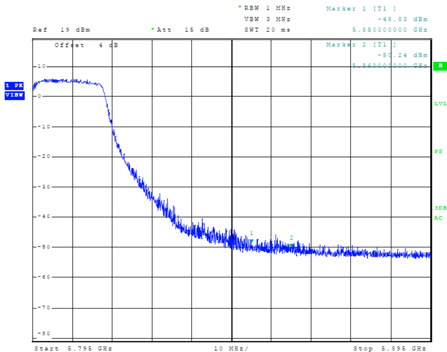
Figure 22 Plot of Transmitter High Band Edge (5725-5850 MHz Band, 40 MHz Chnl, Chain 0)
