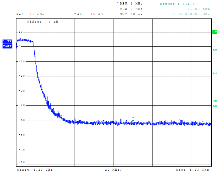
Figure 37 Plot of Transmitter High Band Edge (5150-5250 MHz Band, 40 MHz Chnl, Chain 1)
