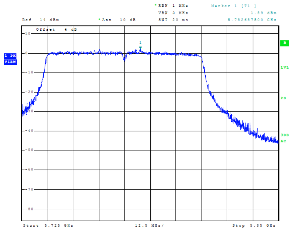
Figure 71 Plot of Transmitter Emissions (Across 5725-5850 MHz Band, 80 MHz Chnl, Chain 2)
