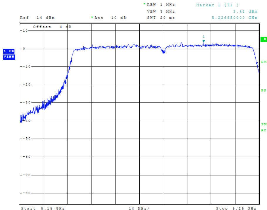
Figure 32 Plot of Transmitter Emissions (Across 5150-5250 MHz Band, 80 MHz Chnl, Chain 1)
