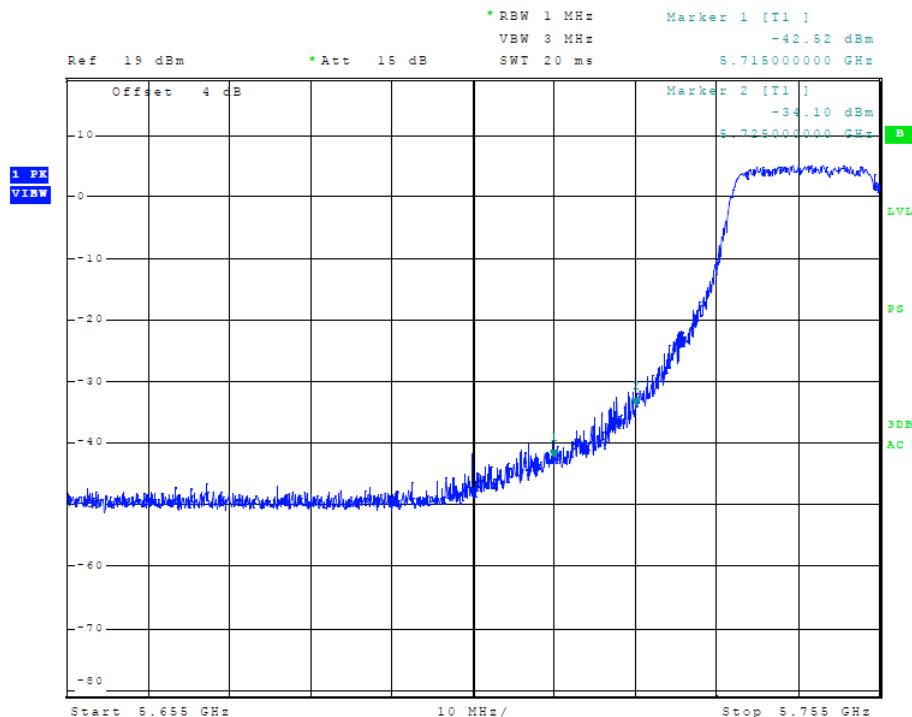
Figure 46 Plot of Transmitter Low Band Edge (5725-5850 MHz Band, 40 MHz Chnl, Chain 1)
