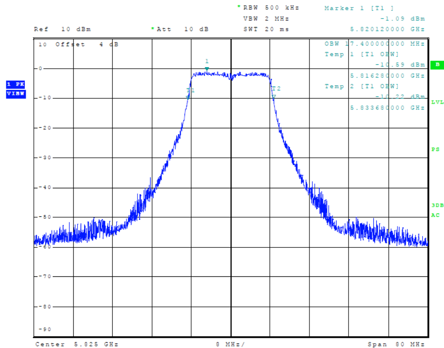
Figure 24 Plot of Transmitter Emissions (5725-5850 MHz Band, 20 MHz Chnl, Chain 0, 99% OBW)
