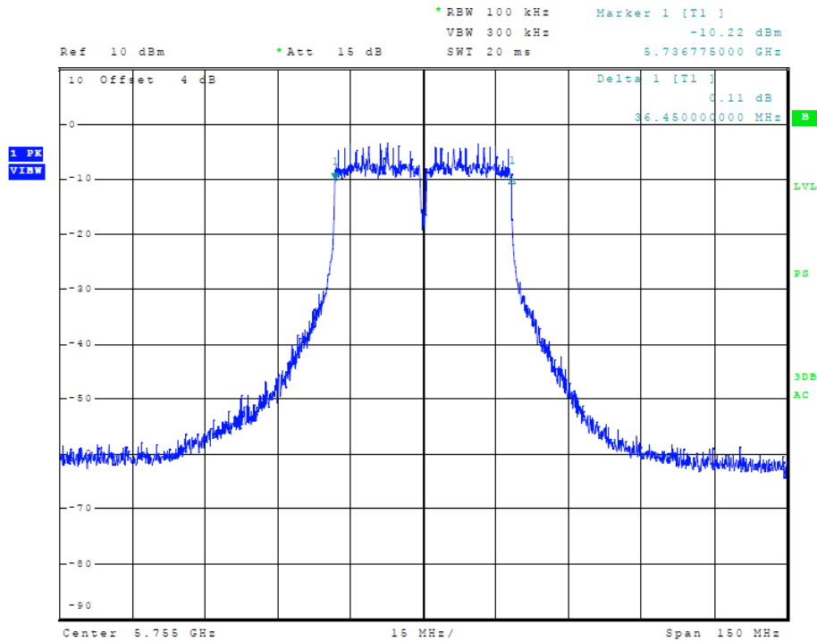
Figure 27 Plot of Transmitter Emissions (5725-5850 MHz Band, 40 MHz Chnl, Chain 0, 6-dB OBW)
