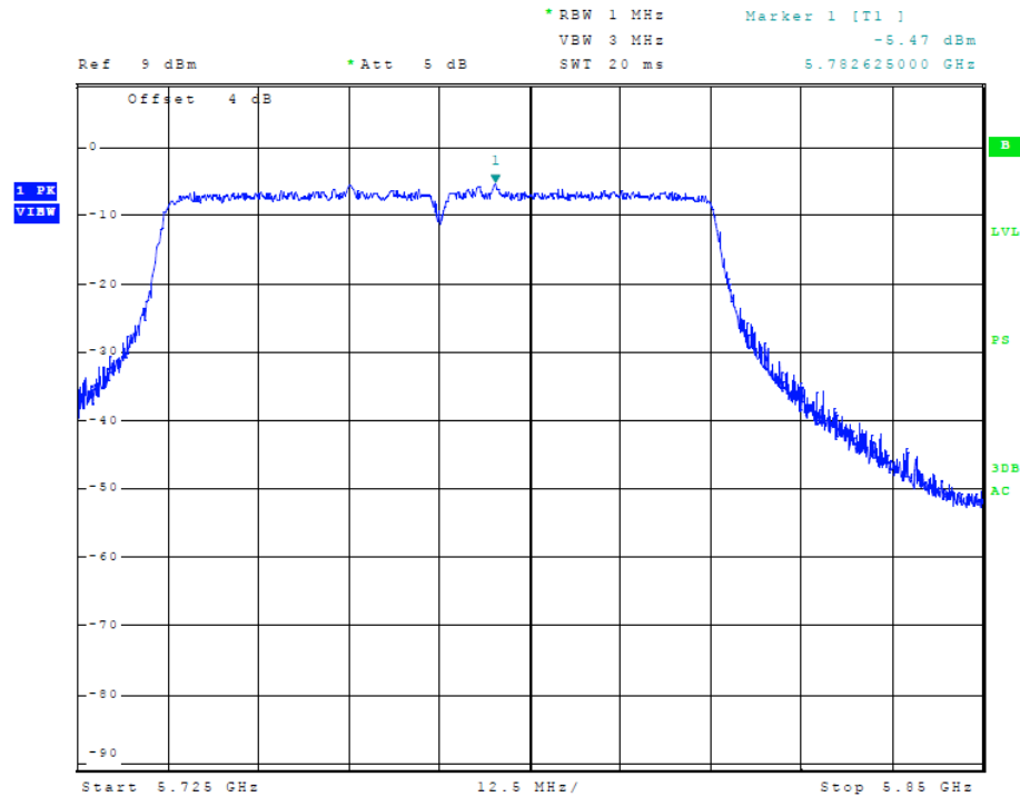
Figure 17 Plot of Transmitter Emissions (Across 5725-5850 MHz Band, 80 MHz Chnl, Chain 0)
