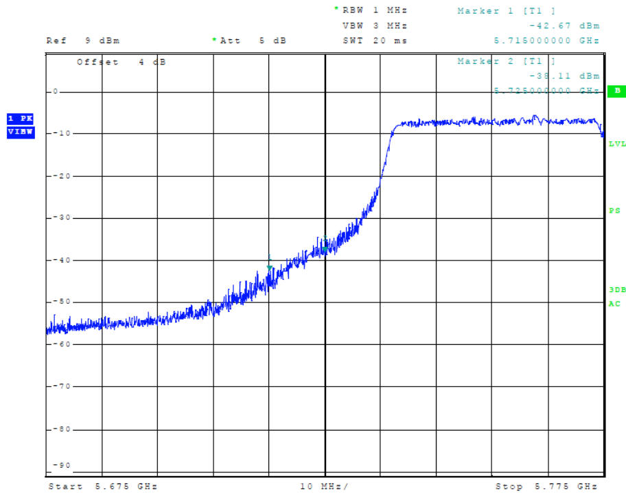
Figure 47 Plot of Transmitter Low Band Edge (5725-5850 MHz Band, 80 MHz Chnl, Chain 1)
