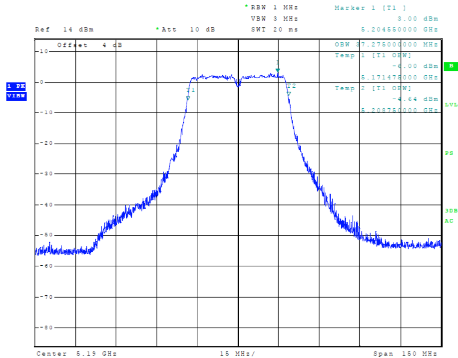
Figure 67 Plot of Transmitter Emissions (5150-5250 MHz Band, 40 MHz Chnl, Chain 2, 99% OBW)
