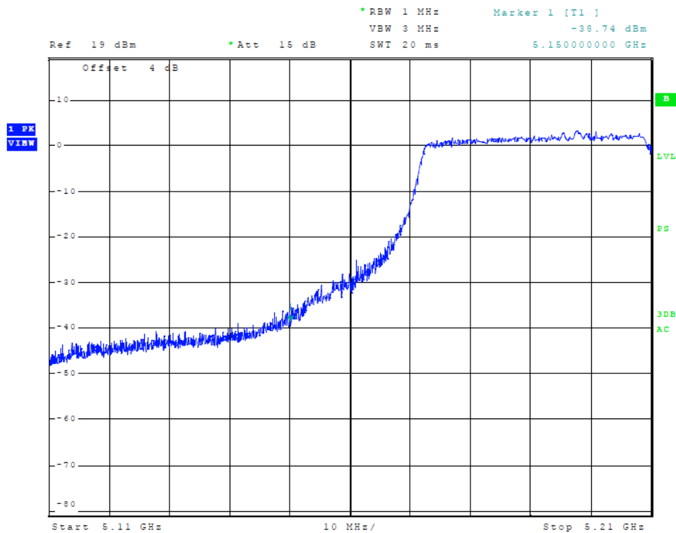
Figure 8 Plot of Transmitter Low Band Edge (5150-5250 MHz Band, 80 MHz Chnl, Chain 0)
