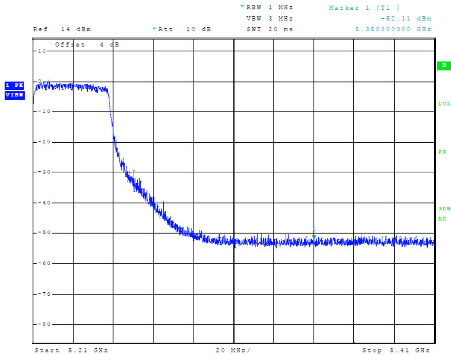
Figure 65 Plot of Transmitter High Band Edge (5150-5250 MHz Band, 80 MHz Chnl, Chain 2)
