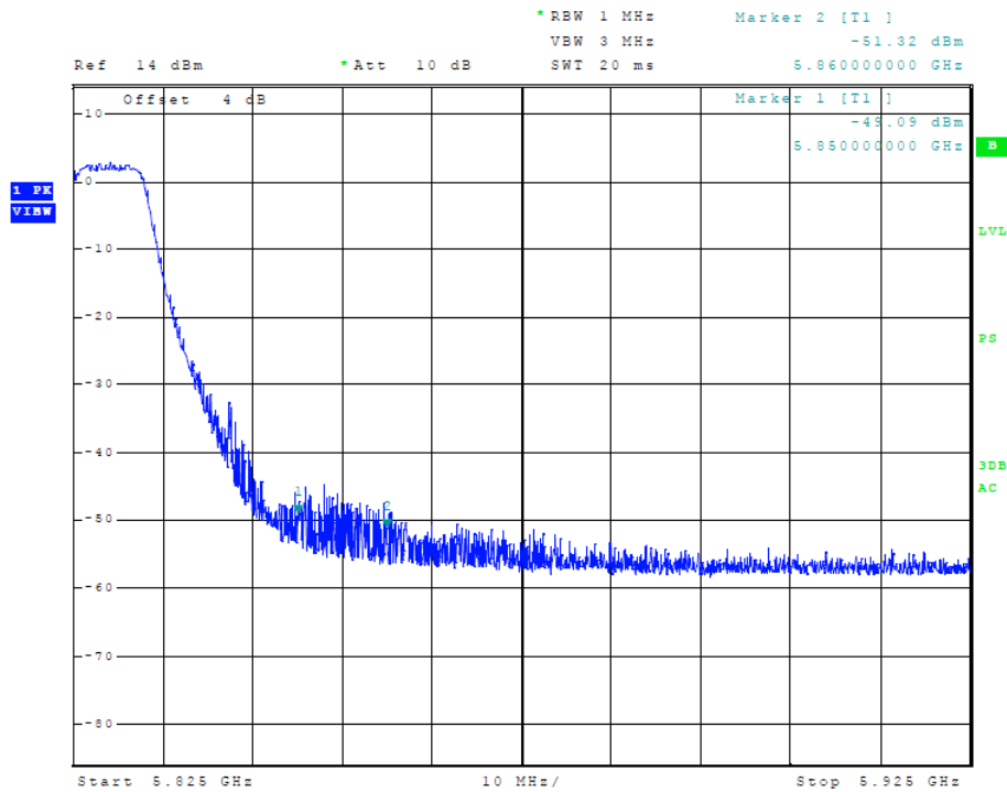
Figure 21 Plot of Transmitter High Band Edge (5725-5850 MHz Band, 20 MHz Chnl, Chain 0)
