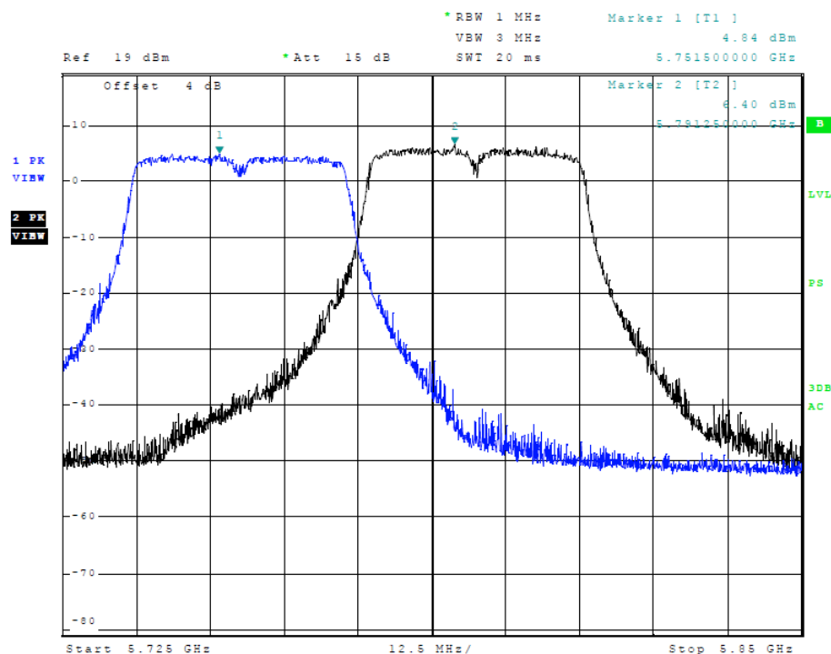
Figure 43 Plot of Transmitter Emissions (Across 5725-5850 MHz Band, 40 MHz Chnl, Chain 1)
