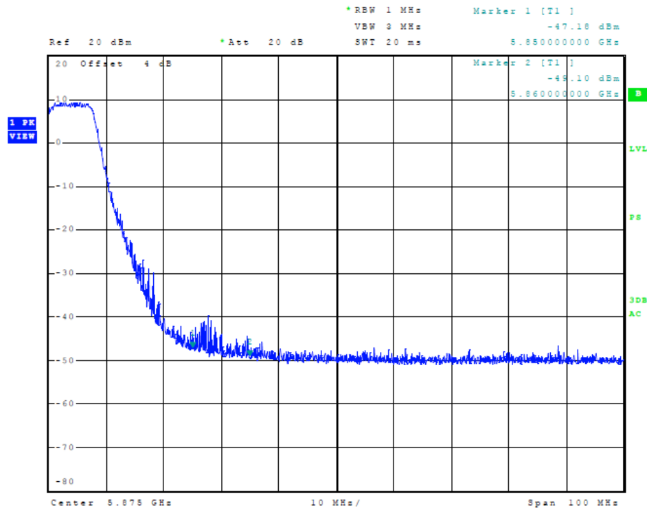
Figure 75 Plot of Transmitter High Band Edge (5725-5850 MHz Band, 20 MHz Chnl, Chain 2)
