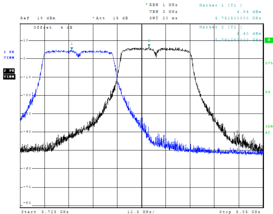
Figure 16 Plot of Transmitter Emissions (Across 5725-5850 MHz Band, 40 MHz Chnl, Chain 0)
