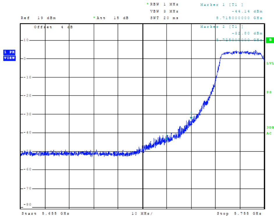
Figure 73 Plot of Transmitter Low Band Edge (5725-5850 MHz Band, 40 MHz Chnl, Chain 2)
