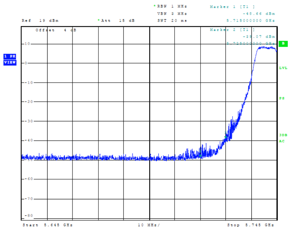
Figure 72 Plot of Transmitter Low Band Edge (5725-5850 MHz Band, 20 MHz Chnl, Chain 2)
