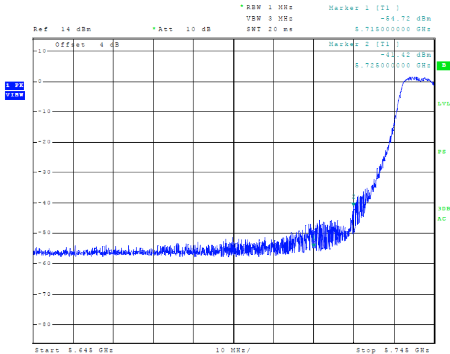
Figure 45 Plot of Transmitter Low Band Edge (5725-5850 MHz Band, 20 MHz Chnl, Chain 1)
