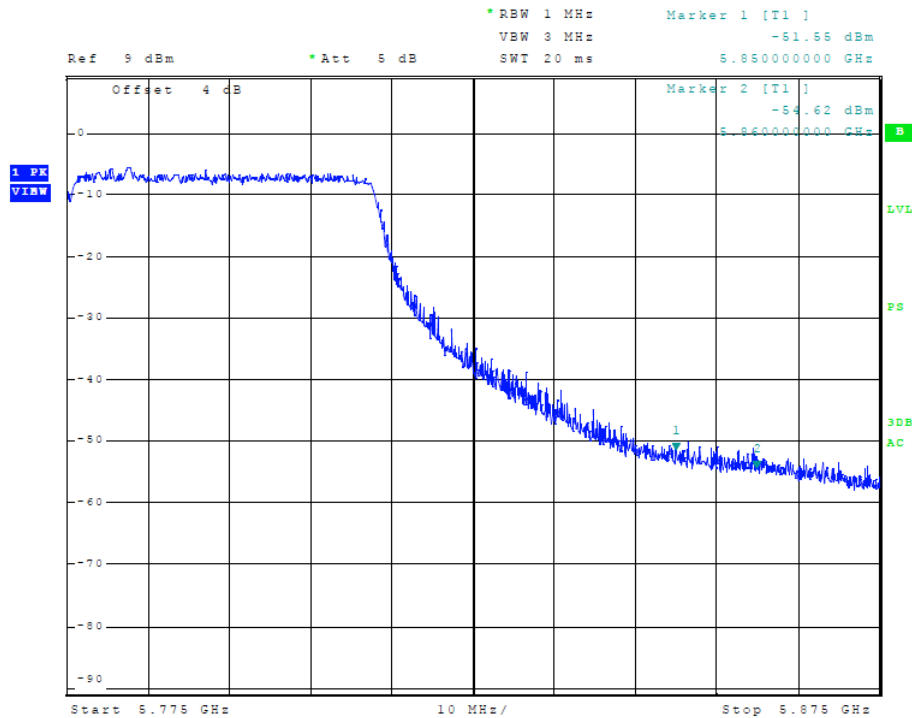
Figure 50 Plot of Transmitter High Band Edge (5725-5850 MHz Band, 80 MHz Chnl, Chain 1)
