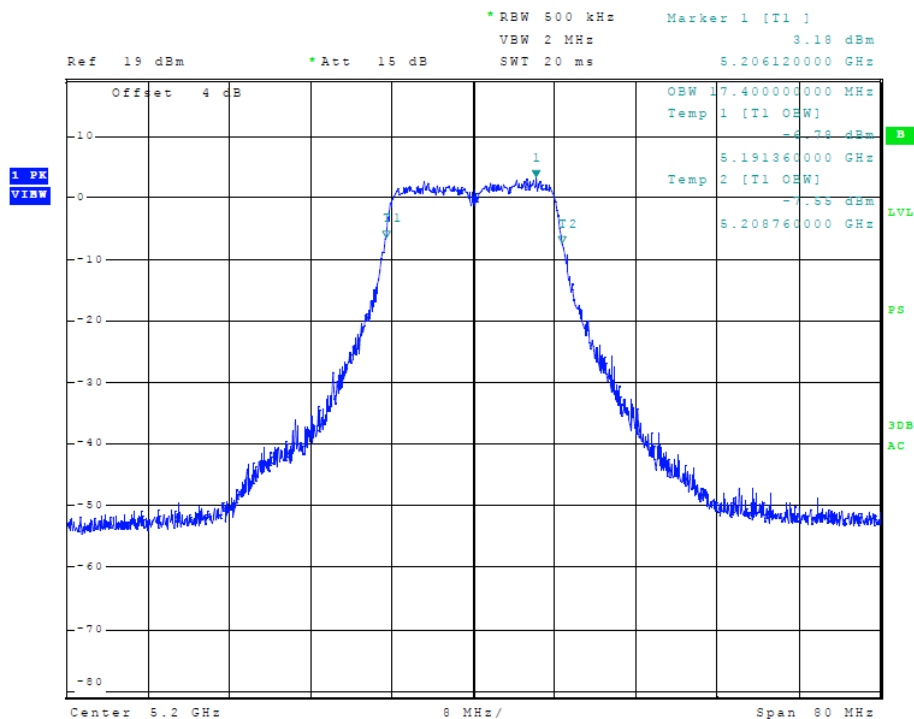
Figure 66 Plot of Transmitter Emissions (5150-5250 MHz Band, 20 MHz Chnl, Chain 2, 99% OBW)
