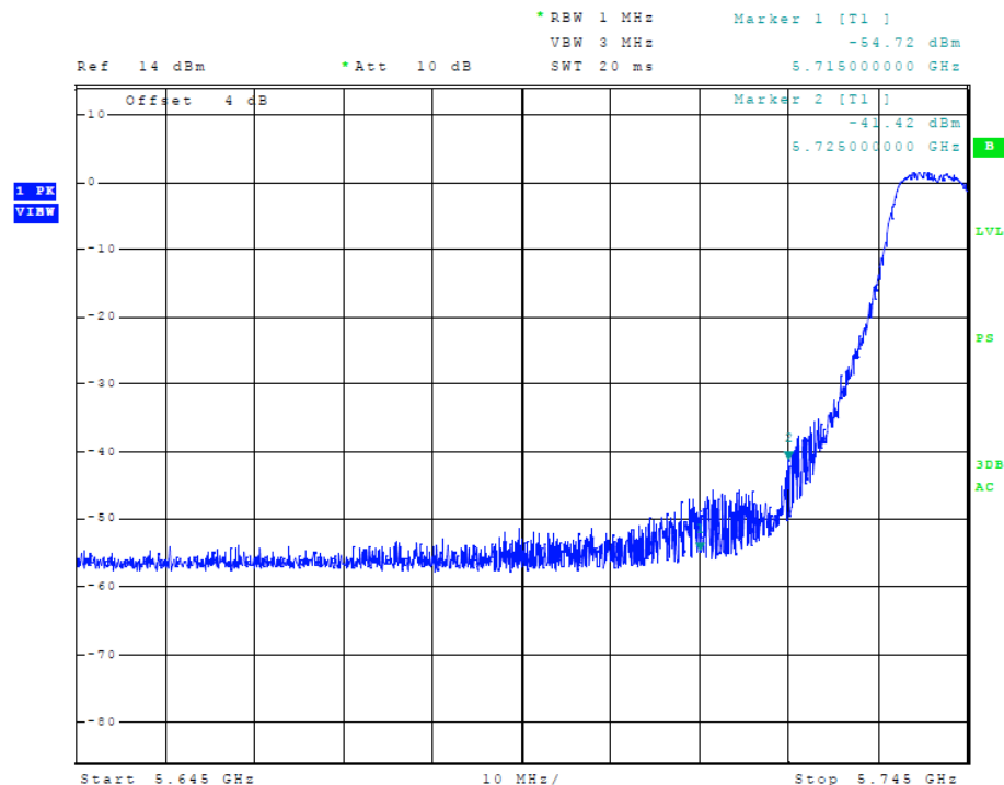
Figure 18 Plot of Transmitter Low Band Edge (5725-5850 MHz Band, 20 MHz Chnl, Chain 0)
