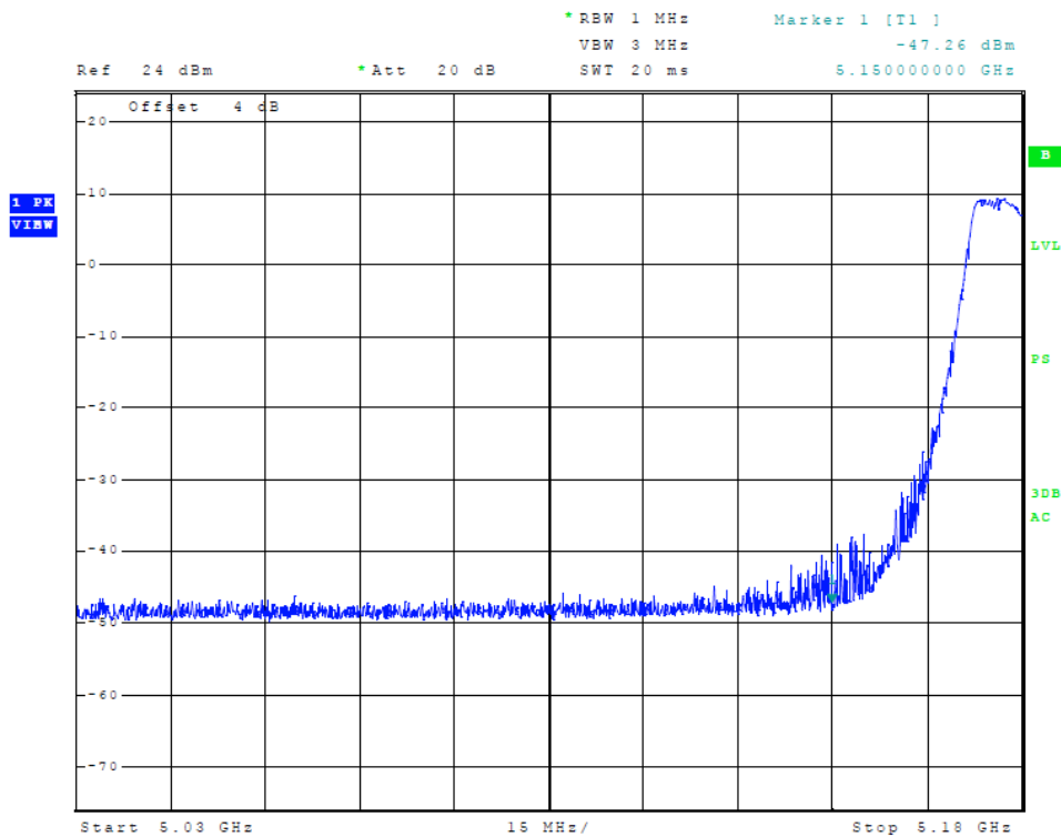
Figure 6 Plot of Transmitter Low Band Edge (5150-5250 MHz Band, 20 MHz Chnl, Chain 0)
