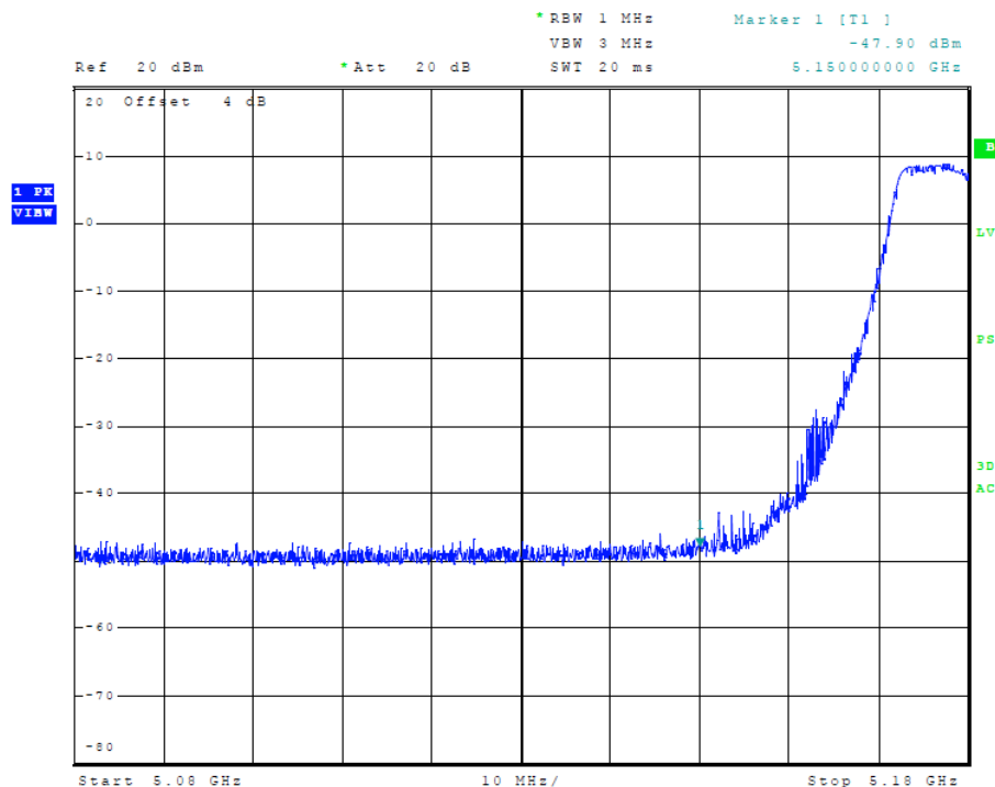
Figure 33 Plot of Transmitter Low Band Edge (5150-5250 MHz Band, 20 MHz Chnl, Chain 1)
