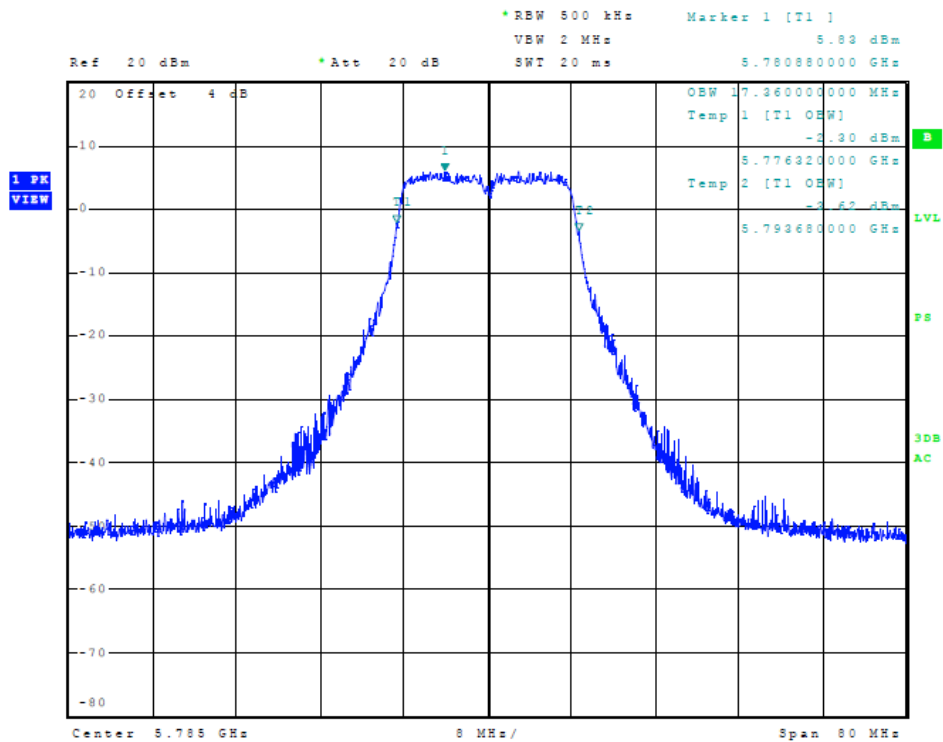
Figure 79 Plot of Transmitter Emissions (5725-5850 MHz Band, 20 MHz Chnl, Chain 2, 99% OBW)
