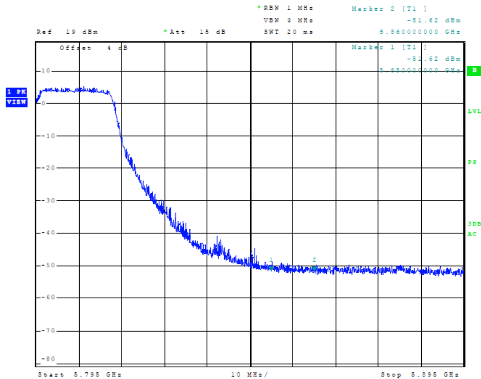
Figure 76 Plot of Transmitter High Band Edge (5725-5850 MHz Band, 40 MHz Chnl, Chain 2)
