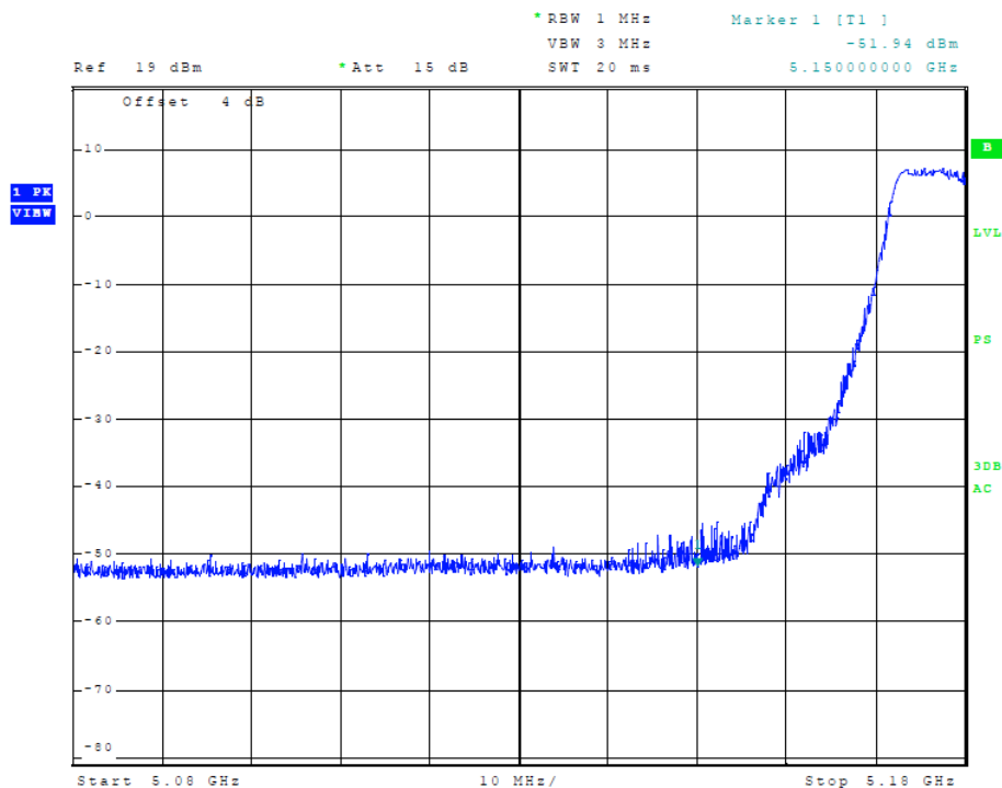
Figure 60 Plot of Transmitter Low Band Edge (5150-5250 MHz Band, 20 MHz Chnl, Chain 2)
