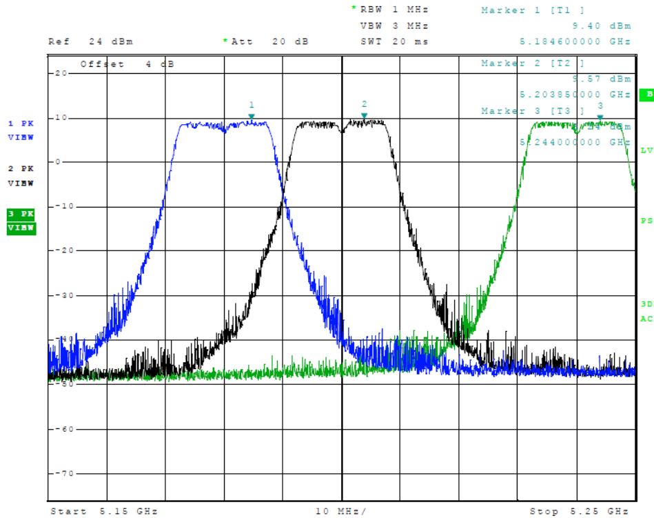
Figure 3 Plot of Transmitter Emissions (Across 5150-5250 MHz Band, 20 MHz Chnl, Chain 0)
