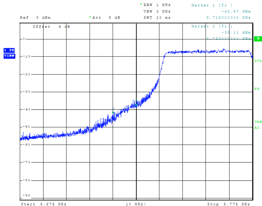
Figure 20 Plot of Transmitter Low Band Edge (5725-5850 MHz Band, 80 MHz Chnl, Chain 0)
