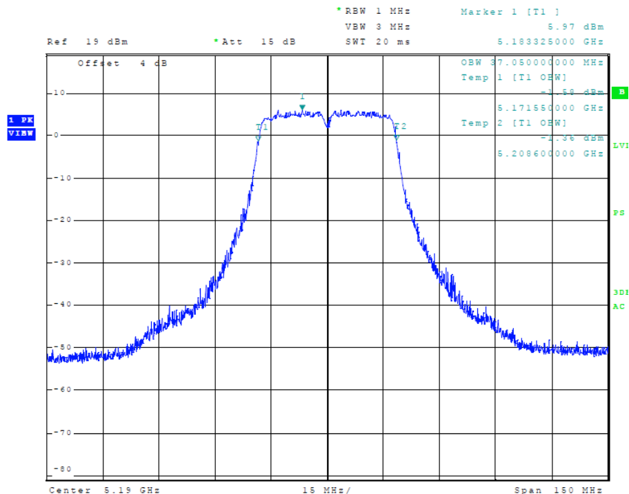
Figure 40 Plot of Transmitter Emissions (5150-5250 MHz Band, 40 MHz Chnl, Chain 1, 99% OBW)
