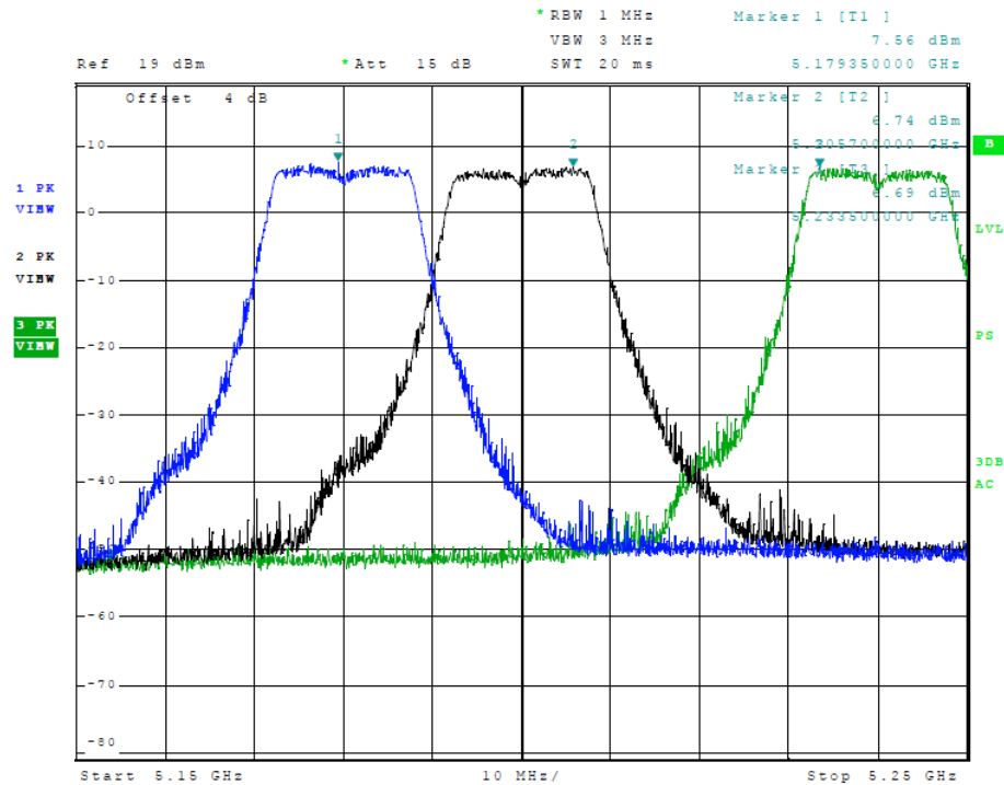
Figure 57 Plot of Transmitter Emissions (Across 5150-5250 MHz Band, 20 MHz Chnl, Chain 2)
