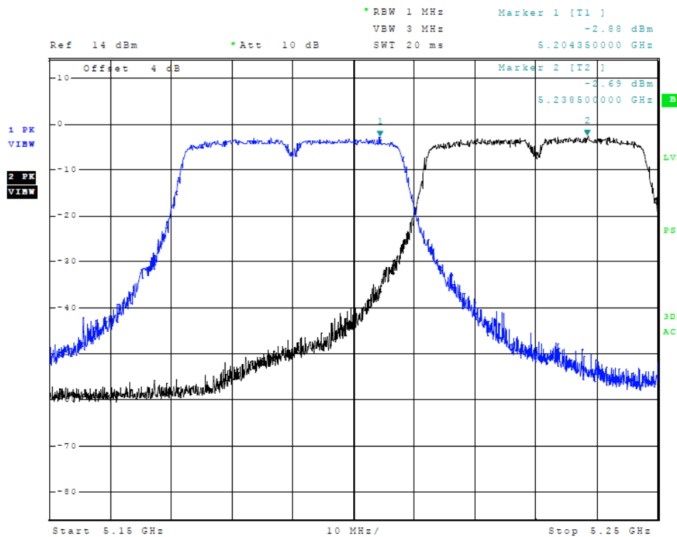
Figure 4 Plot of Transmitter Emissions (Across 5150-5250 MHz Band, 40 MHz Chnl, Chain 0)
