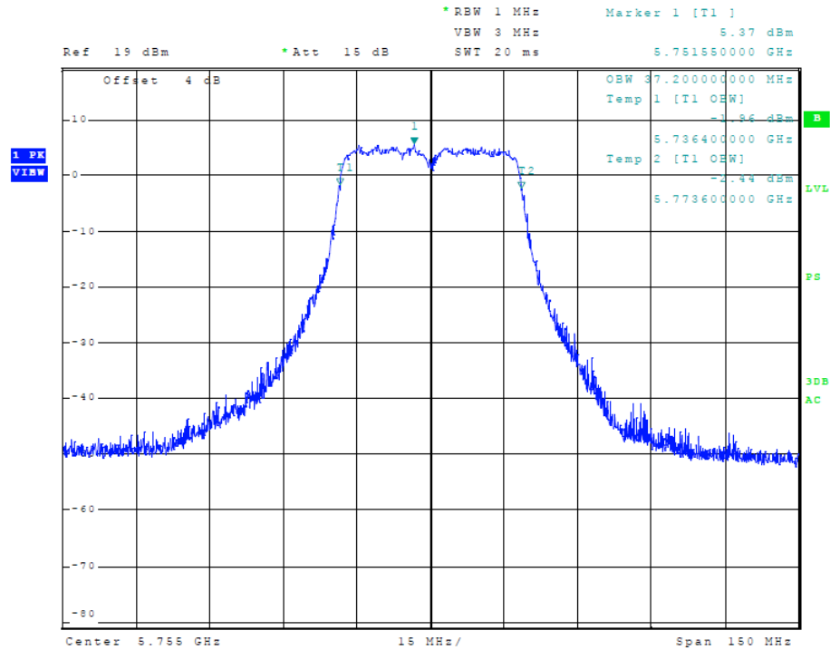
Figure 53 Plot of Transmitter Emissions (5725-5850 MHz Band, 40 MHz Chnl, Chain 1, 99% OBW)
