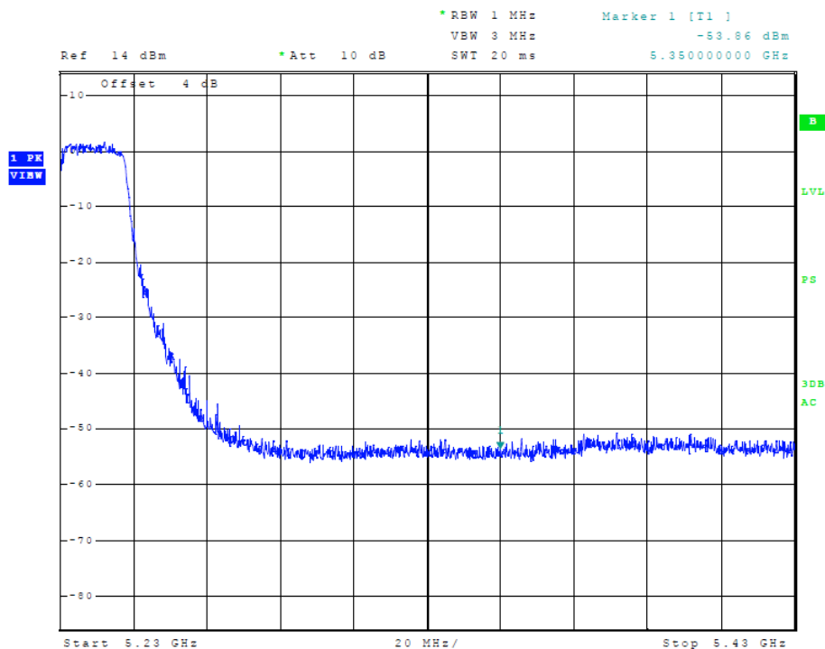
Figure 64 Plot of Transmitter High Band Edge (5150-5250 MHz Band, 40 MHz Chnl, Chain 2)
