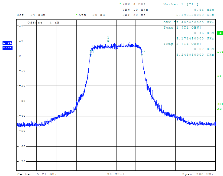
Figure 41 Plot of Transmitter Emissions (5150-5250 MHz Band, 80 MHz Chnl, Chain 1, 99% OBW)
