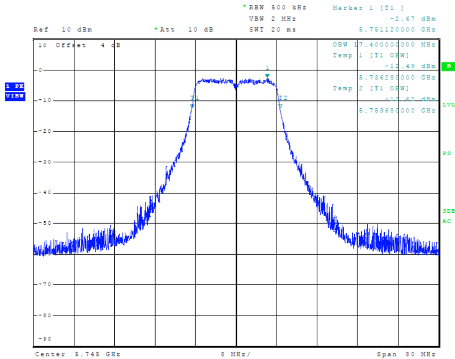
Figure 51 Plot of Transmitter Emissions (5725-5850 MHz Band, 20 MHz Chnl, Chain 1, 99% OBW)
