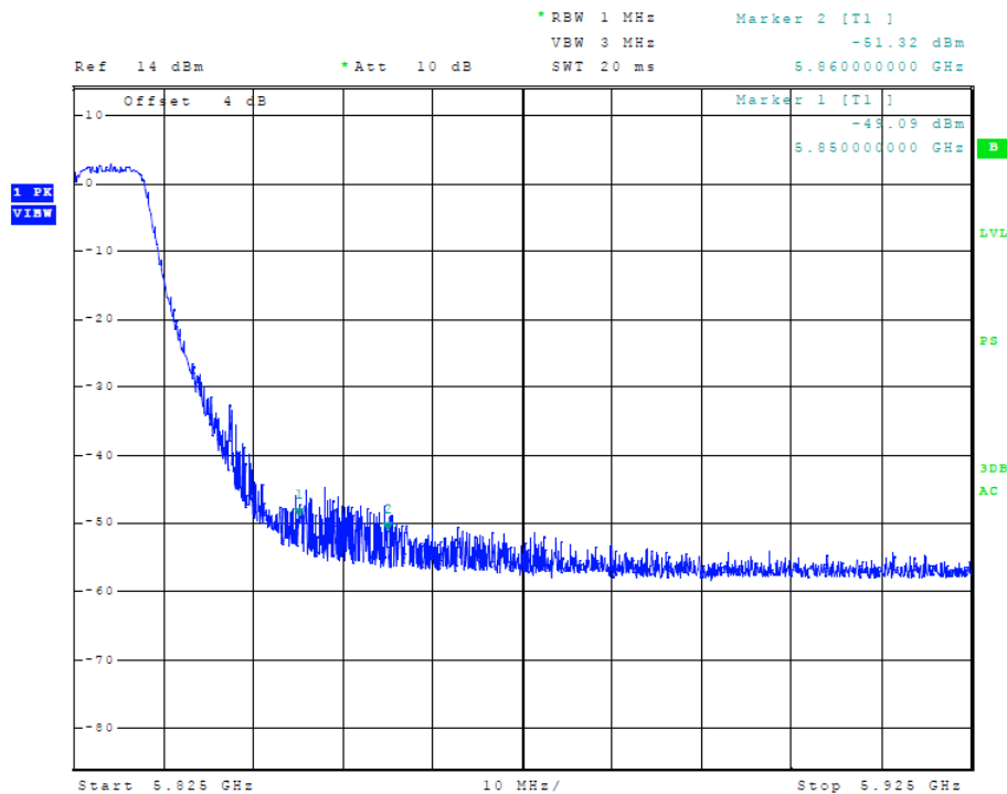
Figure 48 Plot of Transmitter High Band Edge (5725-5850 MHz Band, 20 MHz Chnl, Chain 1)
