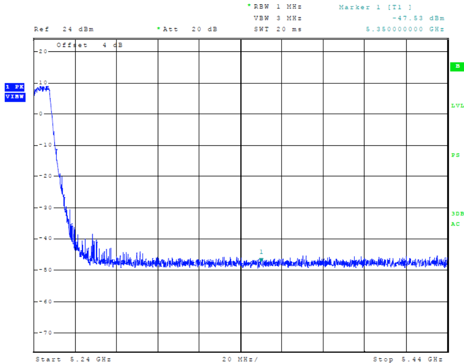
Figure 9 Plot of Transmitter High Band Edge (5150-5250 MHz Band, 20 MHz Chnl, Chain 0)
