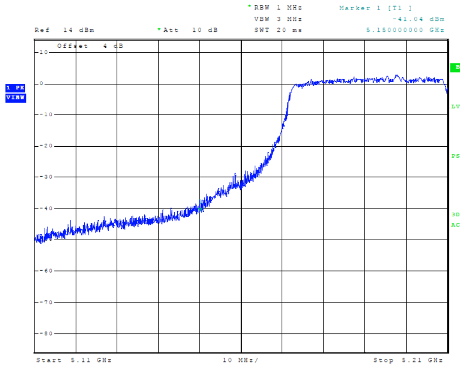
Figure 35 Plot of Transmitter Low Band Edge (5150-5250 MHz Band, 80 MHz Chnl, Chain 1)
