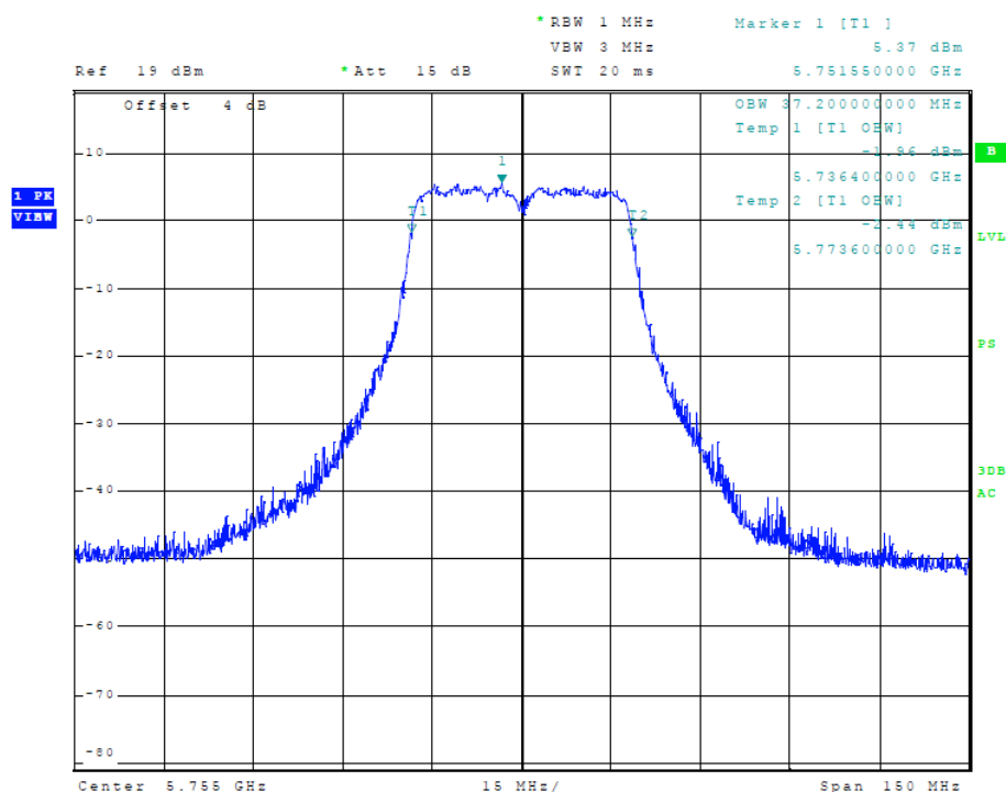
Figure 26 Plot of Transmitter Emissions (5725-5850 MHz Band, 40 MHz Chnl, Chain 0, 99% OBW)
