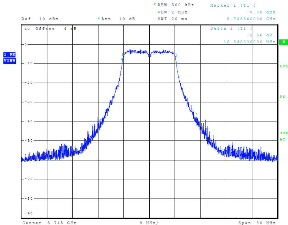
Figure 25 Plot of Transmitter Emissions (5725-5850 MHz Band, 20 MHz Chnl, Chain 0, 6-dB OBW)
