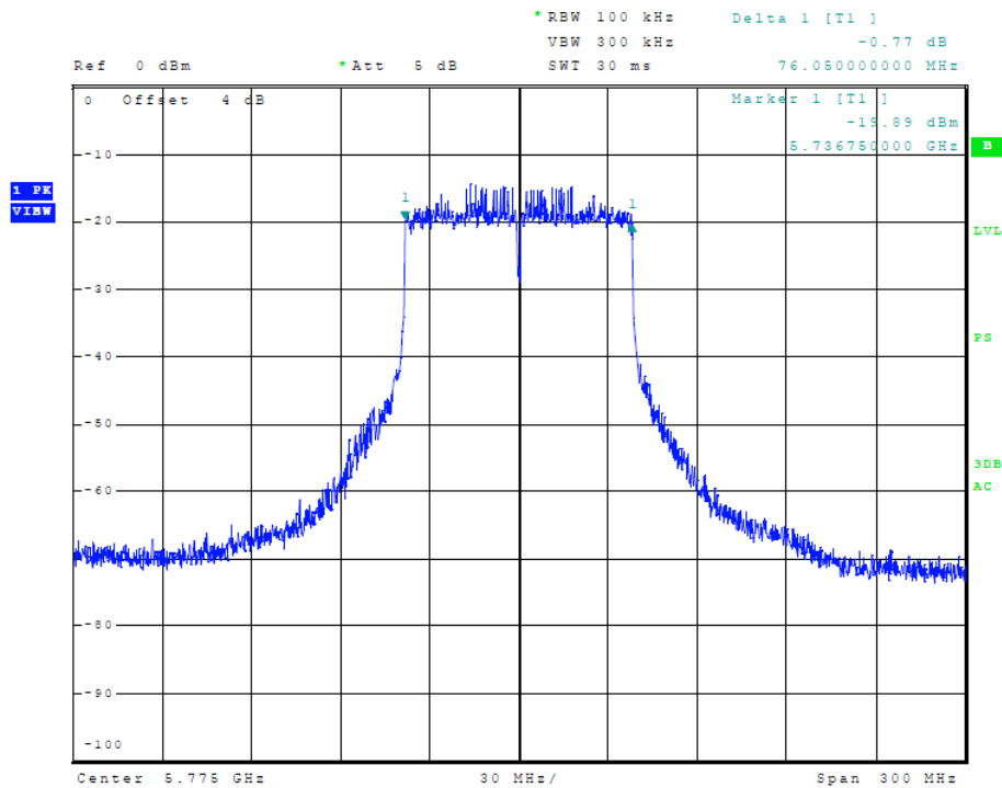
Figure 29 Plot of Transmitter Emissions (5725-5850 MHz Band, 80 MHz Chnl, Chain 0, 6-dB OBW)
