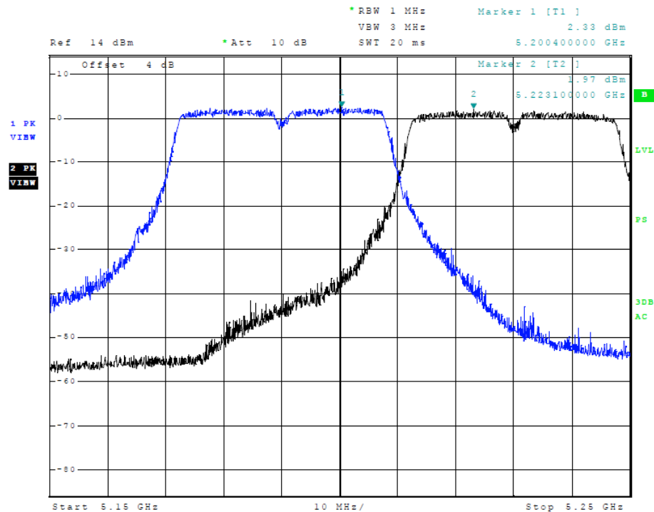
Figure 58 Plot of Transmitter Emissions (Across 5150-5250 MHz Band, 40 MHz Chnl, Chain 2)
