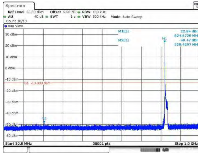
Band26_15MHz_16QAM_26865_1RB#0
