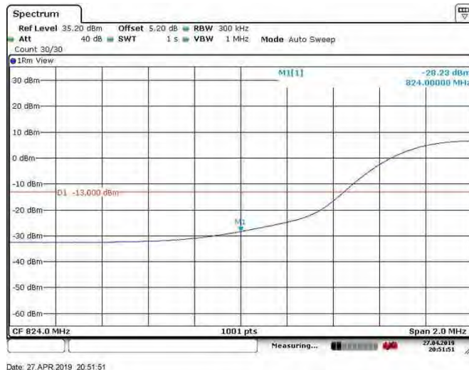
Band26_15MHz_16QAM_26965_1RB#74
