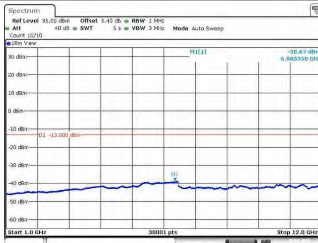
Band26_15MHz_QPSK_26915_1RB#0
