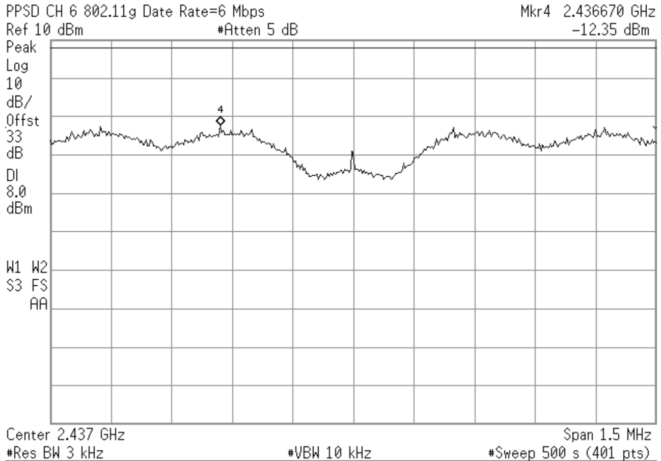
Plot F-5 - PPSD Mid Channel (802.11g)
