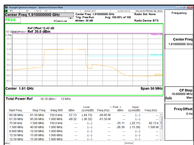
LTE2 15MHz 16QAM HIGH Ch RB75-0
