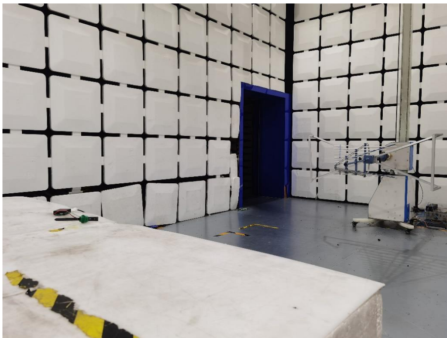
Description: Radiated Emission Test Setup for 30MHz ~ 1GHz (Mode1)
