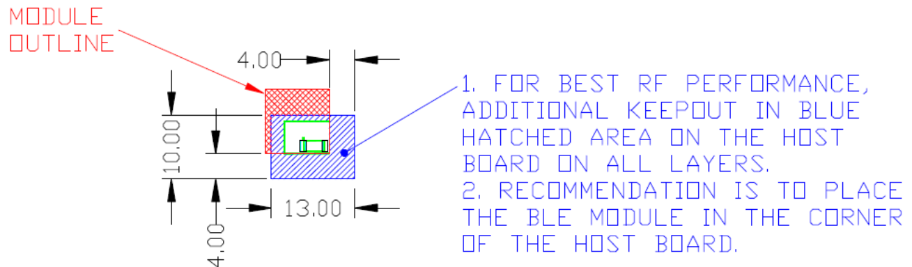
Host PCB Keep Out Area Around Chip Antenna
