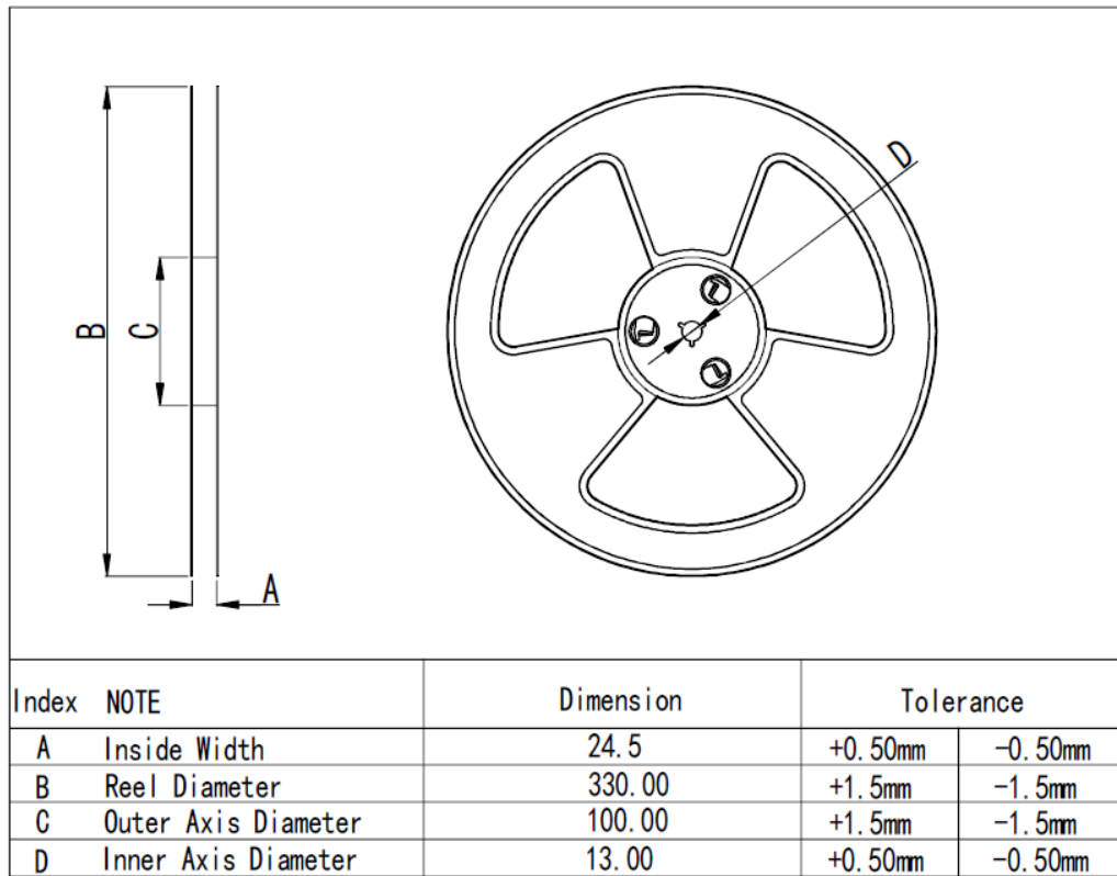
Figure 10. Reel Dimensions
