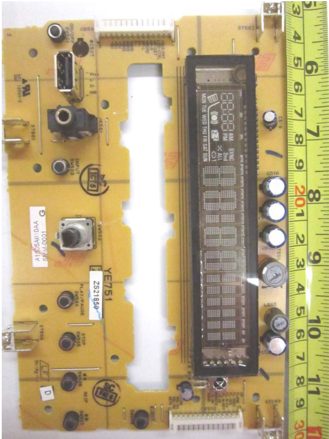
LCD Display PCB Component Side
