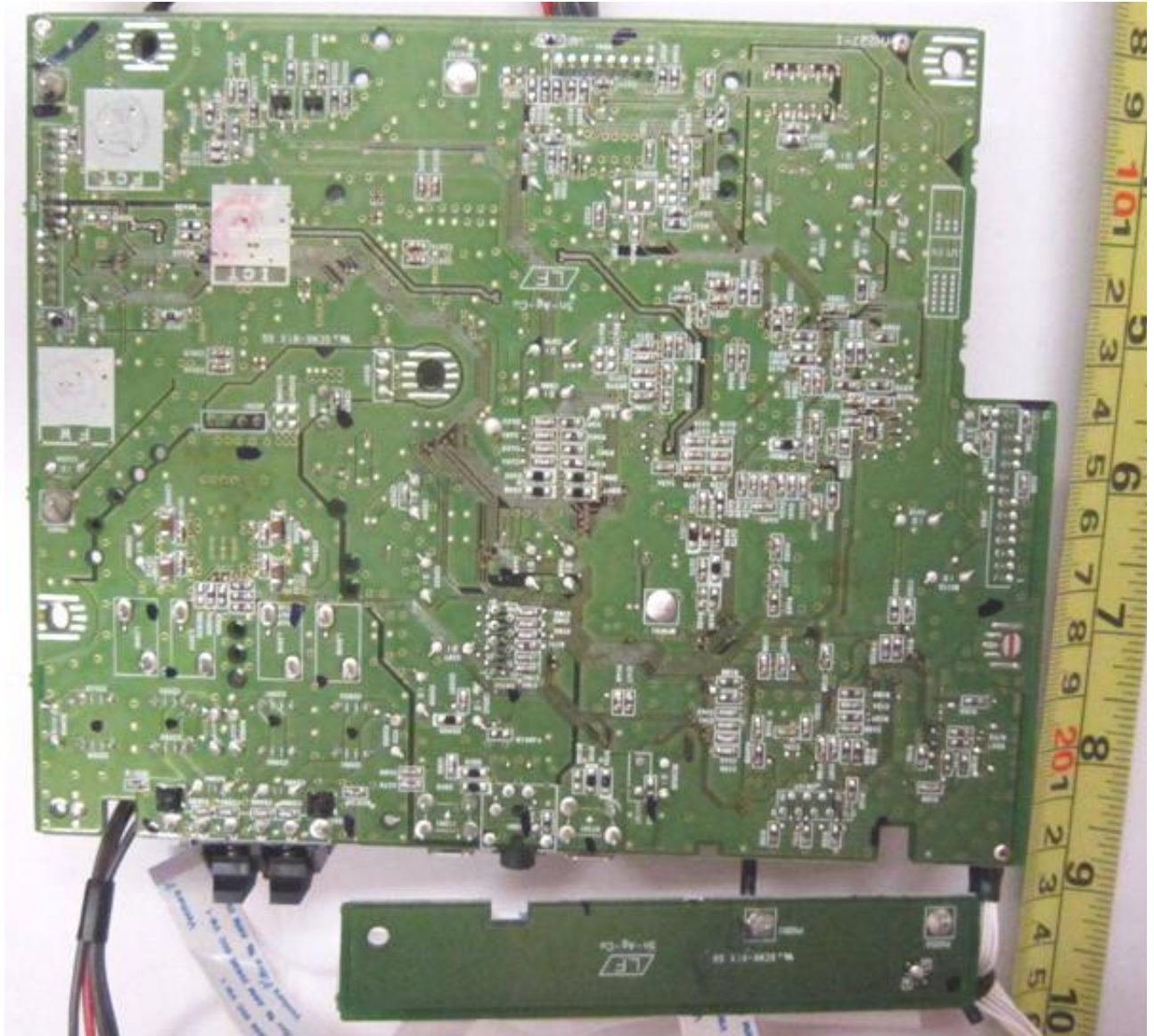
Main-Board PCB Trace Side
