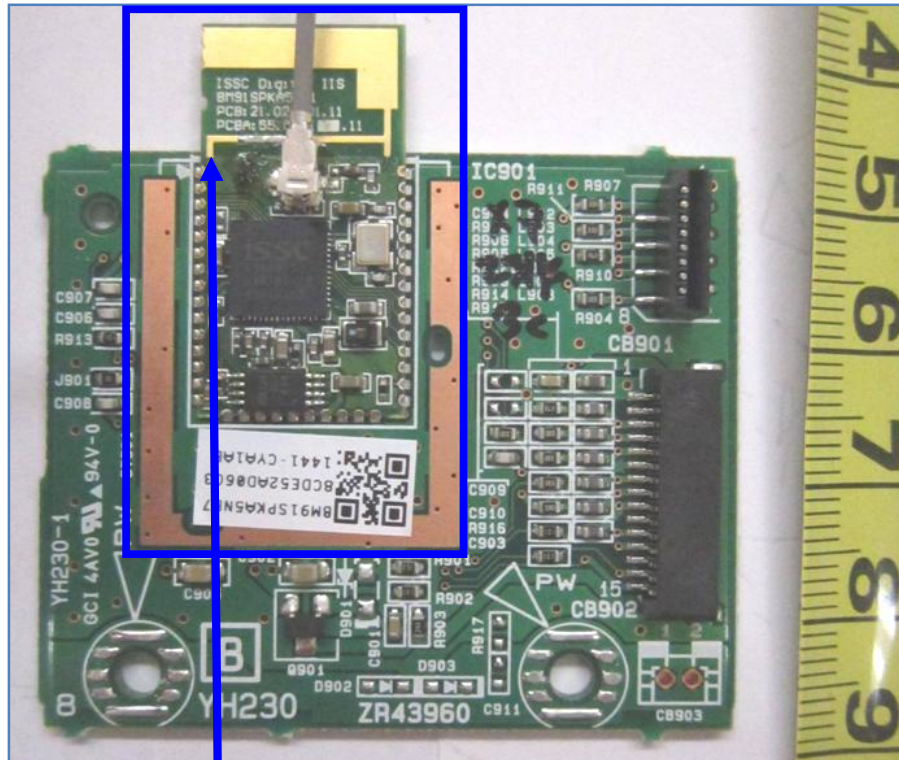
RF Module Circuit Component View
