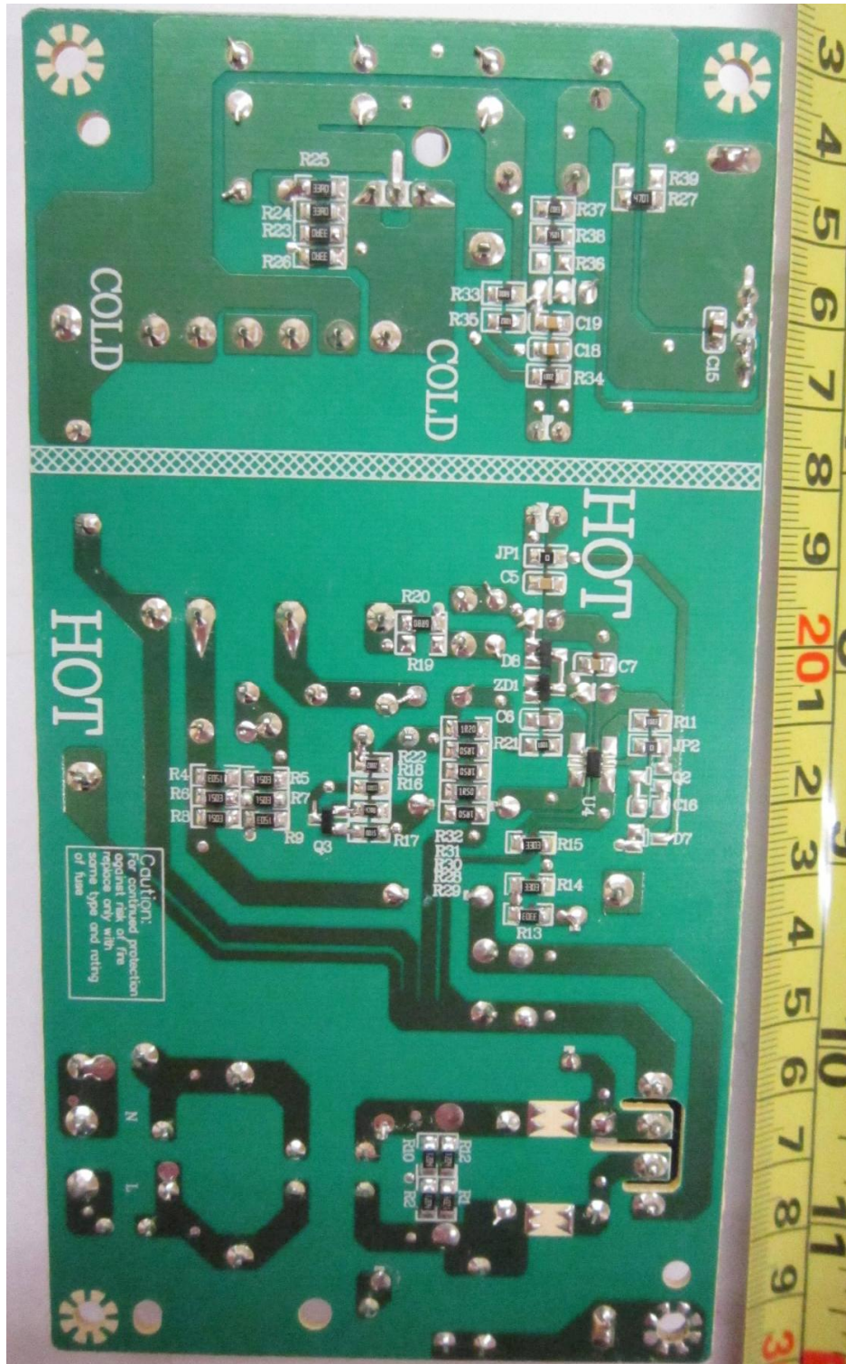
Power Supply PCB Trace Side
