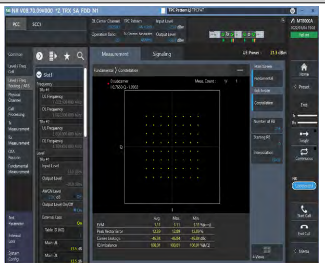
1-N25-15-40-M-4-DFT-64QAM-Out_Full-216@0-see graph-PASS
