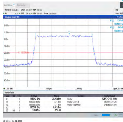
1-N25-PC3-15-10-L-9-CP-256QAM-Outter_Full-52@0-Ant1-9.285-9.960-≤10-PASS
