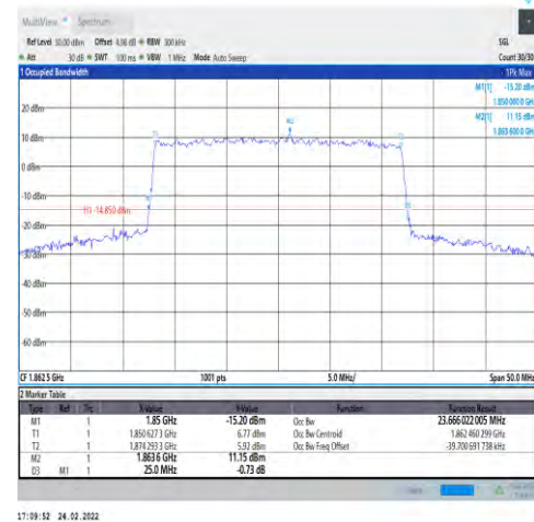
1-N25-PC3-15-25-L-8-CP-64QAM-Outer_Full-133@0-Ant1-23.666-25.000-≤25-PASS
