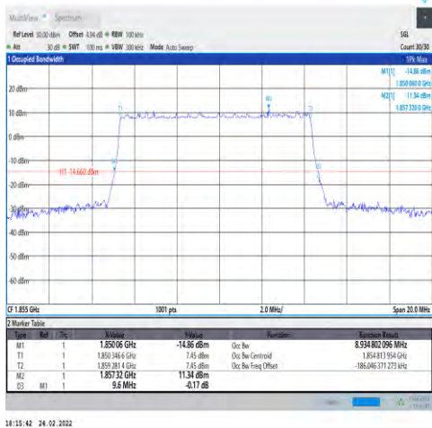
1-N25-PC3-15-10-L-4-DFT-64QAM-Outer_Full-50@0-Ant1-8.935-9.600-≤10-PASS
