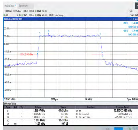
1-N25-PC3-15-15-H-4-DFT-64QAM-Outer_Full-75@0-Ant1-13.406-14.310-≤15-PASS
