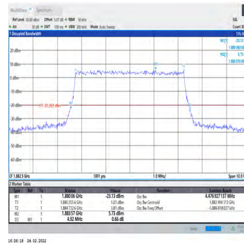
1-N25-PC3-15-5-M-9-CP-256QAM-Outer_Full-25@0-Ant1-4.477-4.920-≤5-PASS
