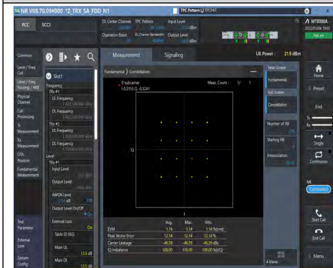
1-N25-15-40-M-3-DFT-16QAM-Out_Full-216@0-see graph-PASS
