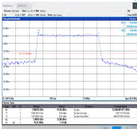
1-N25-PC3-15-15-H-3-DFT-16QAM-Outer_Full-75@0-Ant1-13.447-14.310-≤15-PASS
