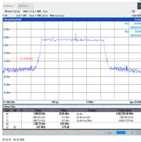
1-N25-PC3-15-5-M-8-CP-64QAM-Outer_Full-25@0-Ant1-4.462-4.910-≤5-PASS
