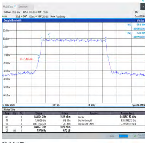
1-N25-PC3-15-5-M-4-DFT-64QAM-Outer_Ful I-25@0-Ant1-4.465-4.870-≤5-PASS
