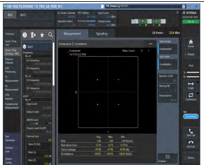
1-N25-15-40-M-2-DFT-QPSK-Out_Full-216@0-see graph-PASS
