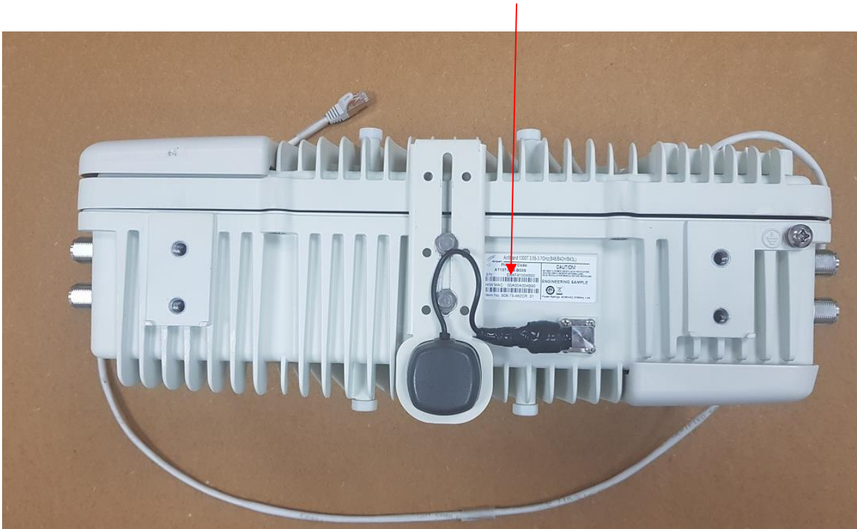
“ AirStrand AS1300T 3.55-3.7 GHz (B48)” side panel, label with FCC ID: PIDAS1300B48 location
