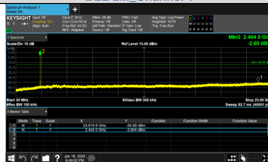
30.0 MHz - 25000.0 MHz BLE 2M_Channel 1
