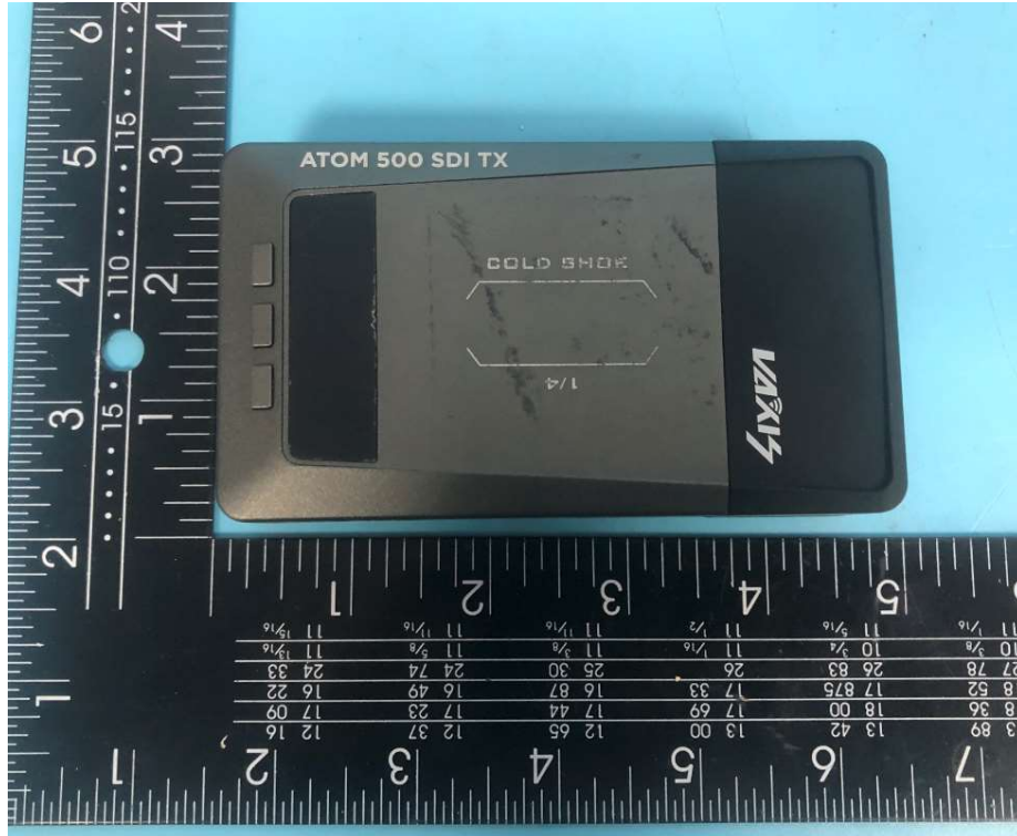
Photo 1(Transmitter)
