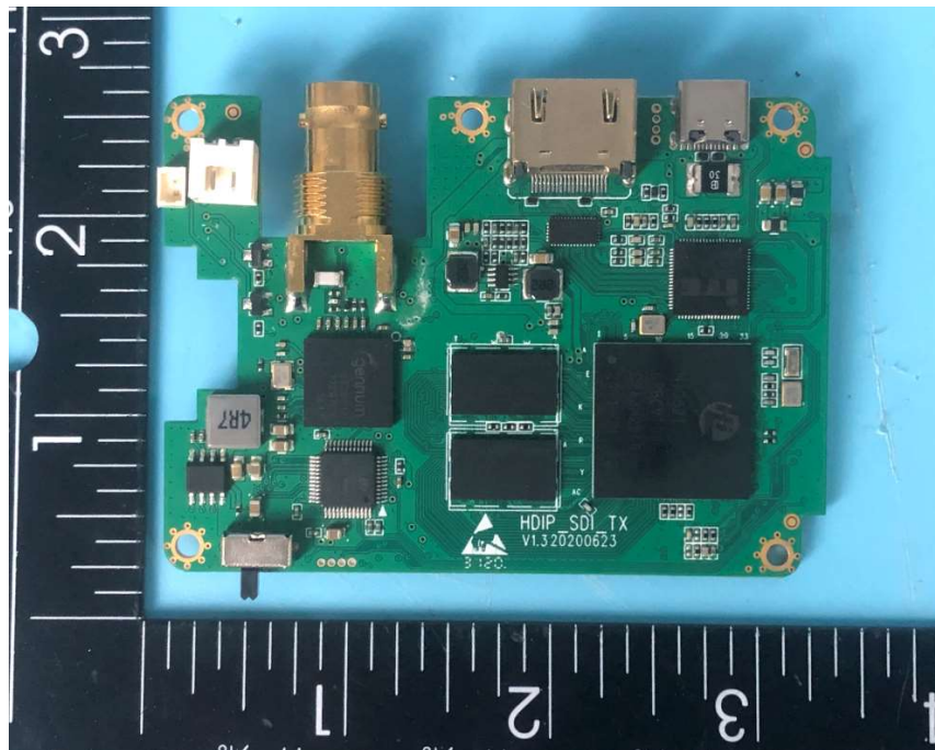
Photo 15(Transmitter)
