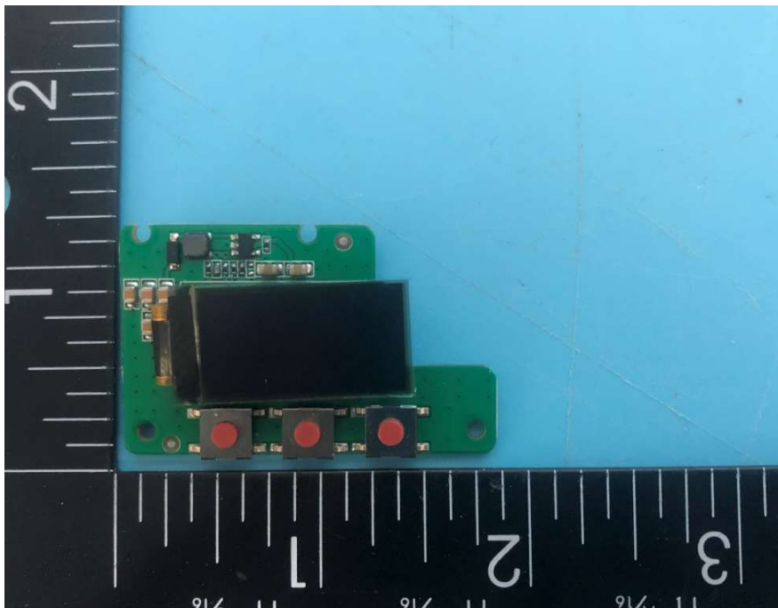
Photo 5(Transmitter)
