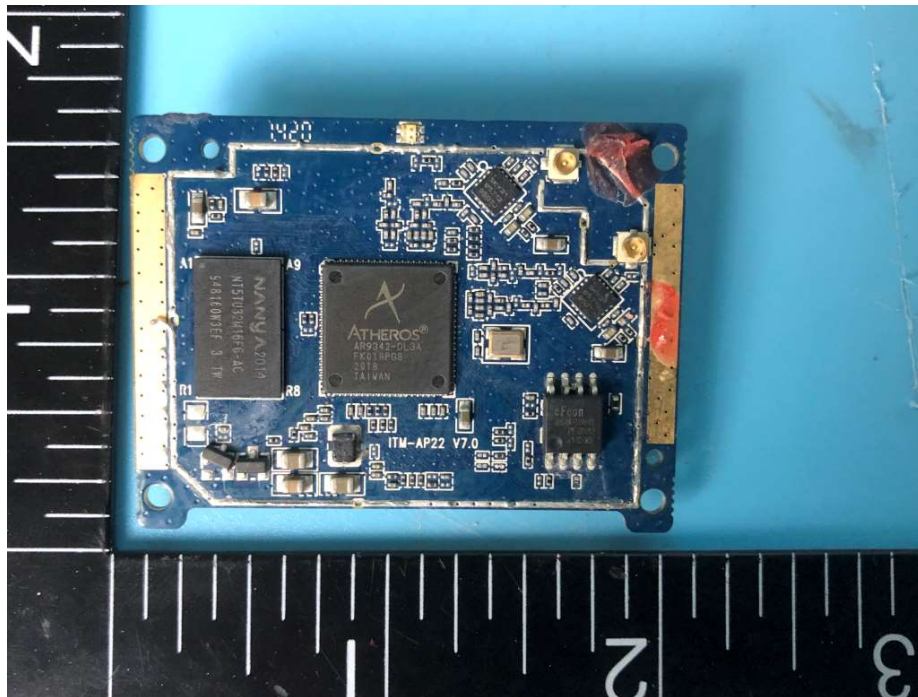
Photo 23(Transmitter)
