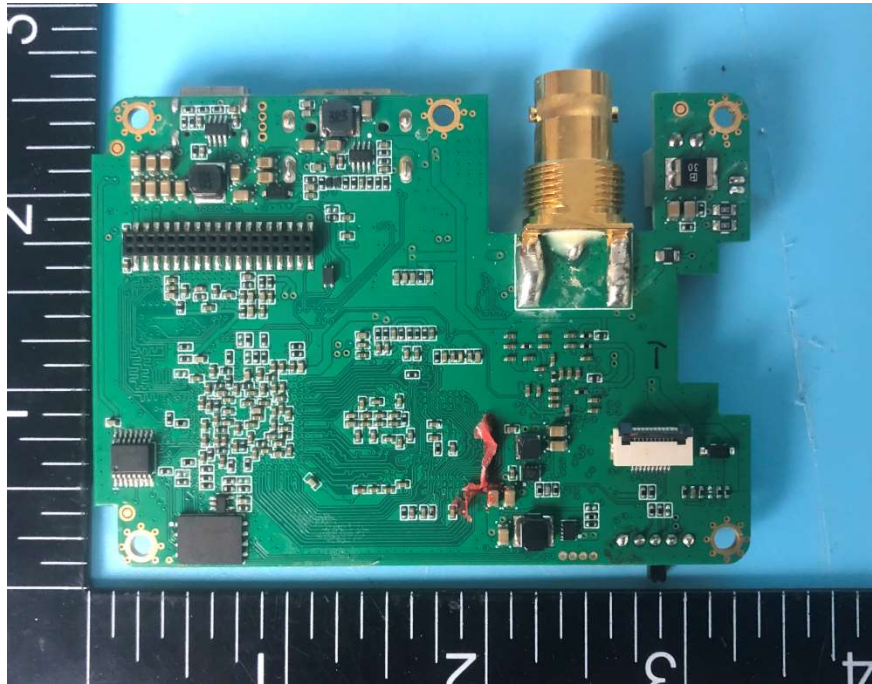
Photo 11(Transmitter)
