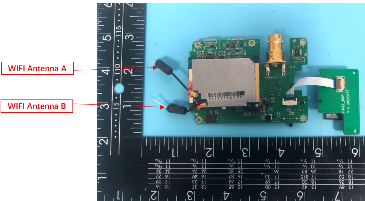
Photo 4(Transmitter)
