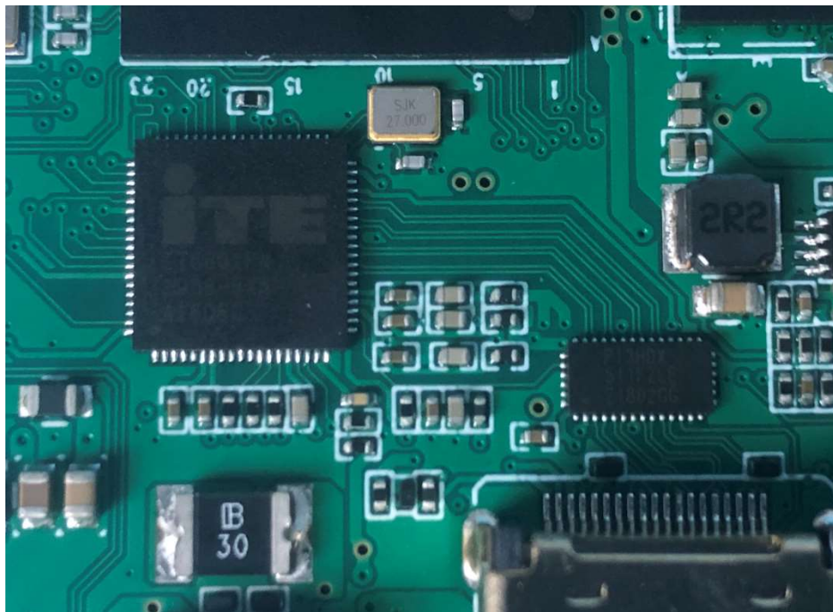
Photo 17(Transmitter)
