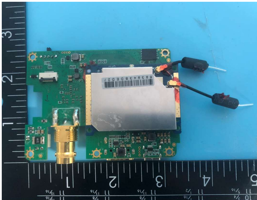
Photo 7(Transmitter)
