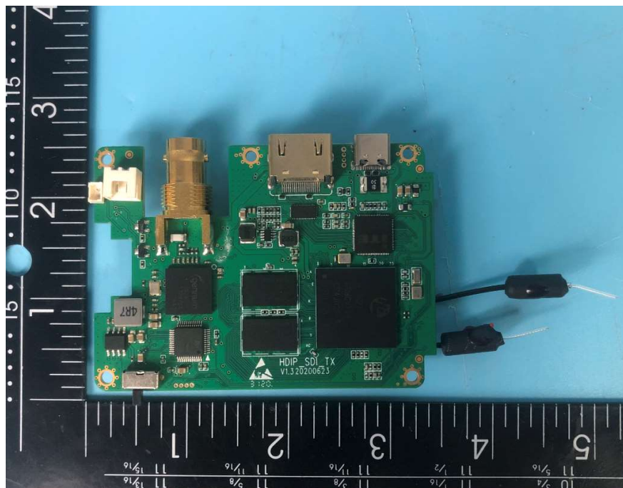
Photo 8(Transmitter)
