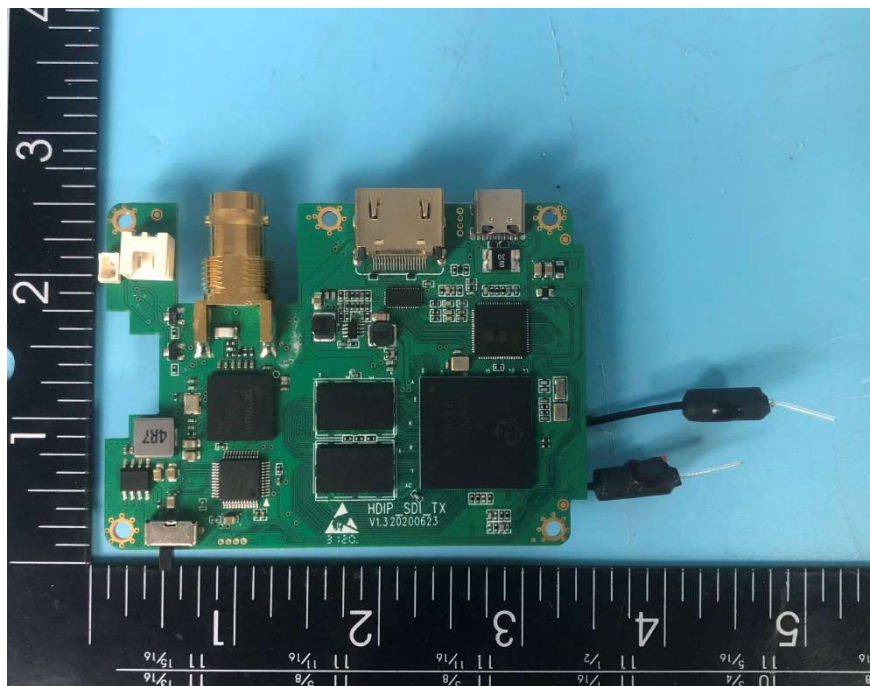
Photo 9(Transmitter)
