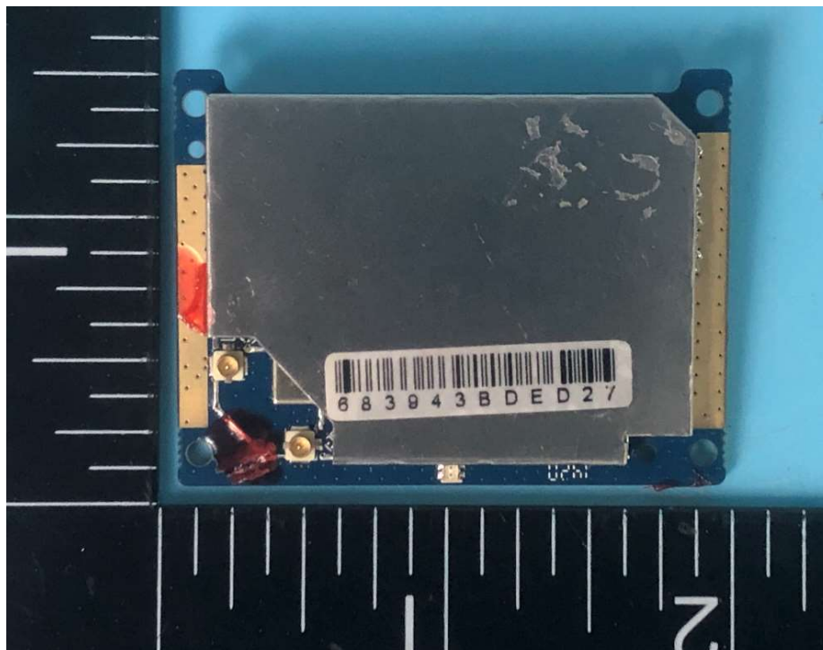
Photo 22(Transmitter)
