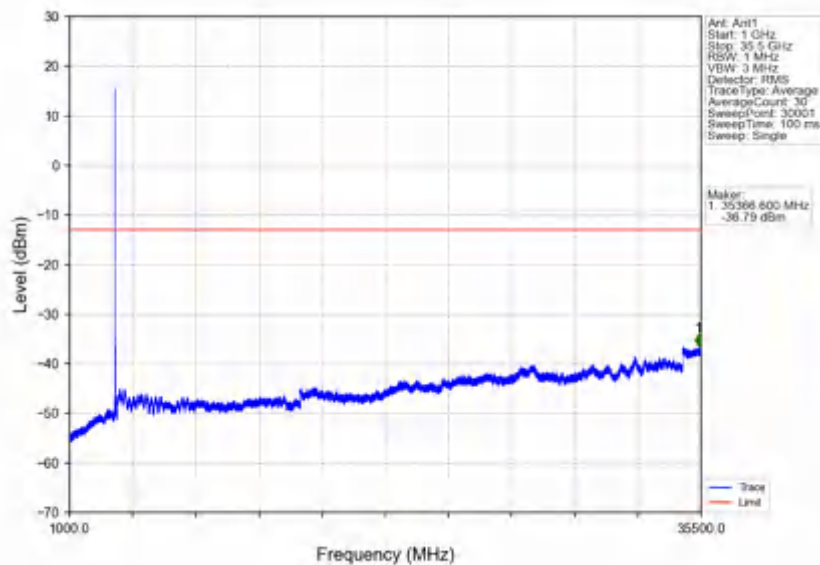
n78e_30kHz_SISO_NTNV_40MHz_DFT-s-OFDM QPSK_3529.98MHz_Edge_1RB_Right
