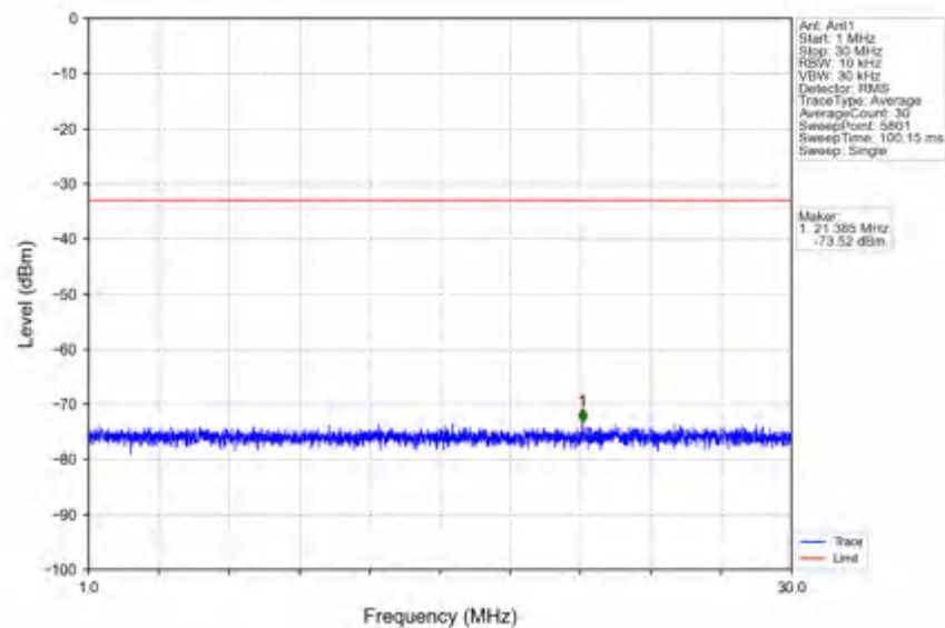
n78e_30kHz_SISO_NTNV_30MHz_CP-OFDM QPSK_3534.99MHz_Inner_1RB_Right
