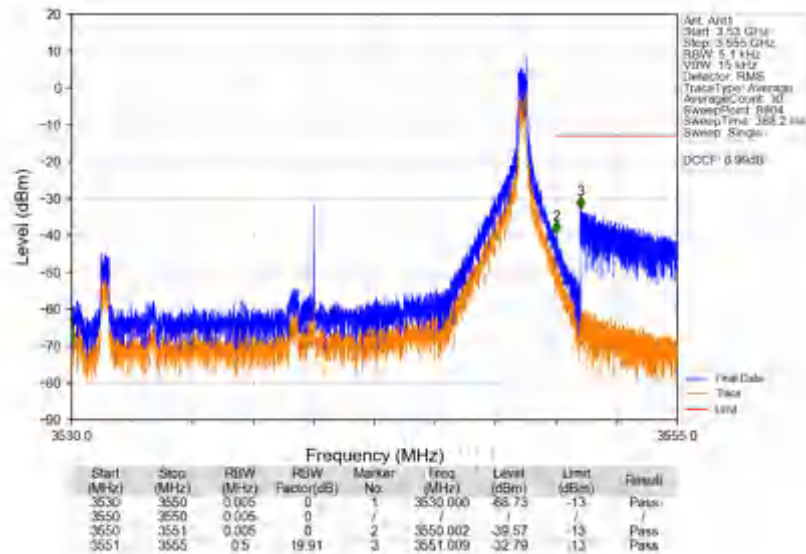
n78e_30kHz_SISO_NTNV_20MHz_DFT-s-OFDM QPSK_3540MHz_Inner_1RB_Right
