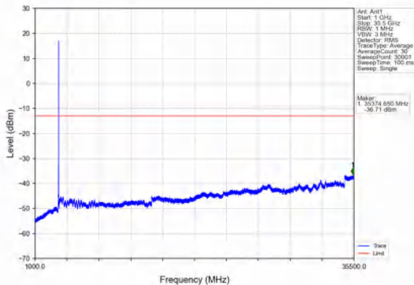
n78e_30kHz_SISO_NTNV_30MHz_CP-OFDM QPSK_3534.99MHz_Outer_Full
