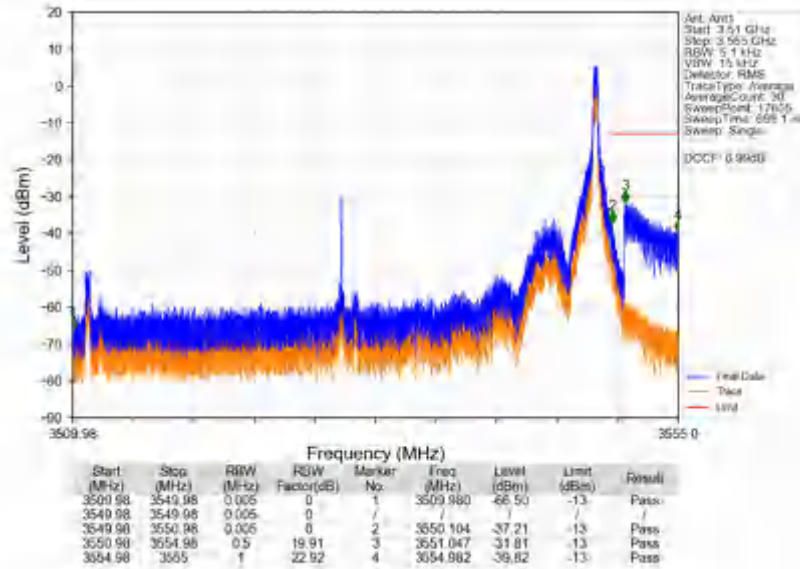
n78e_30kHz_SISO_NTNV_40MHz_CP-OFDM QPSK_3529.98MHz_Edge_1RB_Right
