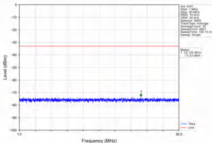
n78e_30kHz_SISO_NTNV_25MHz_CP-OFDM QPSK_3537.48MHz_Inner_1RB_Right
