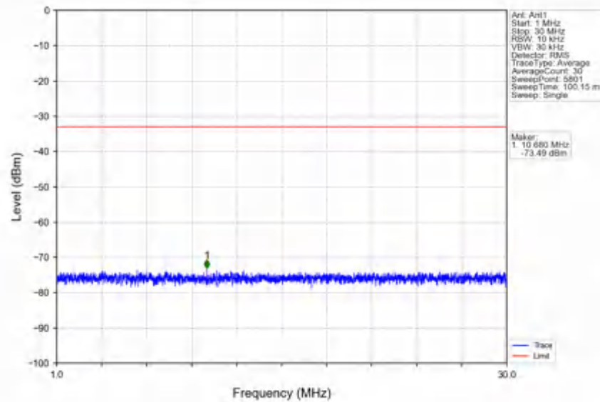
n78e_30kHz_SISO_NTNV_40MHz_DFT-s-OFDM_QPSK_3529.98MHz_Outer_Full
