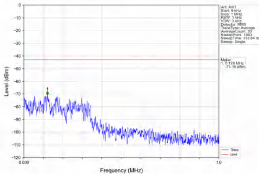
n78e_30kHz_SISO_NTNV_40MHz_DFT-s-OFDM_PI/2_BPSK_3470.01MHz_Edge_1RB_Left
