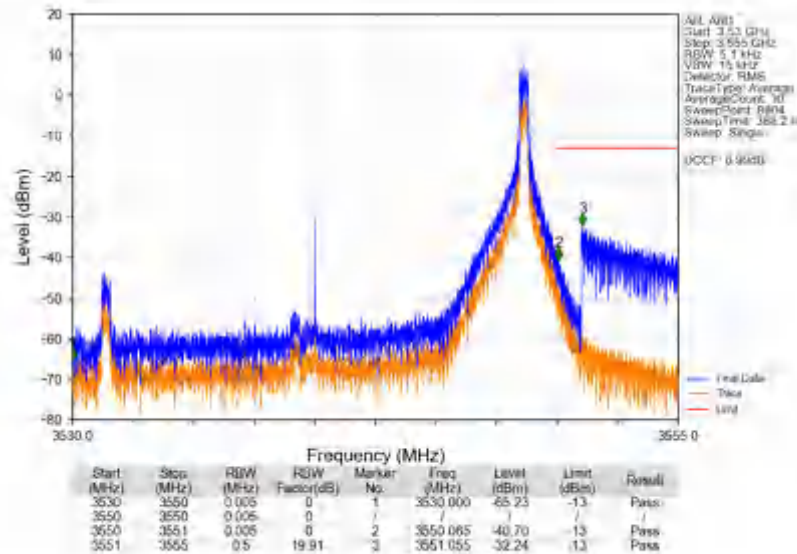
n78e_30kHz_SISO_NTNV_20MHz_CP-OFDM_QPSK_3540MHz_Inner_1RB_Right
