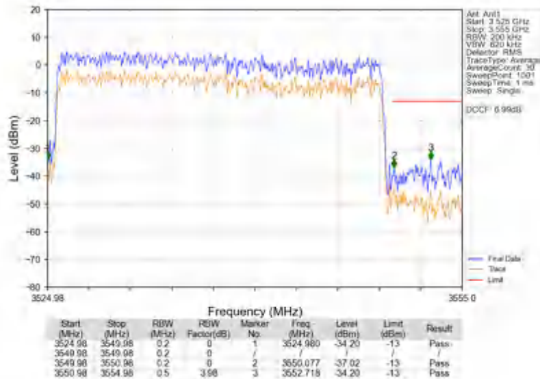
n78e_30kHz_SISO_NTNV_25MHz_CP-OFDM QPSK_3537.48MHz_Outer_Full
