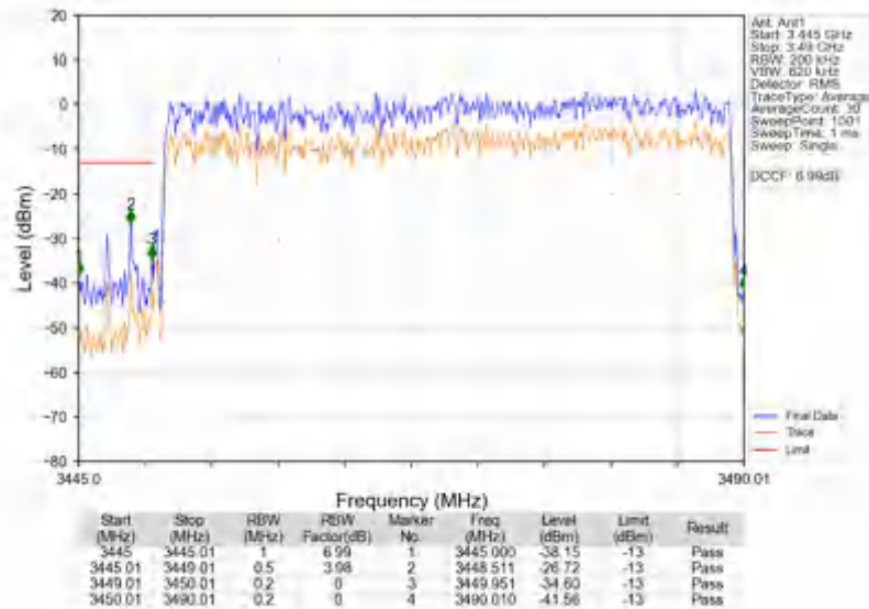
n78e_30kHz_SISO_NTV_40MHz_CP-OFDM QPSK_3470.01MHz_Outer_Full
