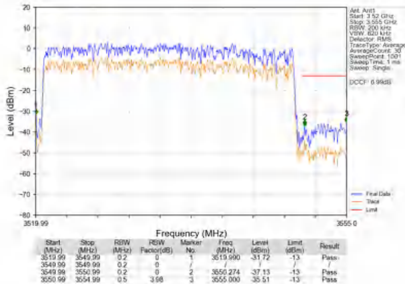
n78e_30kHz_SISO_NTNV_30MHz_CP-OFDM QPSK_3534.99MHz_Outer_Full
