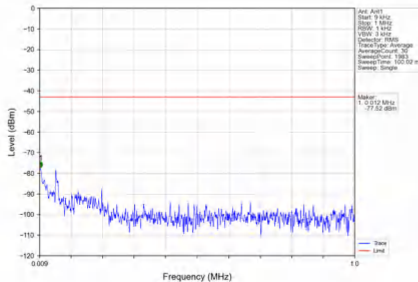
n78e_30kHz_SISO_NTNV_20MHz_DFT-s-OFDM_QPSK_3540MHz_Outer_Full
