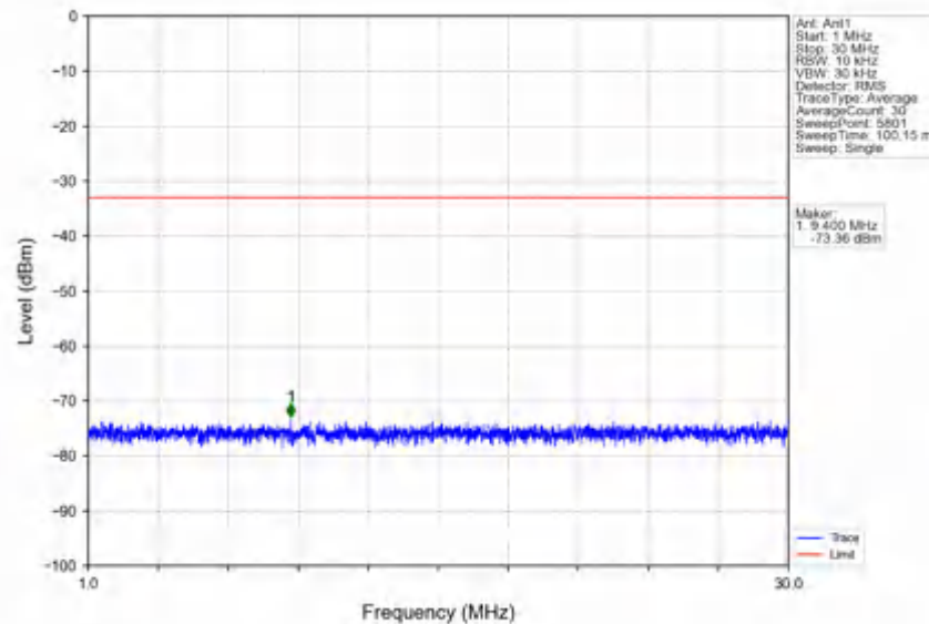
n78e_30kHz_SISO_NTNV_30MHz_CP-OFDM_QPSK_3465MHz_Outer_Full
