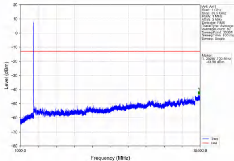
n78e_30kHz_SISO_NTNV_20MHz_DFT-s-OFDM QPSK_3540MHz_Inner_1RB_Right
