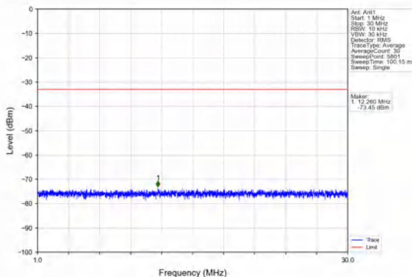
n78e_30kHz_SISO_NTNV_40MHz_DFT-s-OFDM_QPSK_3470.01MHz_Outer_Full
