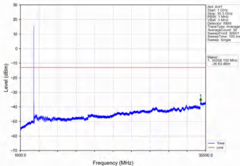
n78e_30kHz_SISO_NTNV_25MHz_DFT-s-OFDM_QPSK_3537.48MHz_Edge_1RB_Right
