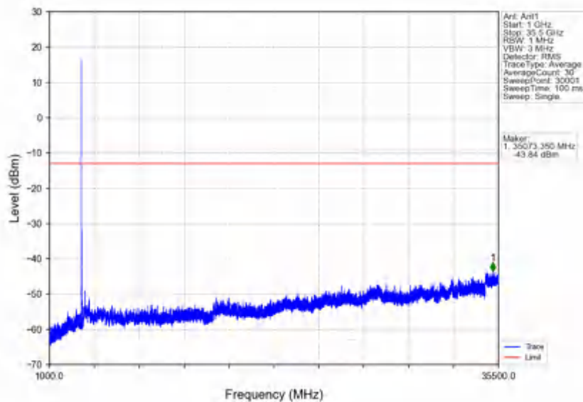
n78e_30kHz_SISO_NTV_20MHz_CP-OFDM QPSK_3460.02MHz_Outer_Full
