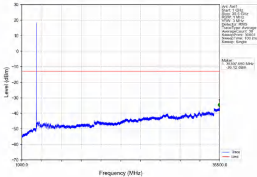
n78e_30kHz_SISO_NTNV_40MHz_CP-OFDM QPSK_3529.98MHz_Outer_Full
