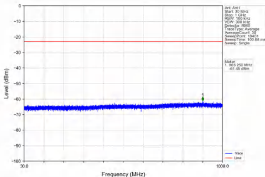
n78e_30kHz_SISO_NTNV_20MHz_CP-OFDM_QPSK_3540MHz_Outer_Full
