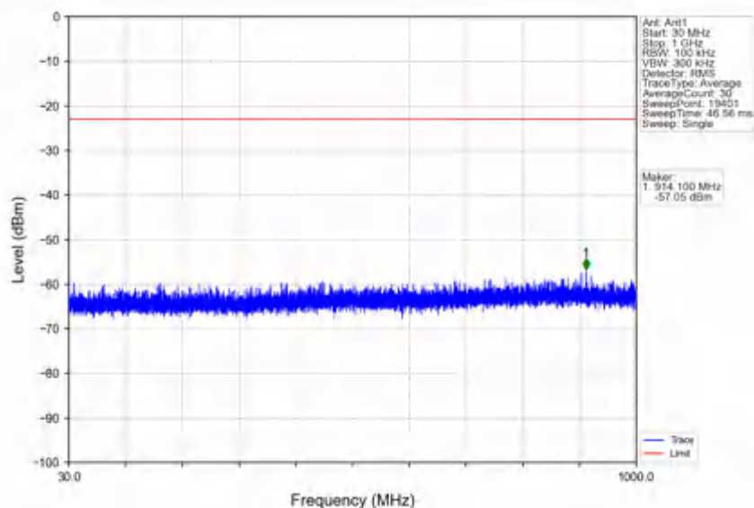
n78e_30kHz_SISO_NTNV_50MHz_DFT-s-OFDM_QPSK_3475.02MHz_Edge_1RB_Left
