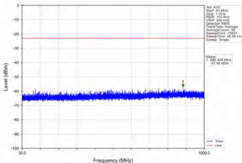
n78e_30kHz_SISO_NTV_40MHz_CP-OFDM QPSK_3500.01MHz_Edge_1RB_Left
