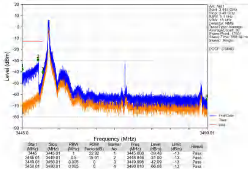
n78e_30kHz_SISO_NTV_40MHz_CP-OFDM_QPSK_3470.01MHz_Inner_1RB_Left
