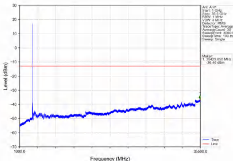
n78e_30kHz_SISO_NTNV_50MHz_DFT-s-OFDM_QPSK_3475.02MHz_Edge_1RB_Left
