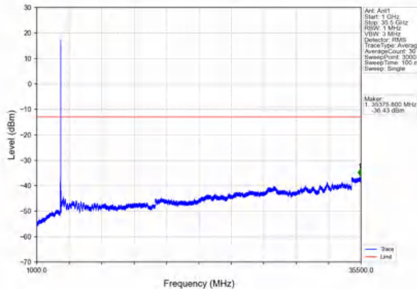
n78e_30kHz_SISO_NTNV_30MHz_DFT-s-OFDM QPSK_3534.99MHz_Inner_1RB_Right
