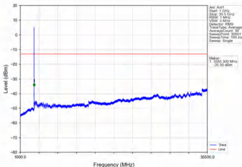
n78e_30kHz_SISO_NTNV_20MHz_CP-OFDM_QPSK_3540MHz_Outer_Full
