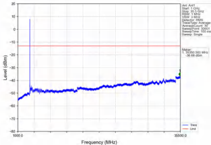
n78e_30kHz_SISO_NTNV_25MHz_DFT-s-OFDM_QPSK_3537.48MHz_Inner_1RB_Right
