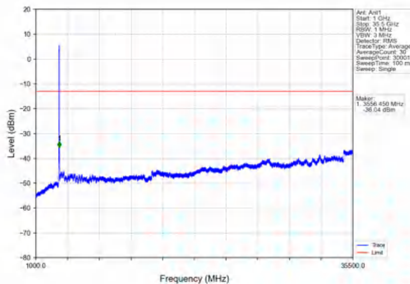
n78e_30kHz_SISO_NTNV_40MHz_CP-OFDM_QPSK_3529.98MHz_Outer_Full
