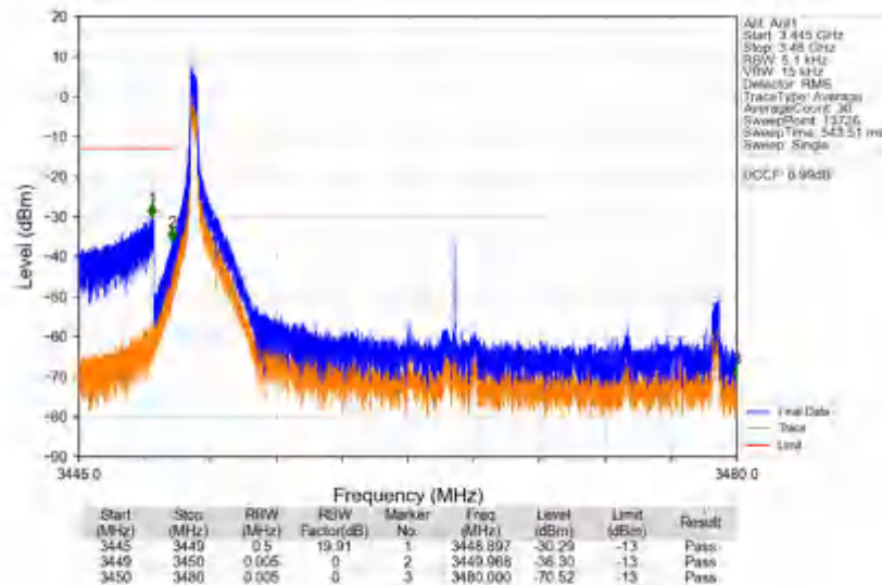
n78e_30kHz_SISO_NTNV_30MHz_DFT-s-OFDM_PI/2_BPSK_3465MHz_Edge_1RB_Left
