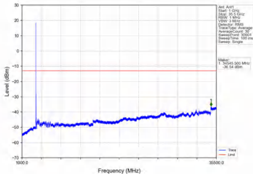
n78e_30kHz_SISO_NTV_40MHz_CP-OFDM QPSK_3470.01MHz_Outer_Full
