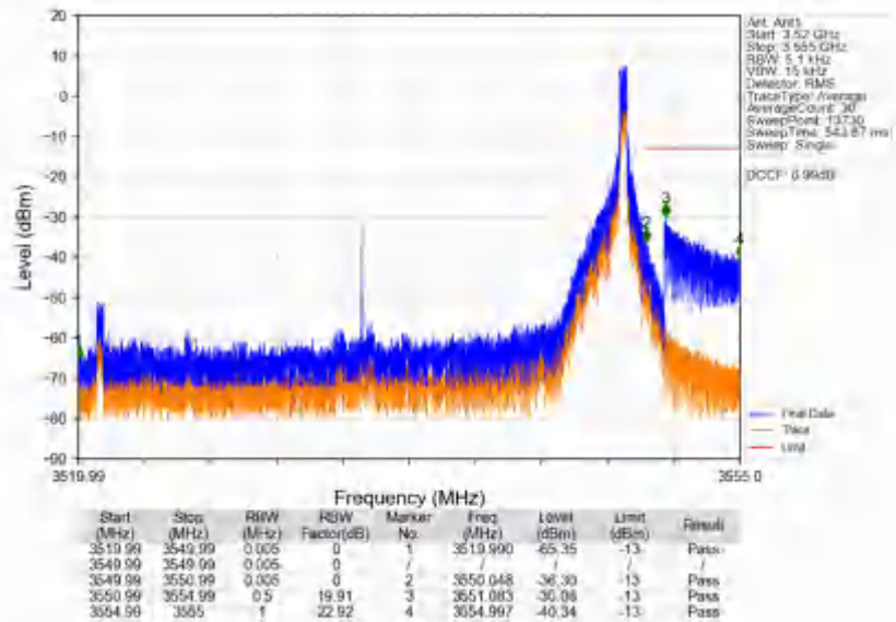
n78e_30kHz_SISO_NTNV_30MHz_DFT-s-OFDM QPSK_3534.99MHz_Edge_1RB_Right
