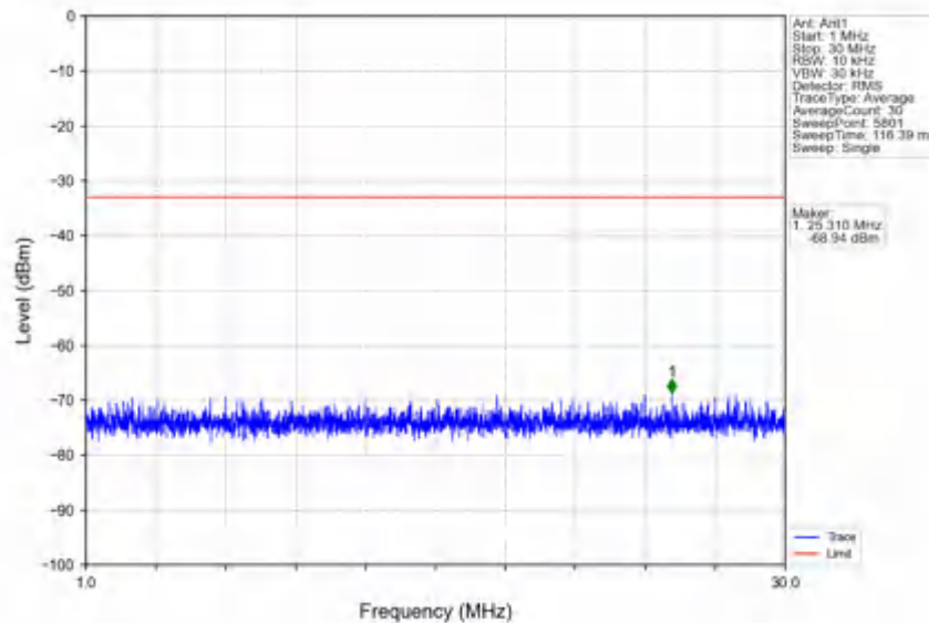
n78e_30kHz_SISO_NTNV_40MHz_DFT-s-OFDM_QPSK_3470.01MHz_Edge_1RB_Left
