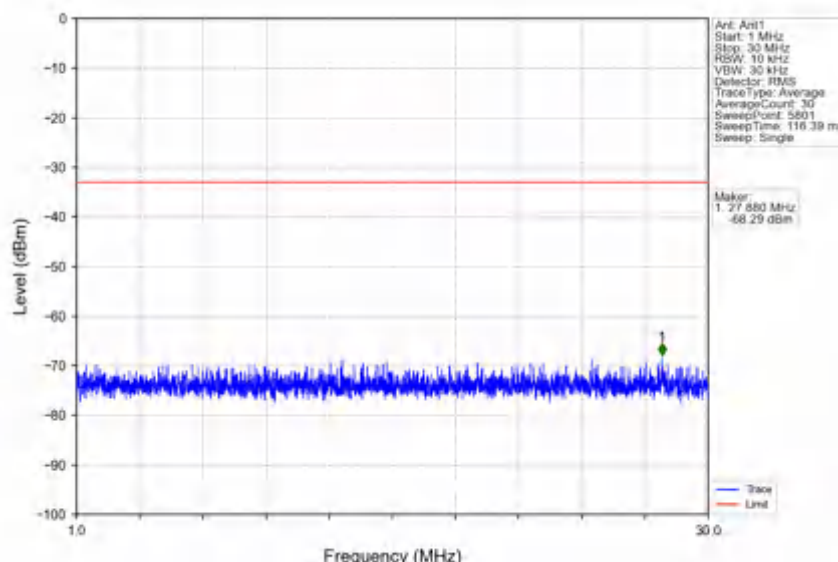
n78e_30kHz_SISO_NTNV_20MHz_CP-OFDM QPSK_3540MHz_Edge_1RB_Right
