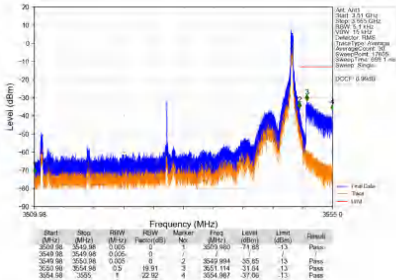
n78e_30kHz_SISO_NTNV_40MHz_DFT-s-OFDM QPSK_3529.98MHz_Edge_1RB_Right
