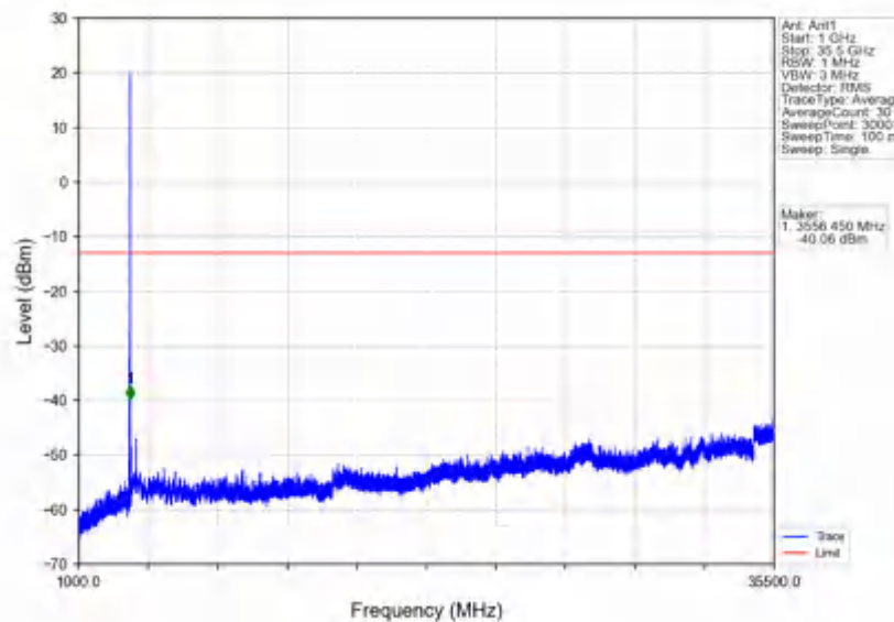
n78e_30kHz_SISO_NTNV_20MHz_DFT-s-OFDM QPSK_3540MHz_Inner_1RB_Right
