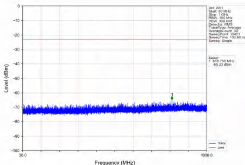
n78e_30kHz_SISO_NTNV_20MHz_DFT-s-OFDM QPSK_3540MHz_Outer_Full
