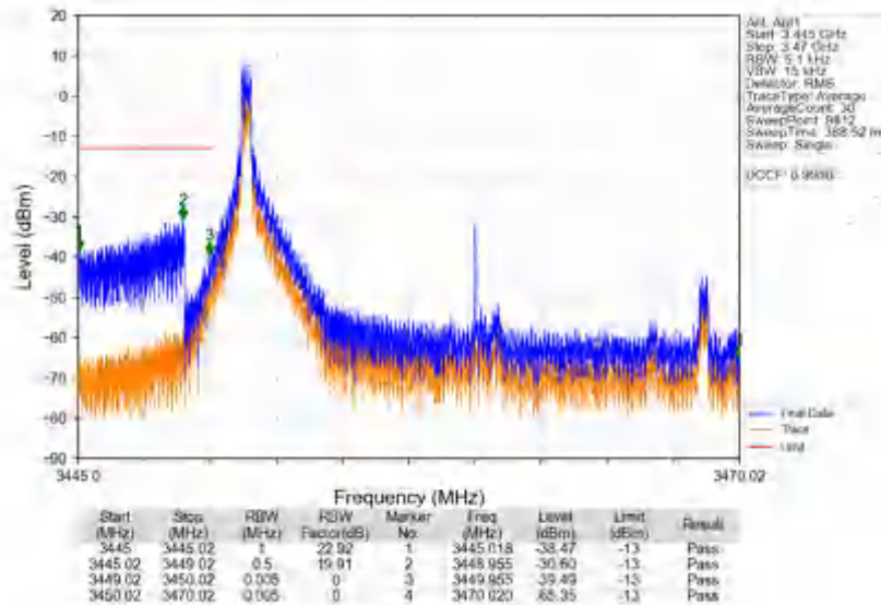
n78e_30kHz_SISO_NTNV_20MHz_DFT-s-OFDM_QPSK_3460.02MHz_Inner_1RB_Left
