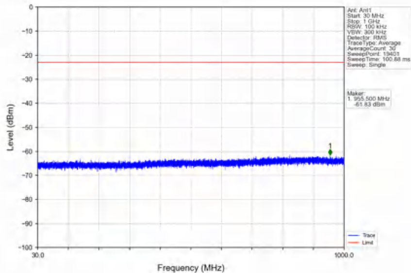
n78e_30kHz_SISO_NTNV_30MHz_DFT-s-OFDM_QPSK_3534.99MHz_Outer_Full
