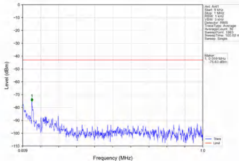
n78e_30kHz_SISO_NTNV_20MHz_DFT-s-OFDM_QPSK_3460.02MHz_Outer_Full
