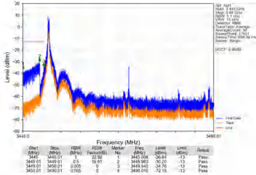
n78e_30kHz_SISO_NTNV_40MHz_DFT-s-OFDM_PI/2_BPSK_3470.01MHz_Edge_1RB_Left
