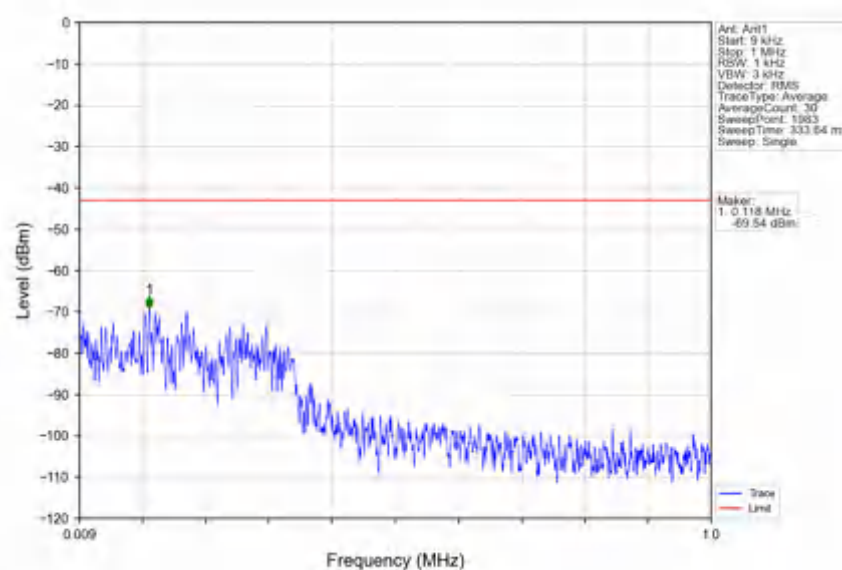
n78e_30kHz_SISO_NTNV_30MHz_DFT-s-OFDM_PI/2_BPSK_3465MHz_Edge_1RB_Left
