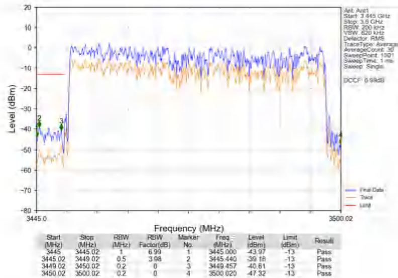
n78e_30kHz_SISO_NTNV_50MHz_DFT-s-OFDM_QPSK_3475.02MHz_Outer_Full
