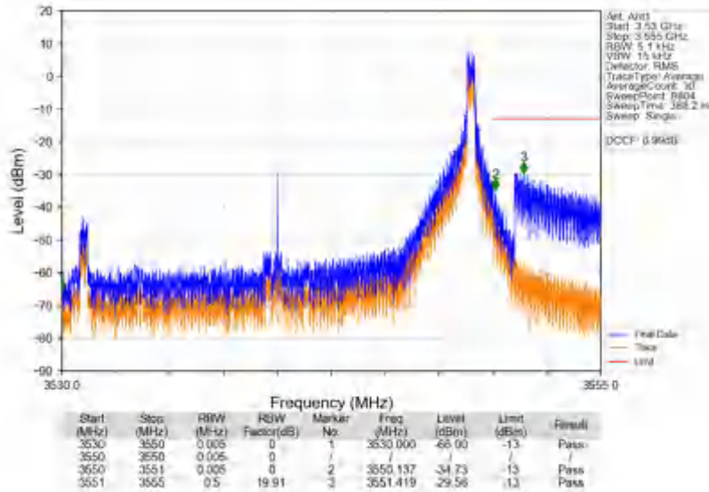
n78e_30kHz_SISO_NTNV_20MHz_DFT-s-OFDM QPSK_3540MHz_Edge_1RB_Right
