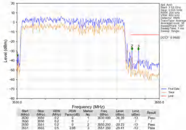
n78e_30kHz_SISO_NTNV_20MHz_DFT-s-OFDM_QPSK_3540MHz_Outer_Full
