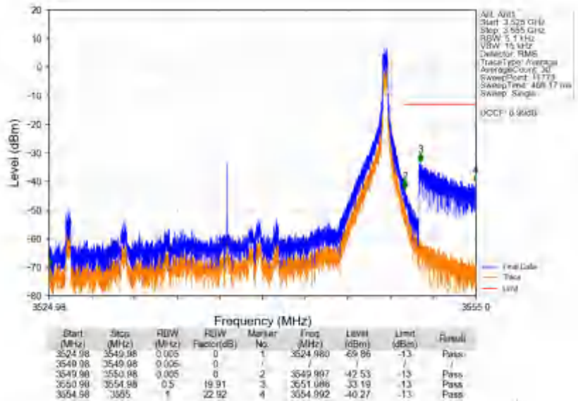
n78e_30kHz_SISO_NTNV_25MHz_DFT-s-OFDM_QPSK_3537.48MHz_Inner_1RB_Right
