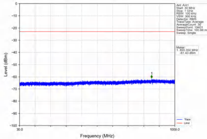
n78e_30kHz_SISO_NTNV_40MHz_DFT-s-OFDM QPSK_3529.98MHz_Inner_1RB_Right
