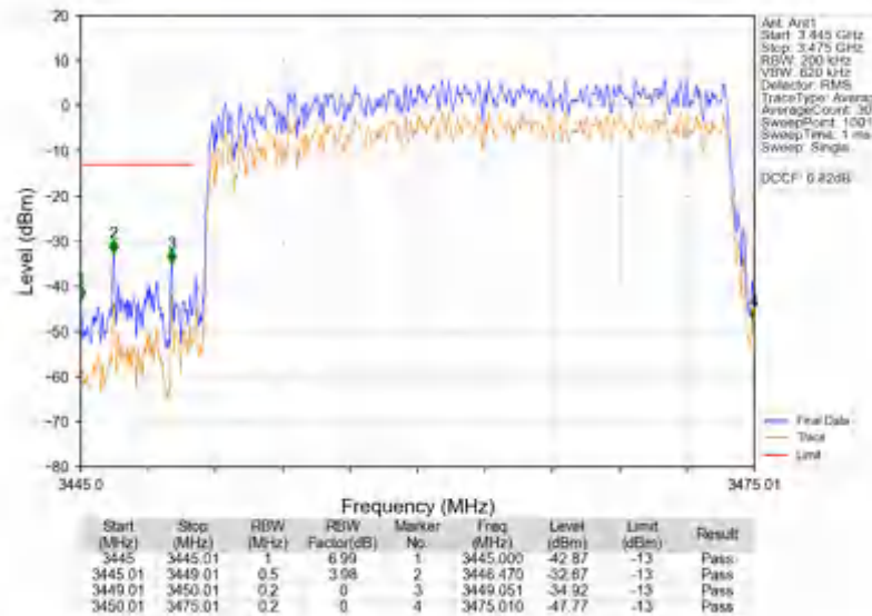
n78e_30kHz_SISO_NTNV_25MHz_DFT-s-OFDM_QPSK_3462.51MHz_Outer_Full
