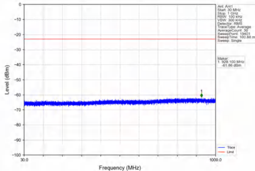
n78e_30kHz_SISO_NTNV_40MHz_CP-OFDM QPSK_3529.98MHz_Inner_1RB_Right
