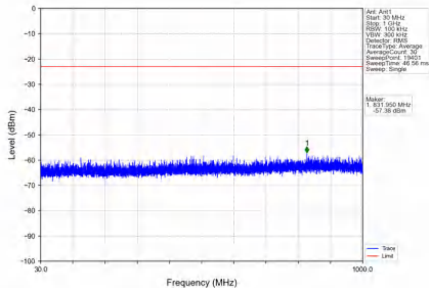
n78e_30kHz_SISO_NTNV_25MHz_CP-OFDM QPSK_3537.48MHz_Edge_1RB_Right
