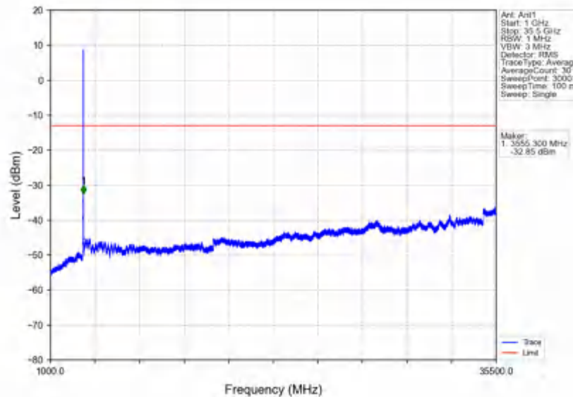
n78e_30kHz_SISO_NTNV_25MHz_CP-OFDM QPSK_3537.48MHz_Outer_Full
