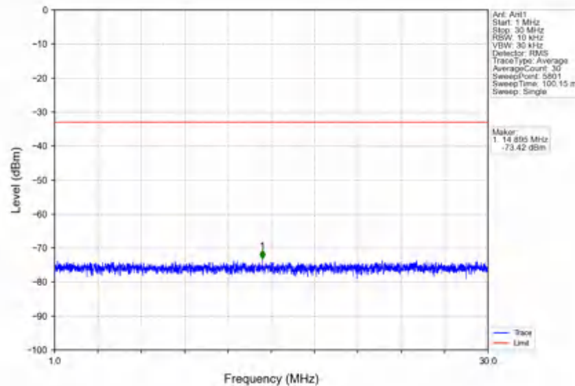
n78e_30kHz_SISO_NTNV_20MHz_CP-OFDM_QPSK_3540MHz_Outer_Full
