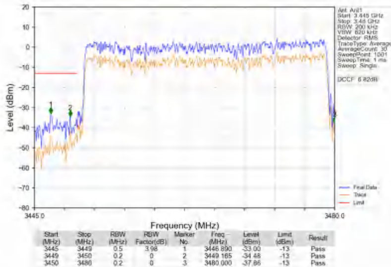
n78e_30kHz_SISO_NTNV_30MHz_CP-OFDM QPSK_3465MHz_Outer_Full
