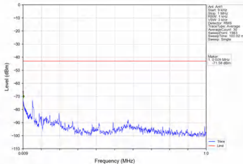
n78e_30kHz_SISO_NTNV_50MHz_DFT-s-OFDM_QPSK_3475.02MHz_Outer_Full
