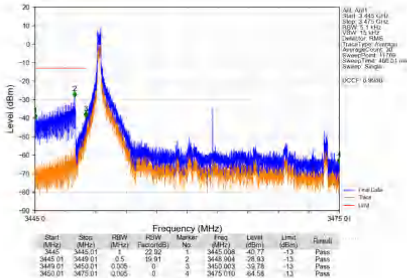
n78e_30kHz_SISO_NTNV_25MHz_DFT-s-OFDM_QPSK_3462.51MHz_Inner_1RB_Left
