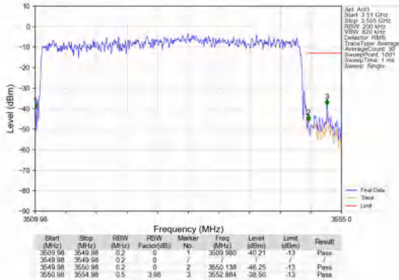
n78e_30kHz_SISO_NTNV_40MHz_CP-OFDM QPSK_3529.98MHz_Outer_Full
