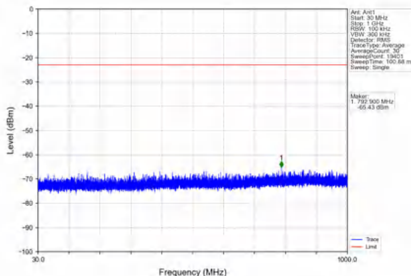
n78e_30kHz_SISO_NTNV_20MHz_CP-OFDM_QPSK_3540MHz_Inner_1RB_Right
