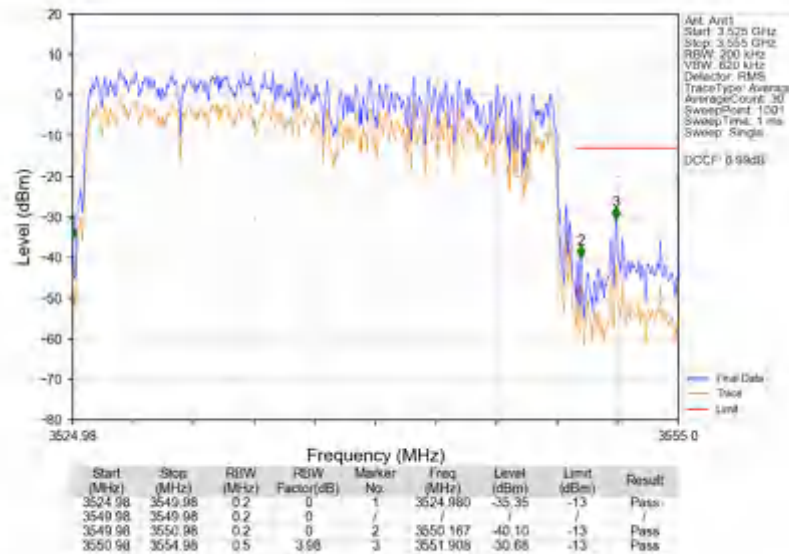
n78e_30kHz_SISO_NTNV_25MHz_DFT-s-OFDM_QPSK_3537.48MHz_Outer_Full
