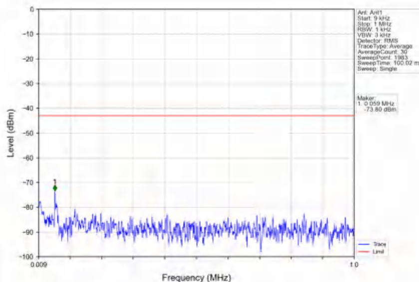
n78e_30kHz_SISO_NTNV_25MHz_CP-OFDM QPSK_3537.48MHz_Outer_Full
