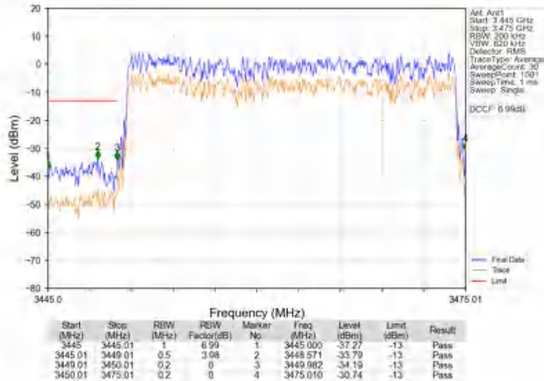
n78e_30kHz_SISO_NTV_25MHz_CP-OFDM QPSK_3462.51MHz_Outer_Full
