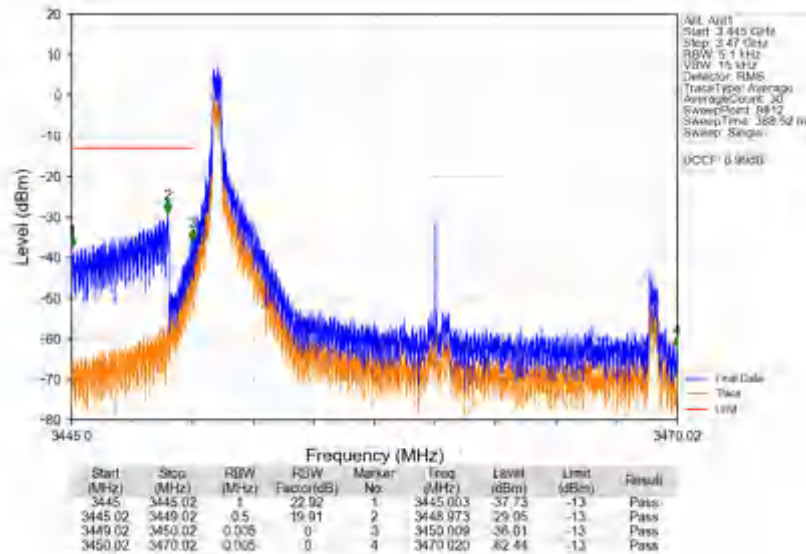
n78e_30kHz_SISO_NTNV_20MHz_DFT-s-OFDM QPSK_3460.02MHz_Edge_1RB_Left
