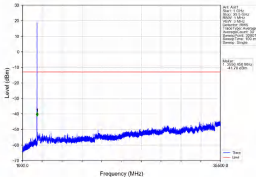
n78e_30kHz_SISO_NTNV_20MHz_DFT-s-OFDM QPSK_3460.02MHz_Edge_1RB_Left
