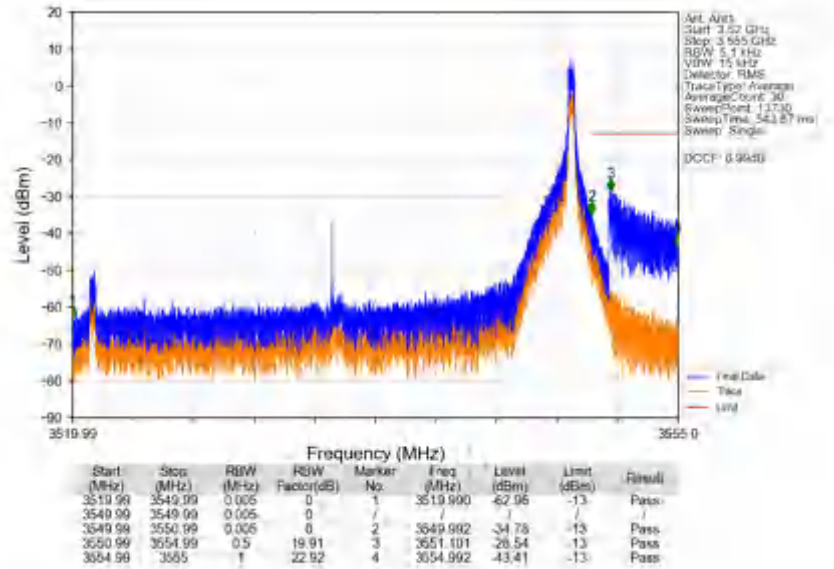
n78e_30kHz_SISO_NTNV_30MHz_CP-OFDM QPSK_3534.99MHz_Edge_1RB_Right
