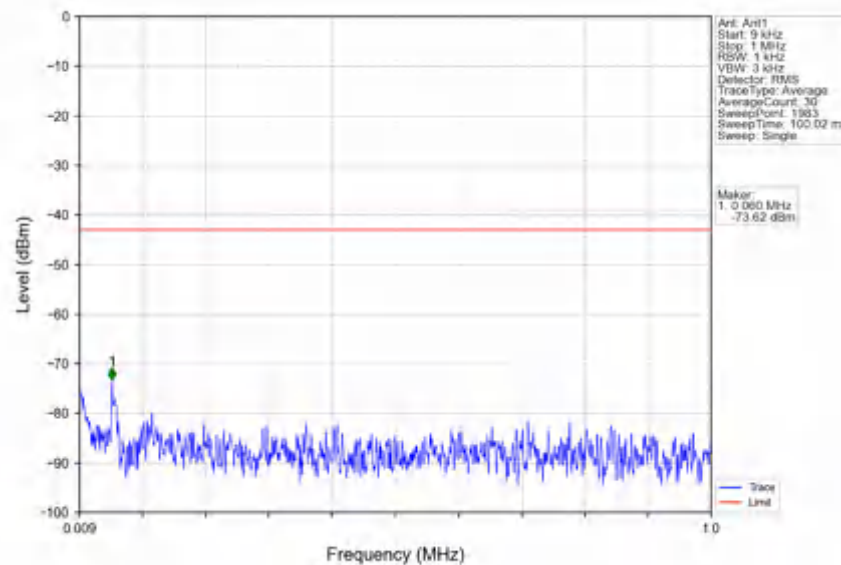
n78e_30kHz_SISO_NTNV_25MHz_CP-OFDM QPSK_3462.51MHz_Outer_Full
