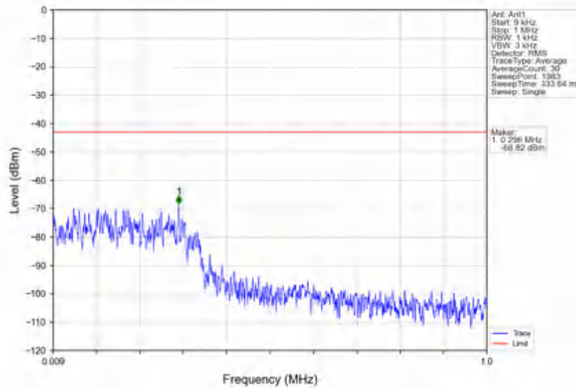
n78e_30kHz_SISO_NTV_30MHz_DFT-s-OFDM_QPSK_3465MHz_Edge_1RB_Left
