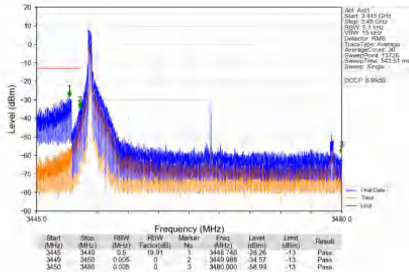
n78e_30kHz_SISO_NTV_30MHz_CP-OFDM QPSK_3465MHz_Edge_1RB_Left
