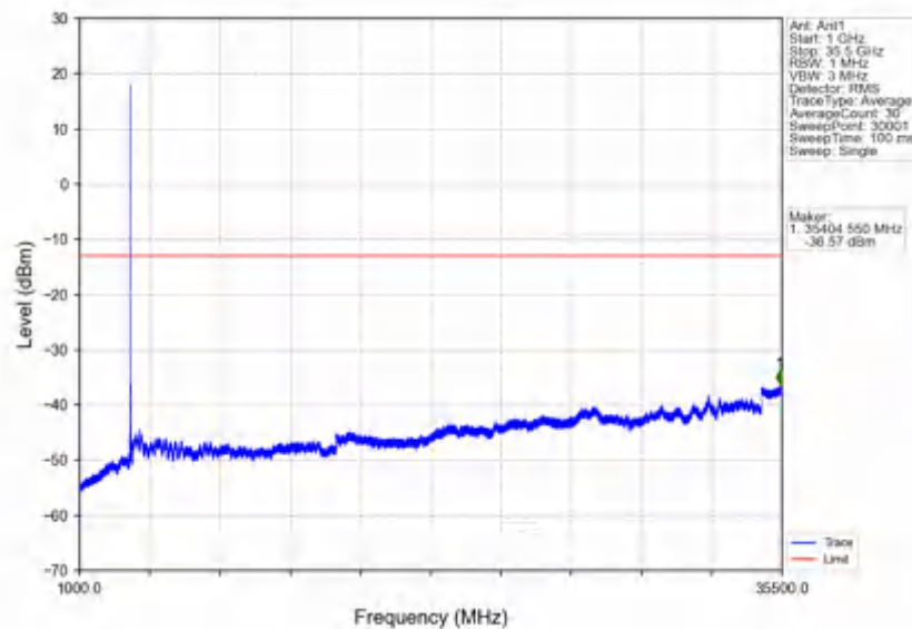
n78e_30kHz_SISO_NTNV_30MHz_DFT-s-OFDM QPSK_3534.99MHz_Edge_1RB_Right
