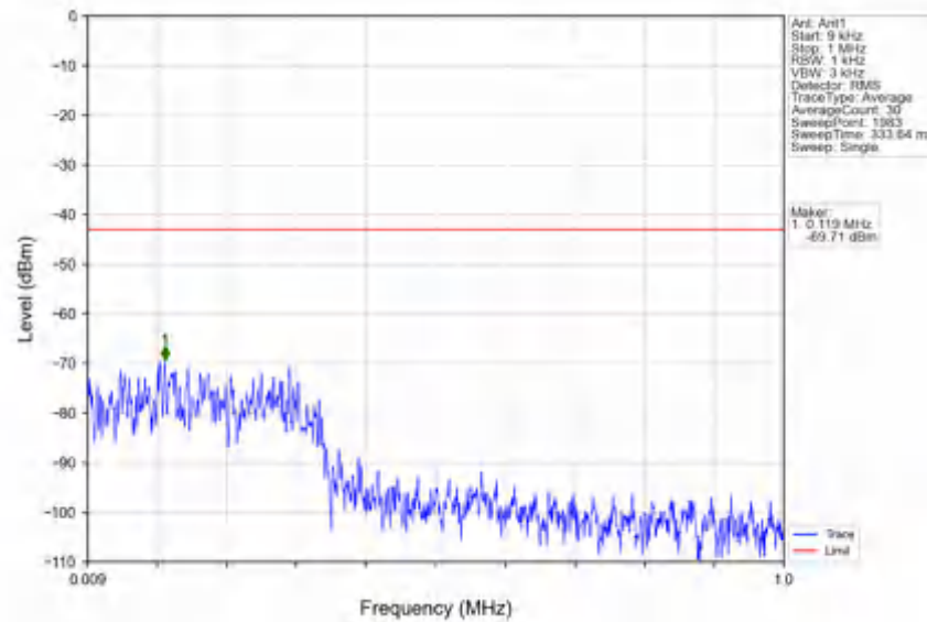
n78e_30kHz_SISO_NTNV_20MHz_DFT-s-OFDM QPSK_3540MHz_Edge_1RB_Right
