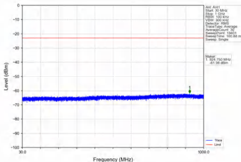
n78e_30kHz_SISO_NTNV_30MHz_DFT-s-OFDM_PI/2_BPSK_3465MHz_Outer_Full
