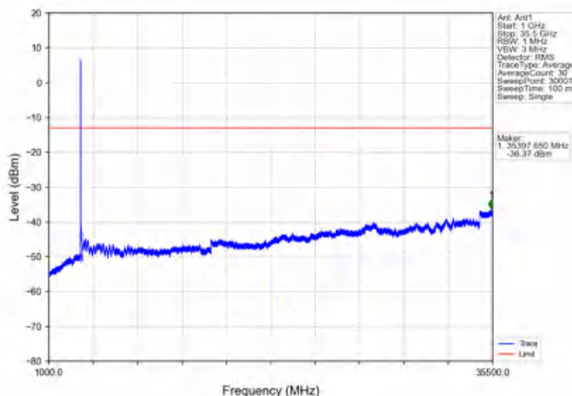
n78e_30kHz_SISO_NTNV_30MHz_DFT-s-OFDM_PI/2_BPSK_3465MHz_Outer_Full
