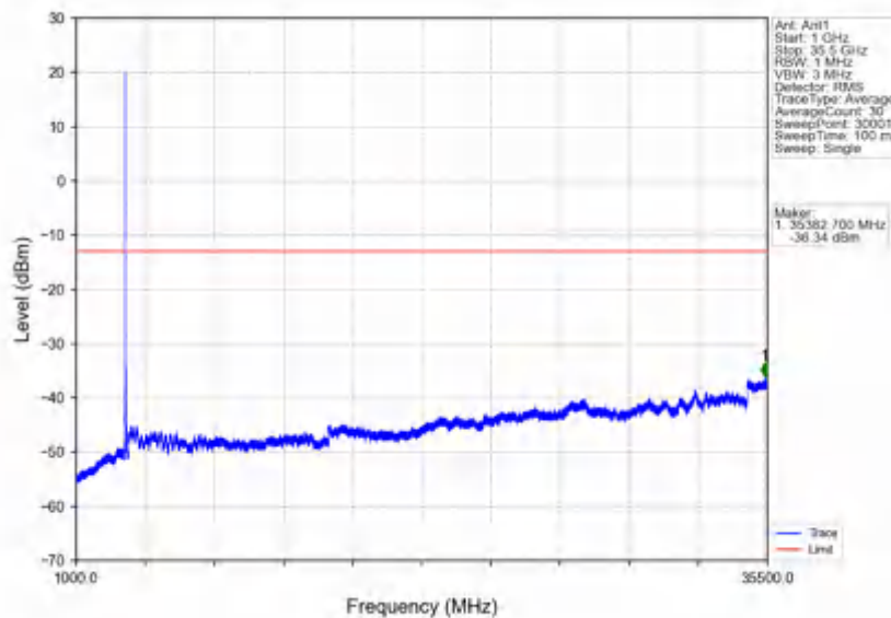
n78e_30kHz_SISO_NTNV_30MHz_CP-OFDM QPSK_3465MHz_Outer_Full
