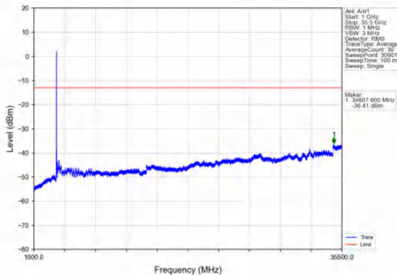
n78e_30kHz_SISO_NTNV_40MHz_DFT-s-OFDM_QPSK_3529.98MHz_Inner_1RB_Right
