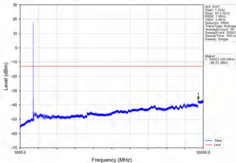
n78e_30kHz_SISO_NTV_30MHz_CP-OFDM QPSK_3500.01MHz_Edge_1RB_Left
