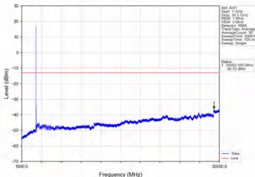
n78e_30kHz_SISO_NTV_40MHz_CP-OFDM QPSK_3500.01MHz_Edge_1RB_Left
