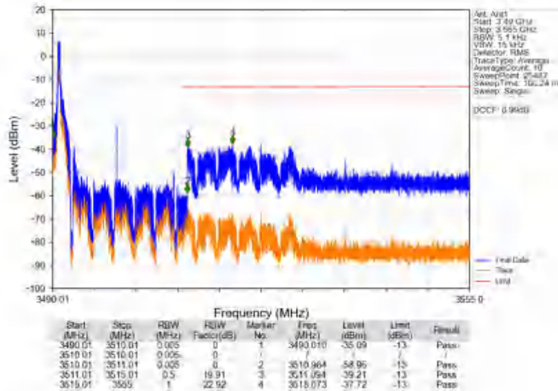
n78e_30kHz_SISO_NTV_20MHz_CP-OFDM QPSK_3500.01MHz_Edge_1RB_Left
