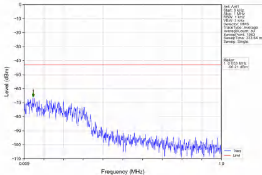
n78e_30kHz_SISO_NTNV_30MHz_CP-OFDM QPSK_3534.99MHz_Edge_1RB_Right
