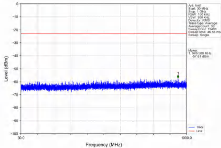
n78e_30kHz_SISO_NTNV_20MHz_DFT-s-OFDM QPSK_3540MHz_Edge_1RB_Right
