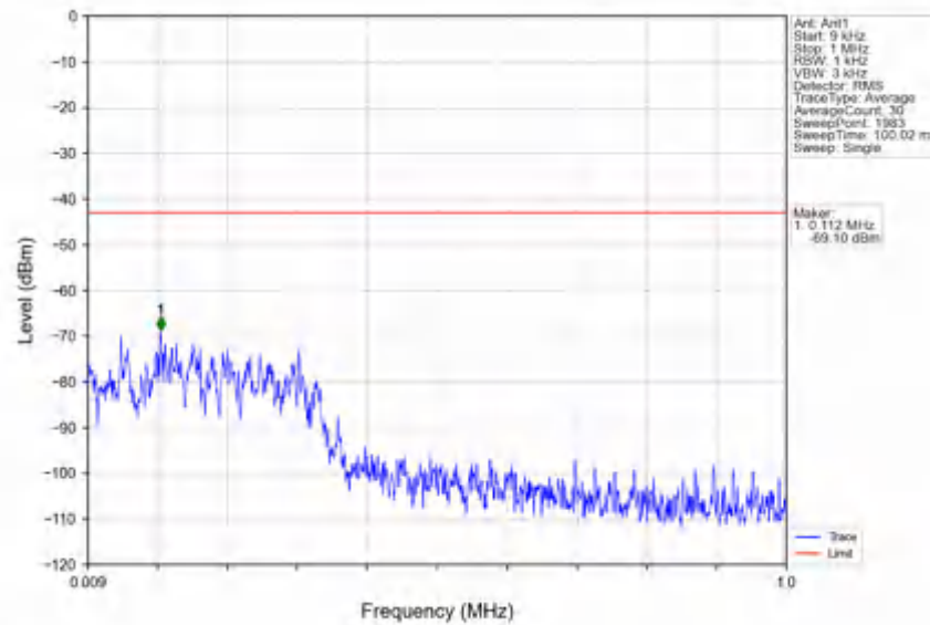
n78e_30kHz_SISO_NTNV_20MHz_DFT-s-OFDM QPSK_3540MHz_Inner_1RB_Right
