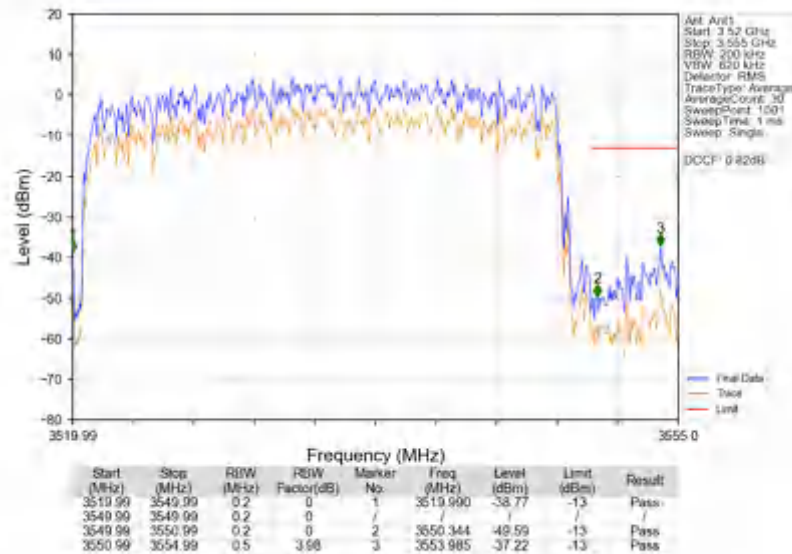
n78e_30kHz_SISO_NTNV_30MHz_DFT-s-OFDM_QPSK_3534.99MHz_Outer_Full
