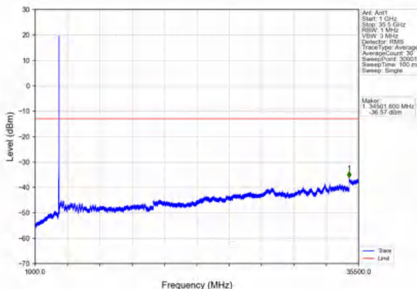
n78e_30kHz_SISO_NTNV_25MHz_DFT-s-OFDM QPSK_3537.48MHz_Inner_1RB_Right
