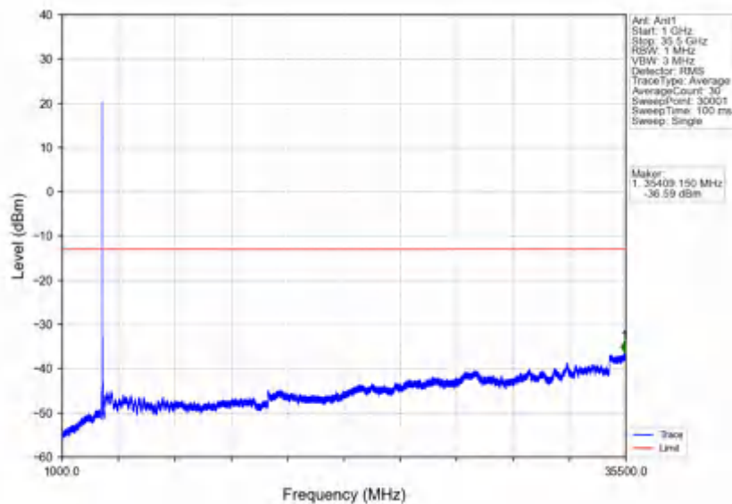
n78e_30kHz_SISO_NTV_25MHz_CP-OFDM QPSK_3462.51MHz_Outer_Full
