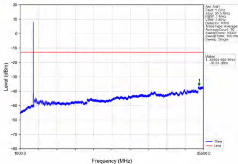
n78e_30kHz_SISO_NTNV_25MHz_DFT-s-OFDM_QPSK_3462.51MHz_Inner_1RB_Left
