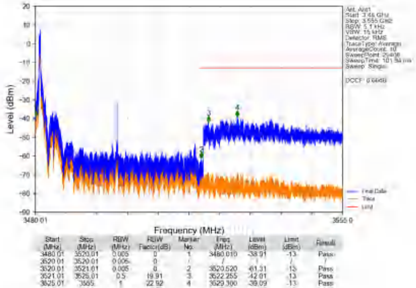
n78e_30kHz_SISO_NTV_40MHz_CP-OFDM QPSK_3500.01MHz_Edge_1RB_Left
