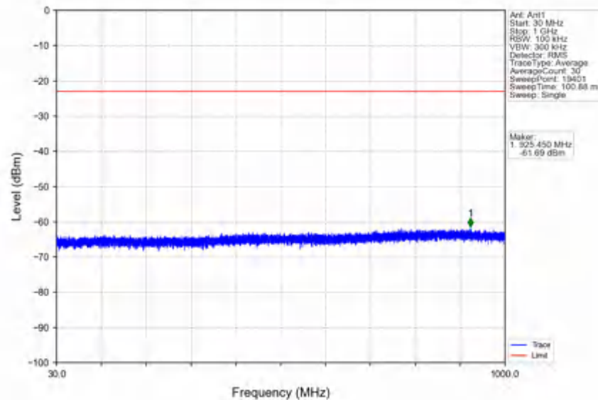
n78e_30kHz_SISO_NTNV_30MHz_DFT-s-OFDM_QPSK_3465MHz_Outer_Full
