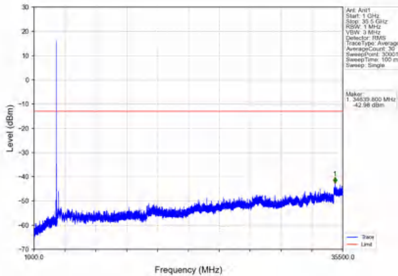
n78e_30kHz_SISO_NTNV_20MHz_DFT-s-OFDM QPSK_3540MHz_Edge_1RB_Right
