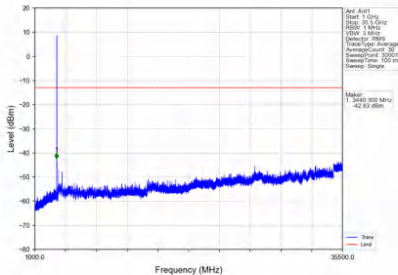
n78e_30kHz_SISO_NTNV_20MHz_DFT-s-OFDM_QPSK_3460.02MHz_Inner_1RB_Left
