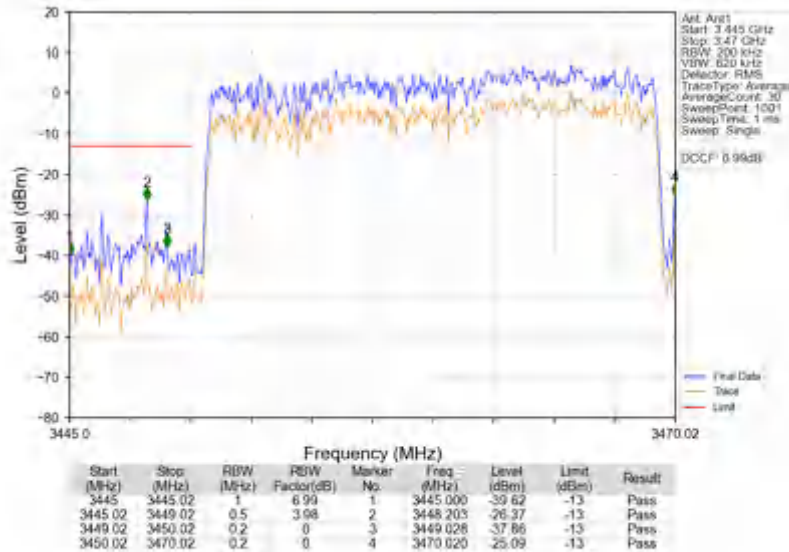
n78e_30kHz_SISO_NTV_20MHz_CP-OFDM QPSK_3460.02MHz_Outer_Full
