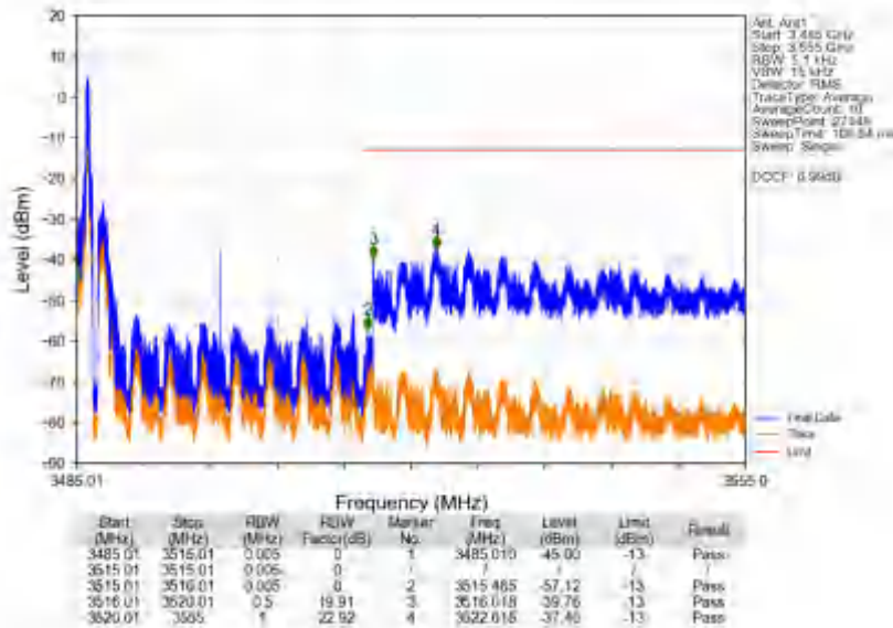
n78e_30kHz_SISO_NTV_30MHz_CP-OFDM QPSK_3500.01MHz_Edge_1RB_Left
