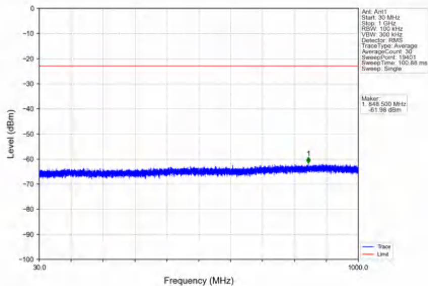
n78e_30kHz_SISO_NTNV_30MHz_CP-OFDM_QPSK_3465MHz_Outer_Full
