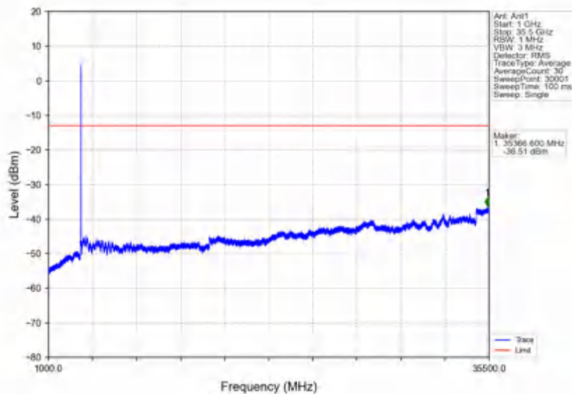
n78e_30kHz_SISO_NTNV_30MHz_DFT-s-OFDM_QPSK_3534.99MHz_Inner_1RB_Right
