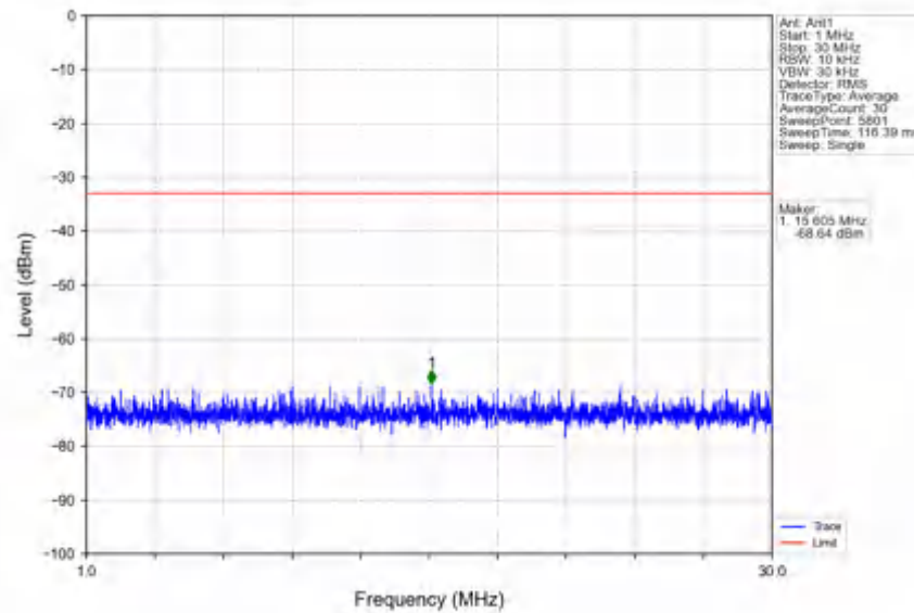
n78e_30kHz_SISO_NTNV_30MHz_DFT-s-OFDM_QPSK_3500.01MHz_Edge_1RB_Left
