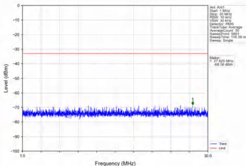
n78e_30kHz_SISO_NTNV_40MHz_CP-OFDM QPSK_3529.98MHz_Edge_1RB_Right
