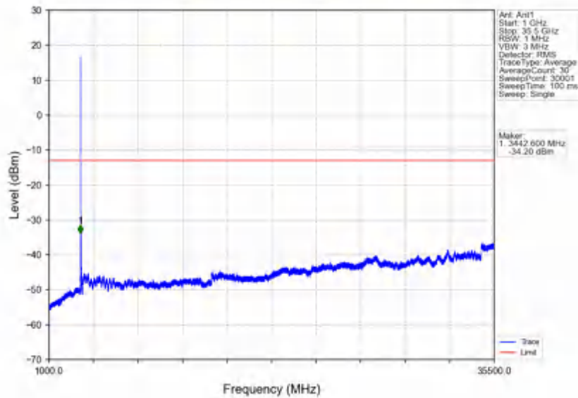
n78e_30kHz_SISO_NTV_40MHz_CP-OFDM QPSK_3500.01MHz_Edge_1RB_Left
