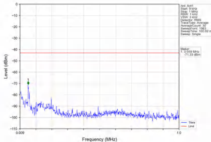
n78e_30kHz_SISO_NTNV_25MHz_DFT-s-OFDM_QPSK_3462.51MHz_Outer_Full
