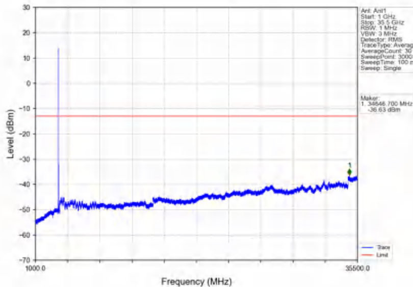
n78e_30kHz_SISO_NTV_30MHz_DFT-s-OFDM QPSK_3465MHz_Edge_1RB_Left
