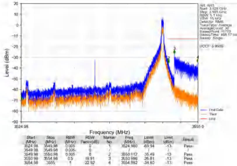
n78e_30kHz_SISO_NTNV_25MHz_CP-OFDM QPSK_3537.48MHz_Edge_1RB_Right
