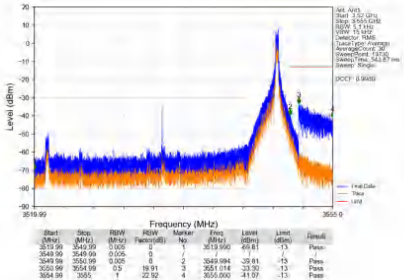
n78e_30kHz_SISO_NTNV_30MHz_DFT-s-OFDM_QPSK_3534.99MHz_Inner_1RB_Right
