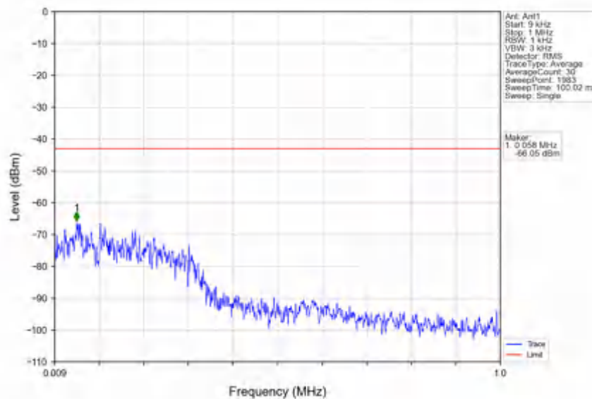
n78e_30kHz_SISO_NTV_40MHz_CP-OFDM_QPSK_3470.01MHz_Inner_1RB_Left
