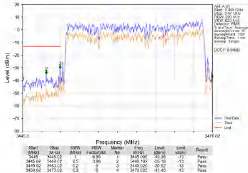
n78e_30kHz_SISO_NTNV_20MHz_DFT-s-OFDM_QPSK_3460.02MHz_Outer_Full
