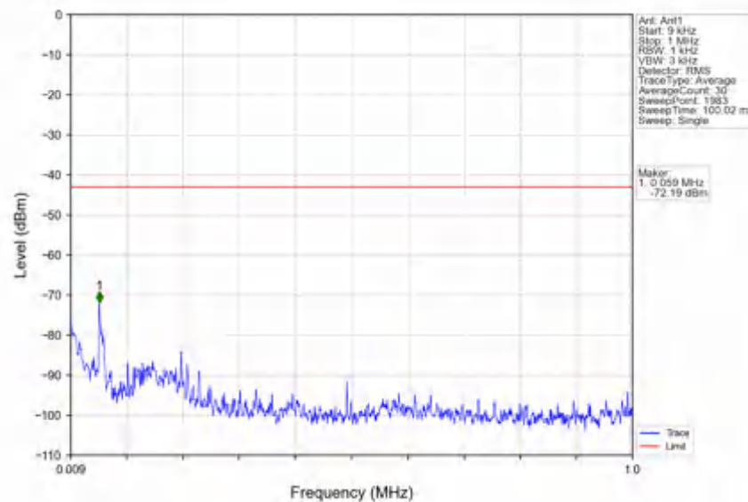
n78e_30kHz_SISO_NTNV_30MHz_DFT-s-OFDM_QPSK_3534.99MHz_Outer_Full
