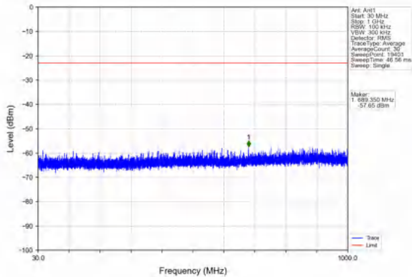
n78e_30kHz_SISO_NTV_25MHz_CP-OFDM_QPSK_3500.01MHz_Edge_1RB_Left
