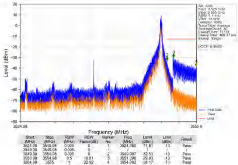
n78e_30kHz_SISO_NTNV_25MHz_DFT-s-OFDM_QPSK_3537.48MHz_Edge_1RB_Right
