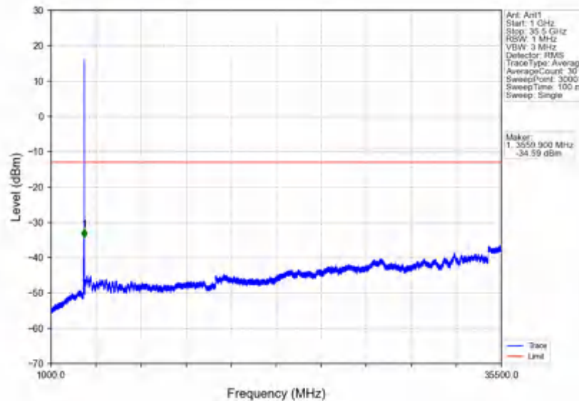
n78e_30kHz_SISO_NTNV_40MHz_DFT-s-OFDM QPSK_3529.98MHz_Inner_1RB_Right
