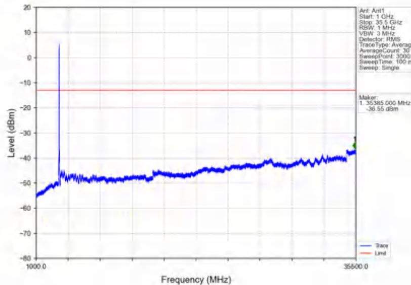
n78e_30kHz_SISO_NTNV_40MHz_CP-OFDM QPSK_3470.01MHz_Outer_Full
