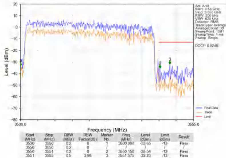
n78e_30kHz_SISO_NTNV_20MHz_CP-OFDM QPSK_3540MHz_Outer_Full
