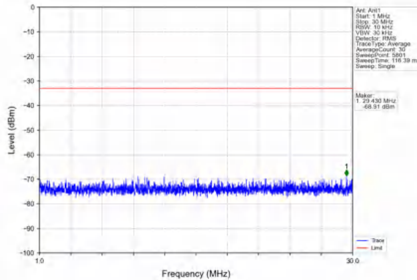
n78e_30kHz_SISO_NTV_30MHz_CP-OFDM QPSK_3465MHz_Edge_1RB_Left
