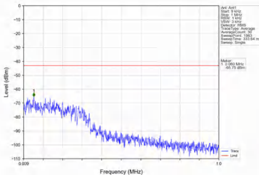
n78e_30kHz_SISO_NTV_30MHz_CP-OFDM QPSK_3465MHz_Edge_1RB_Left
