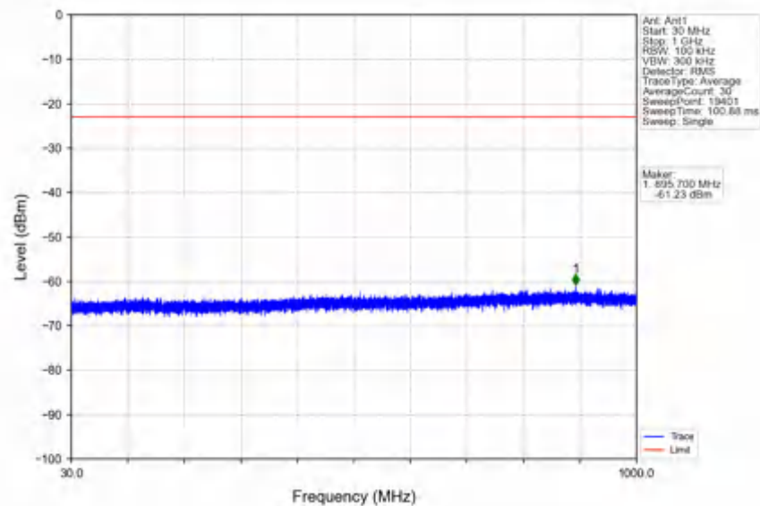
n78e_30kHz_SISO_NTNV_40MHz_CP-OFDM_QPSK_3529.98MHz_Outer_Full
