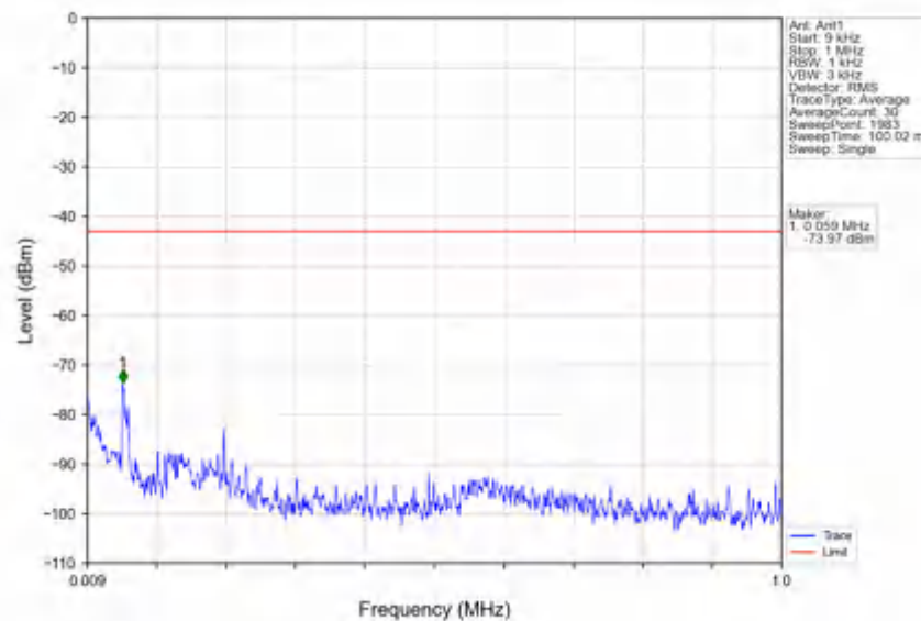
n78e_30kHz_SISO_NTNV_25MHz_DFT-s-OFDM_QPSK_3537.48MHz_Outer_Full
