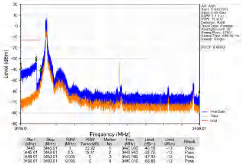
n78e_30kHz_SISO_NTNV_40MHz_DFT-s-OFDM_QPSK_3470.01MHz_Inner_1RB_Left
