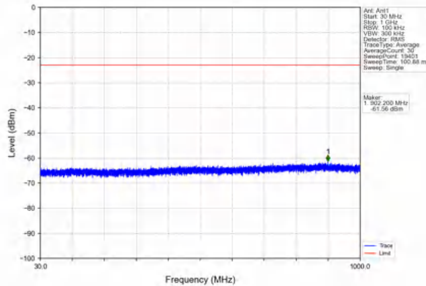
n78e_30kHz_SISO_NTNV_30MHz_DFT-s-OFDM QPSK_3534.99MHz_Inner_1RB_Right
