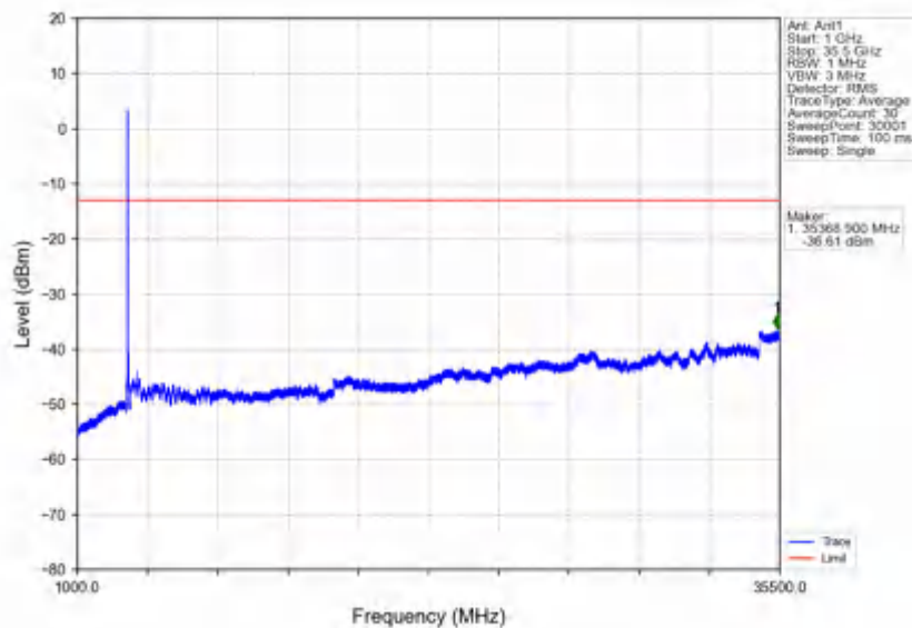
n78e_30kHz_SISO_NTNV_40MHz_DFT-s-OFDM_QPSK_3470.01MHz_Inner_1RB_Left
