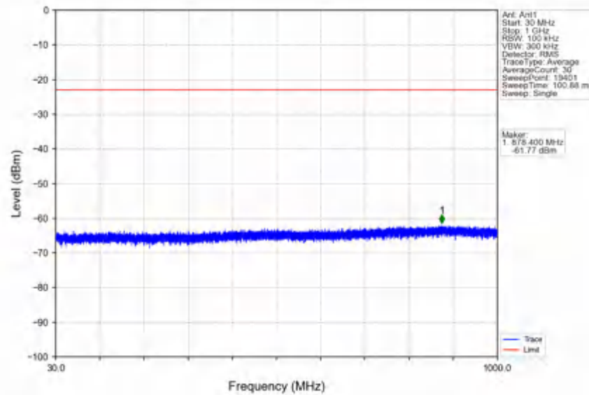
n78e_30kHz_SISO_NTNV_25MHz_CP-OFDM QPSK_3537.48MHz_Outer_Full
