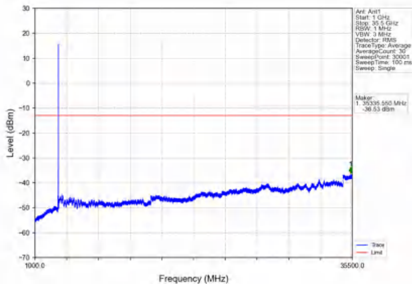
n78e_30kHz_SISO_NTNV_25MHz_CP-OFDM QPSK_3537.48MHz_Outer_Full
