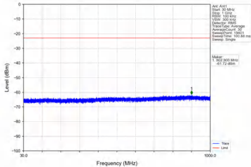
n78e_30kHz_SISO_NTNV_40MHz_CP-OFDM QPSK_3470.01MHz_Outer_Full
