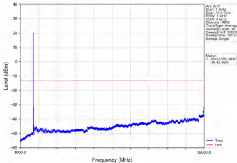
n78e_30kHz_SISO_NTV_25MHz_CP-OFDM_QPSK_3500.01MHz_Edge_1RB_Left
