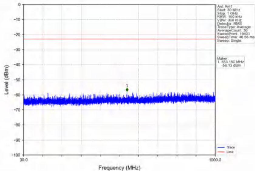
n78e_30kHz_SISO_NTV_30MHz_CP-OFDM_QPSK_3500.01MHz_Edge_1RB_Left
