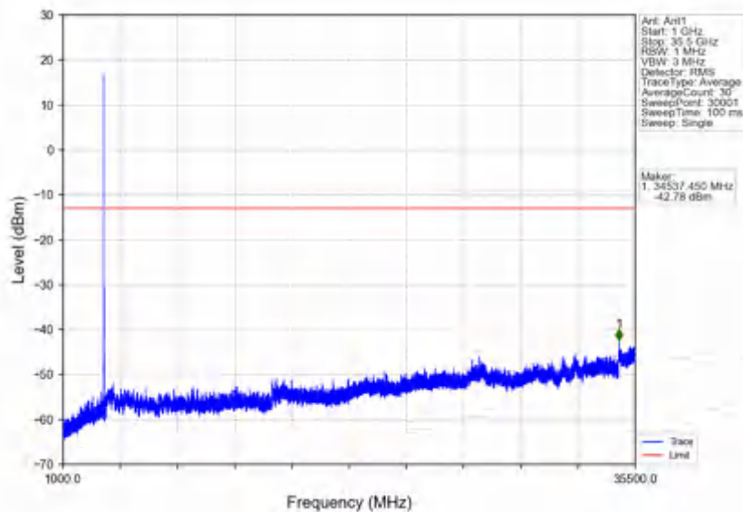
n78e_30kHz_SISO_NTV_20MHz_CP-OFDM QPSK_3500.01MHz_Edge_1RB_Left
