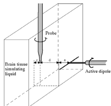
Figure 2. Spherical isotropy jig showing probe, dipole and box filled with simulated brain liquid (see Ref [2], Section A.5.2.1)
