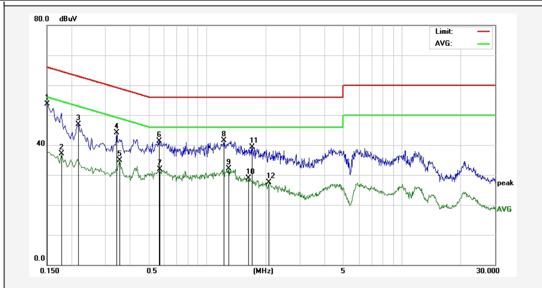
TM1 / Line: Neutral / Band: 5150-5250 MHz / BW: 20 / CH: H
