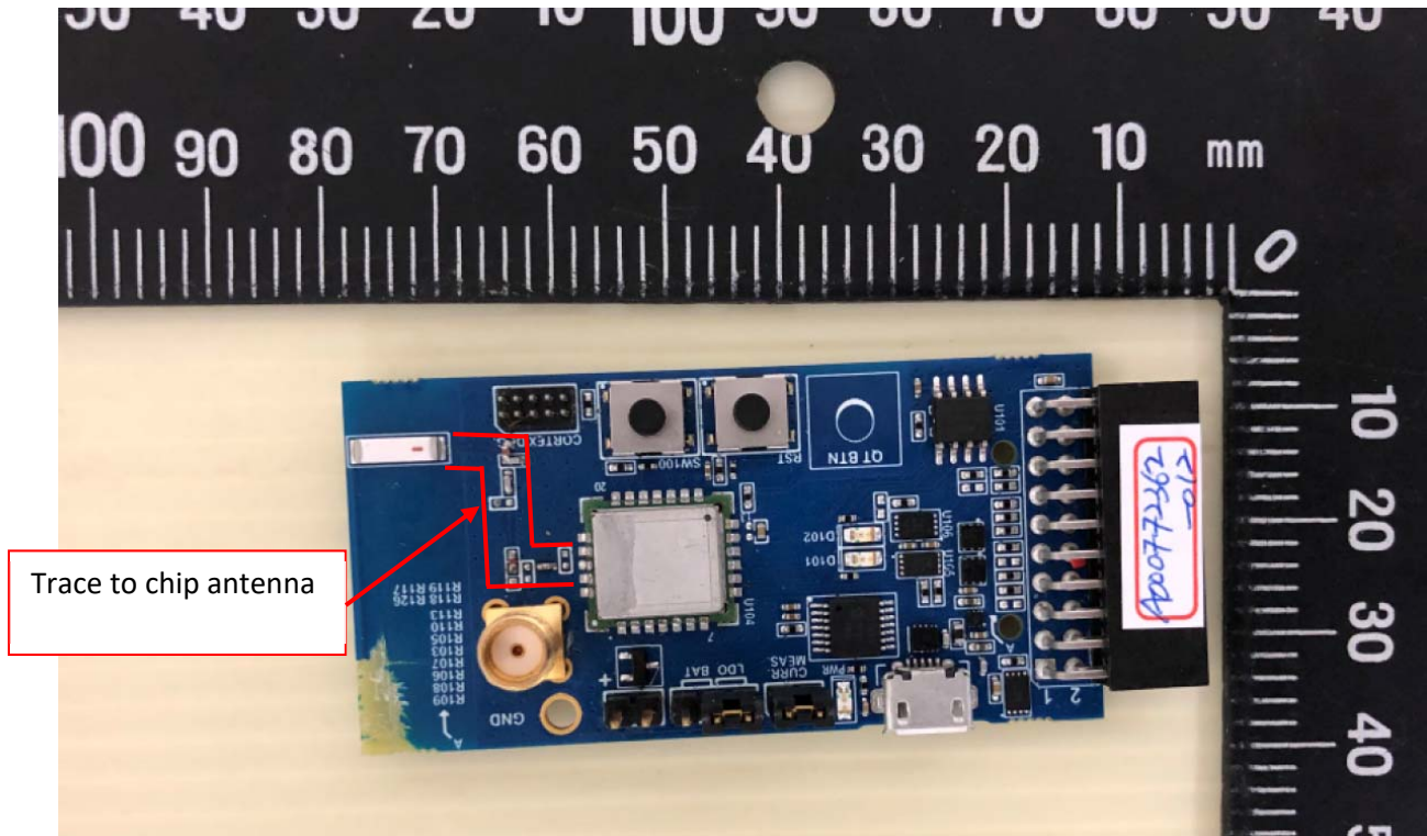
Module with Chip antenna(0900AT43A0070)
