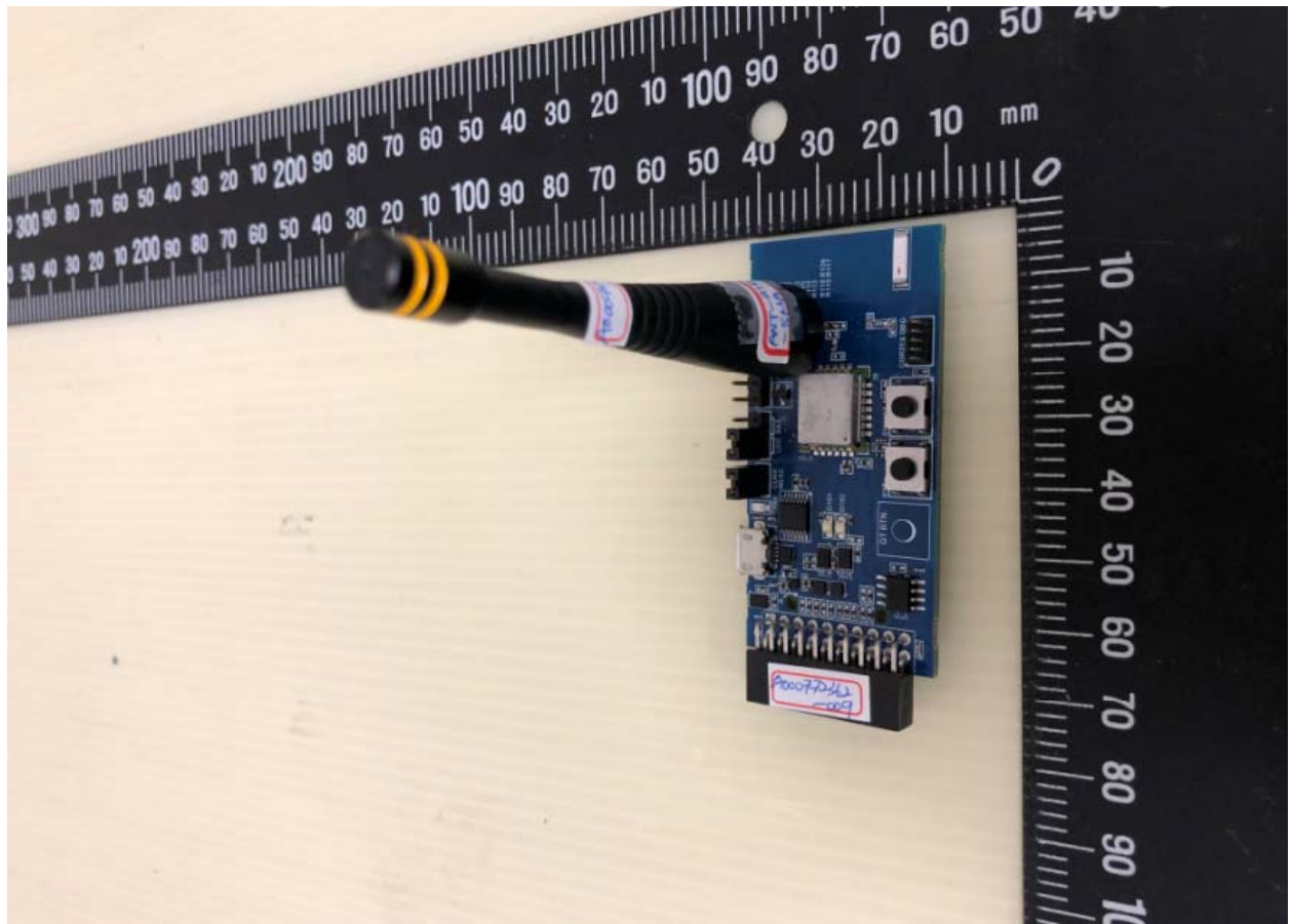
External antenna (ANT-916-CW-QW-SMA) Mounted on RF connector
