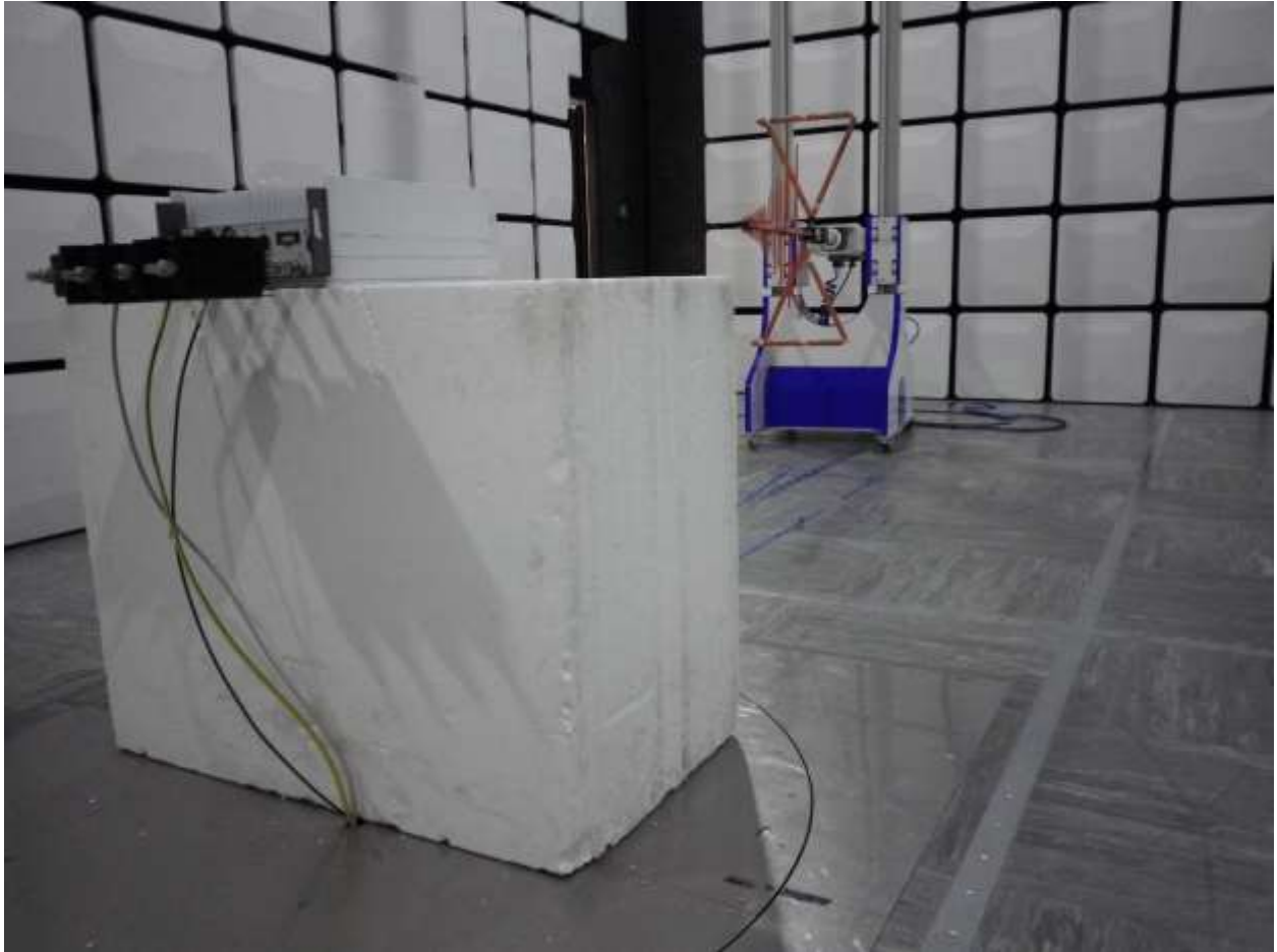
Radiated 30 MHz – 1GHz Testing
