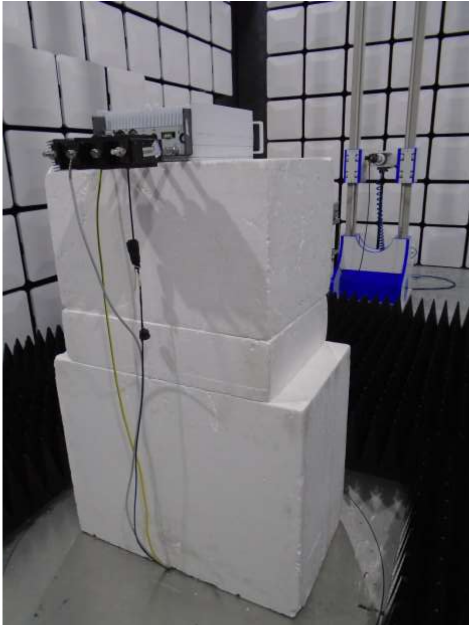
Radiated 18GHz – 22GHz Testing
