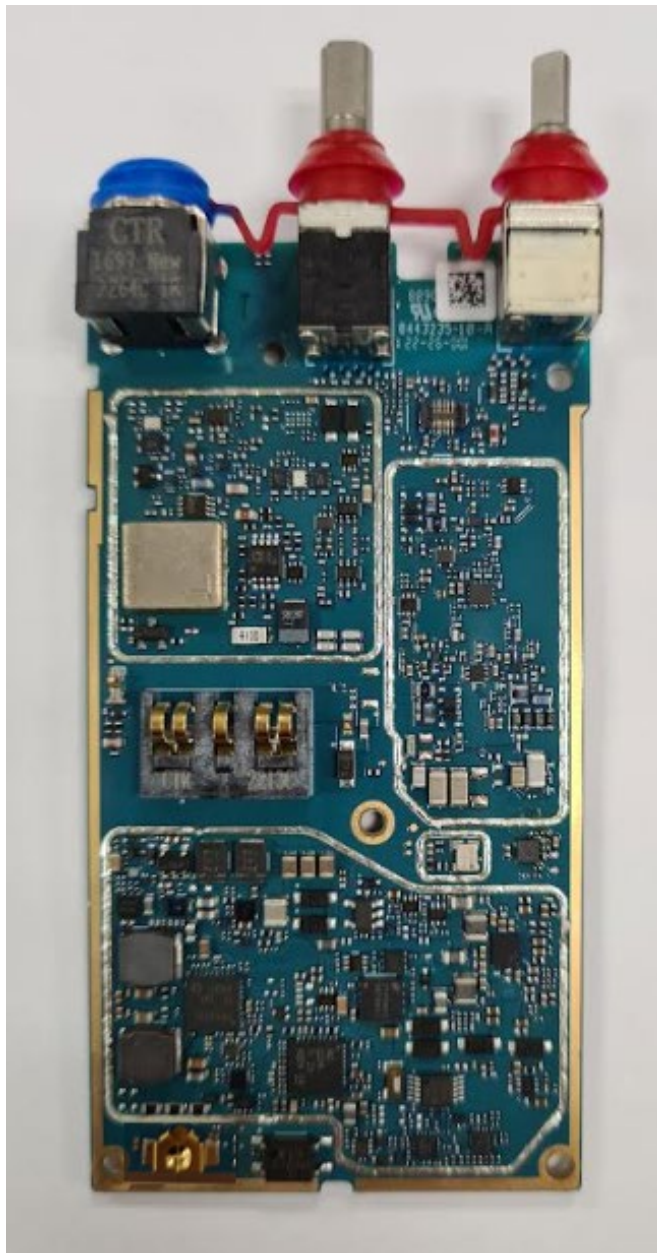
RF board without Shields (Bottom) of TIA FKP Model
