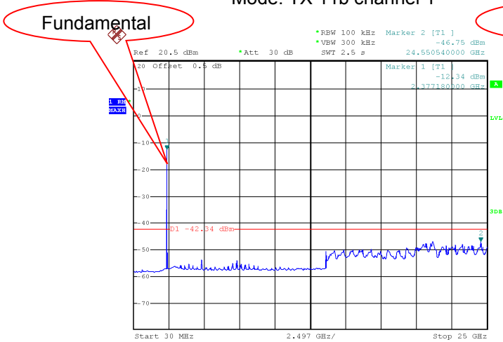
Mode: TX 11b channel 1
