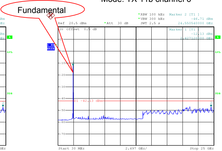
Mode: TX 11b channel 6
