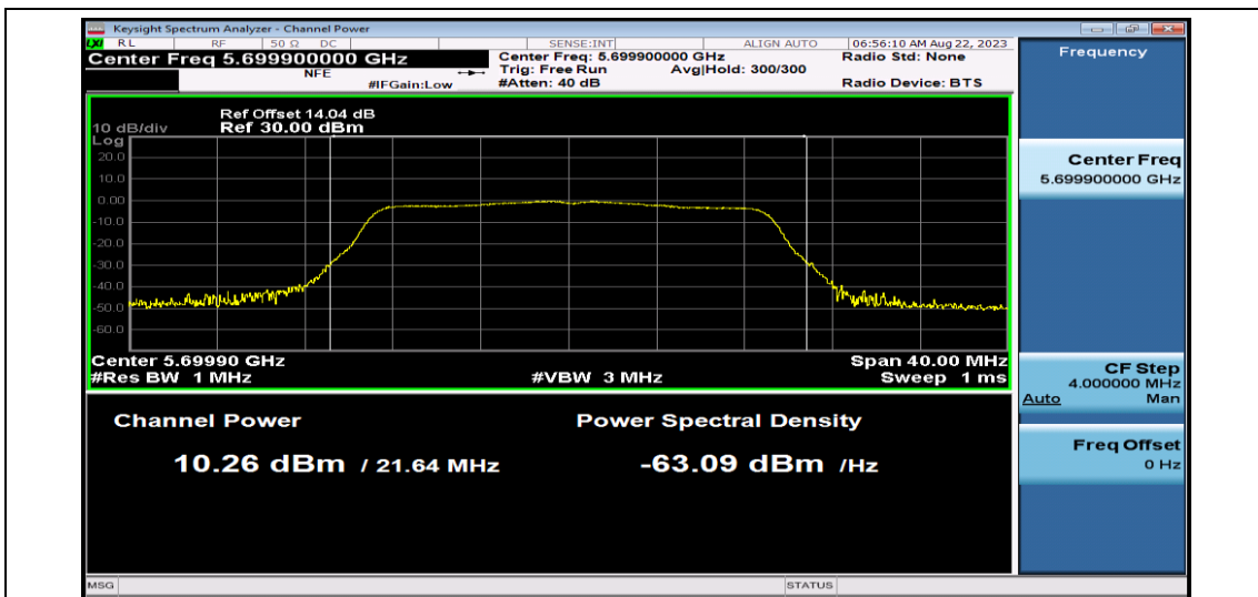
11AC20SISO-Ant1-5700
