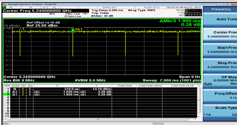
NTNV-11AC20SISO-Ant1-5240
