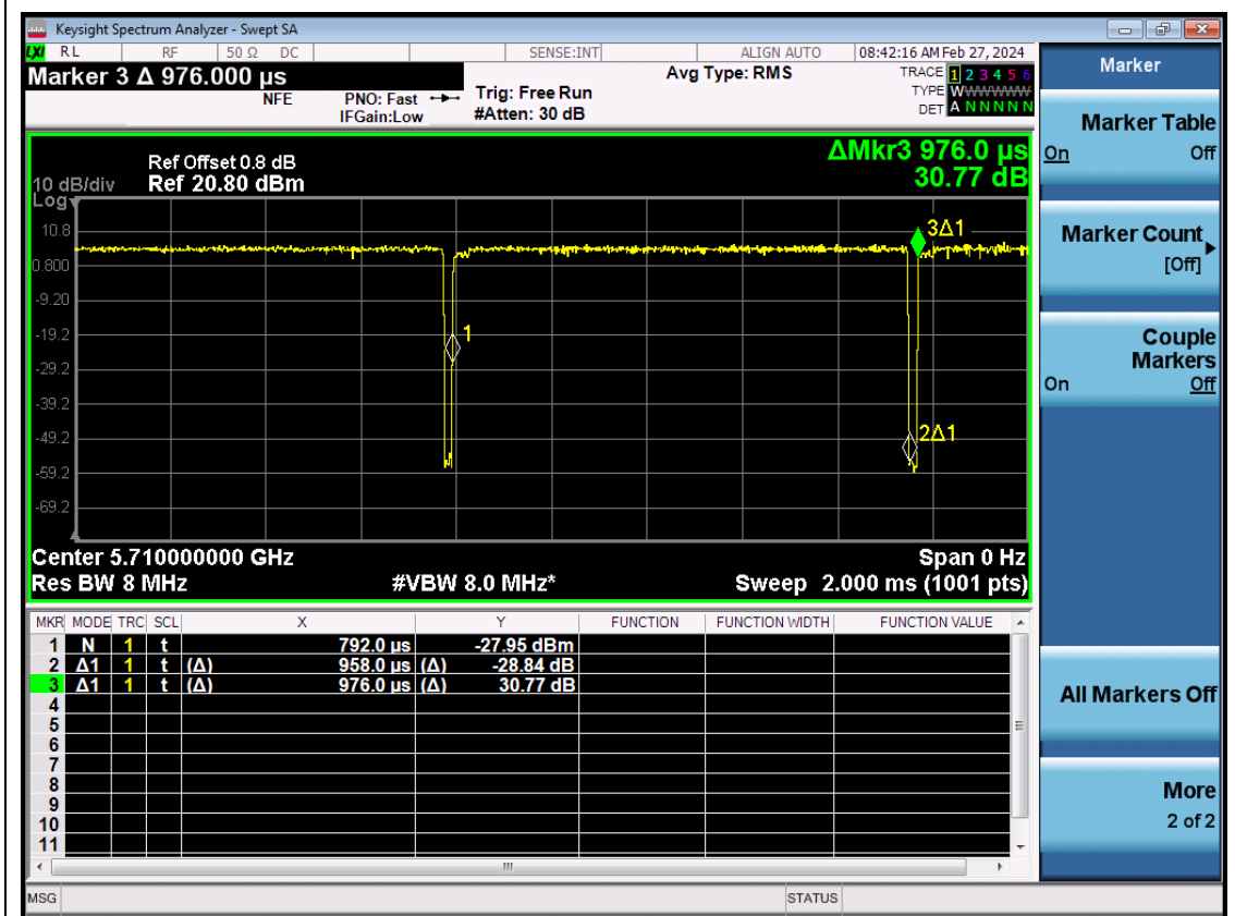
NTNV-11AC40SISO-Ant1-5710
