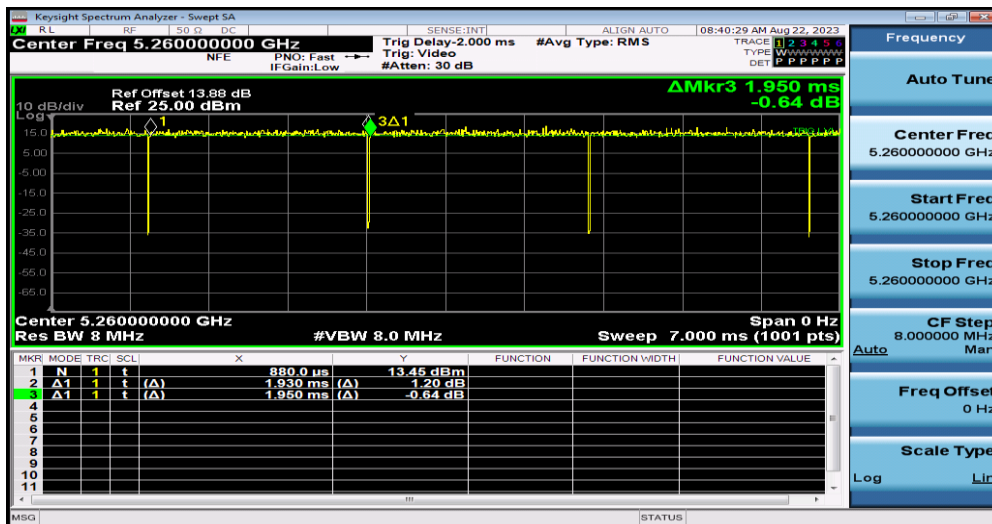
NTNV-11AC20SISO-Ant1-5260
