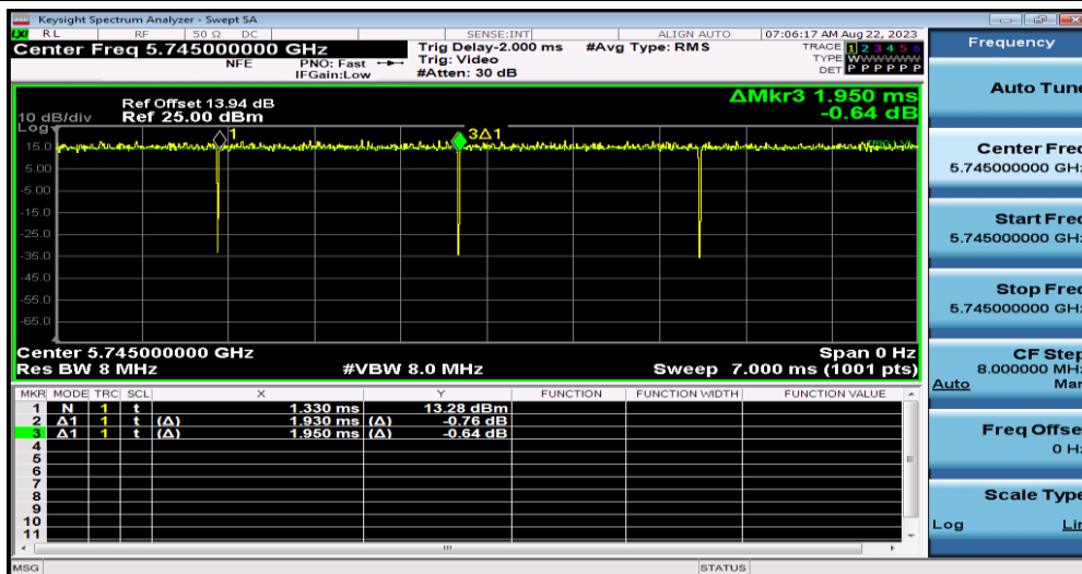
NTNV-11AC20SISO-Ant1-5745
