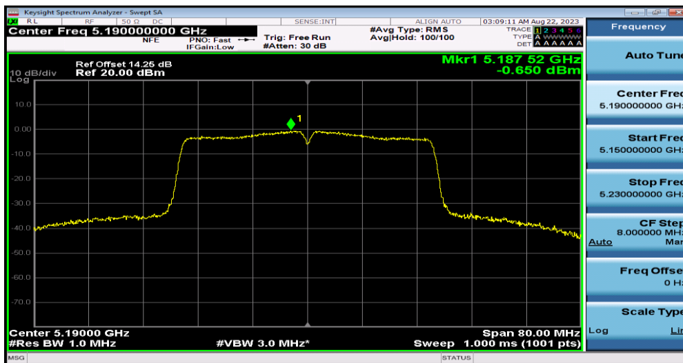
11AC40SISO-Ant1-5190
