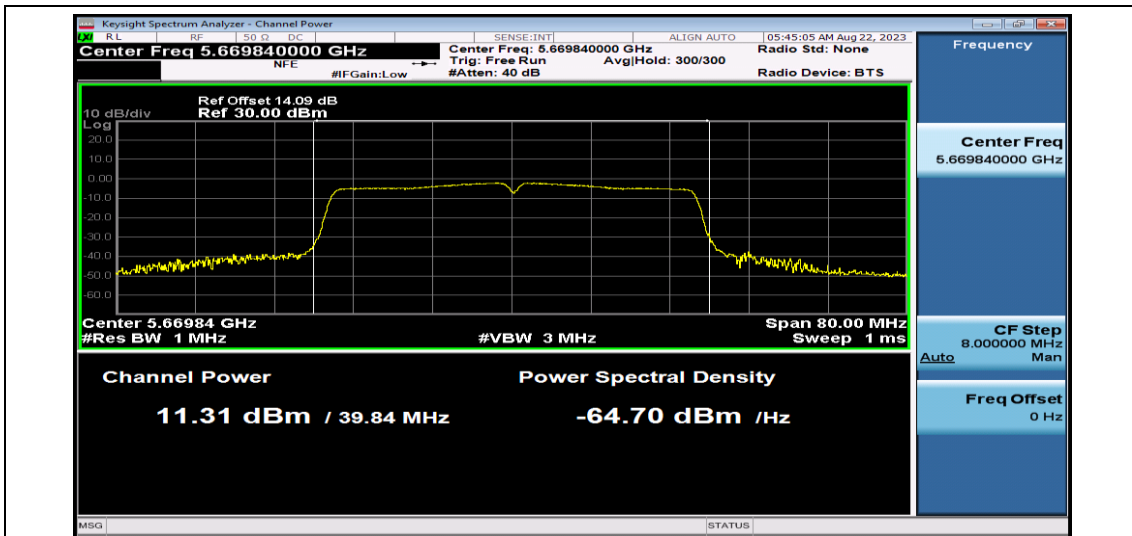
11AC40SISO-Ant1-5670
