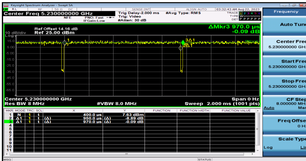
NTNV-11AC40SISO-Ant1-5230
