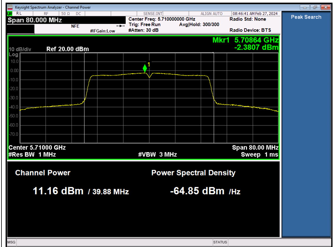
11AC40SISO-Ant1-5710
