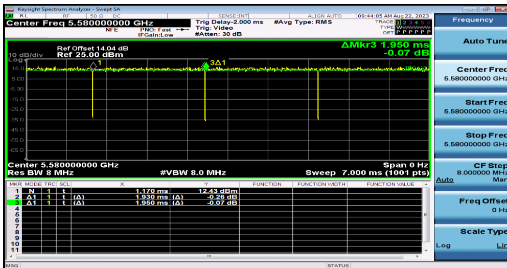
NTNV-11AC20SISO-Ant1-5580
