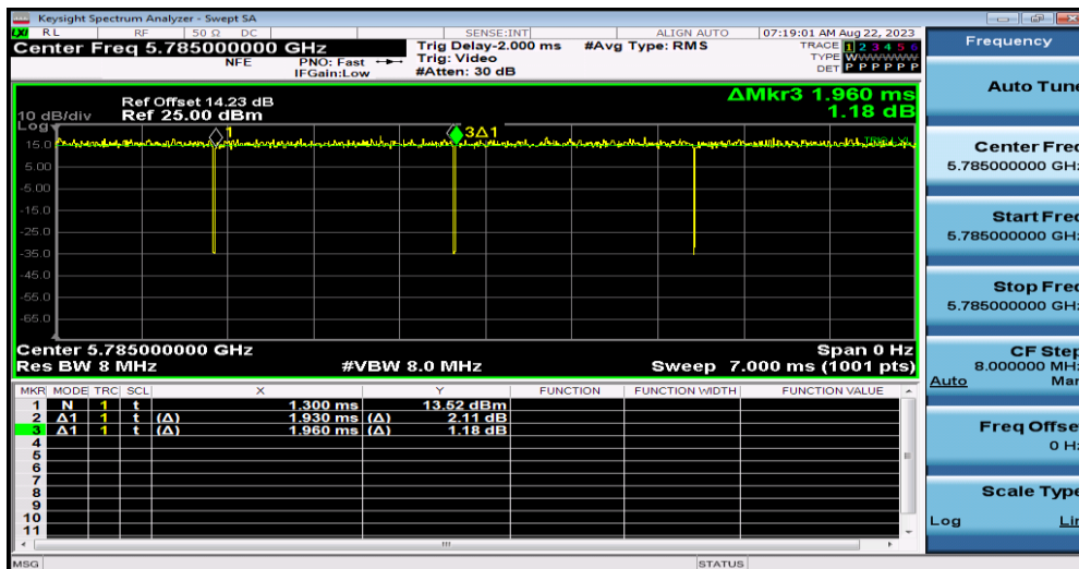
NTNV-11AC20SISO-Ant1-5785
