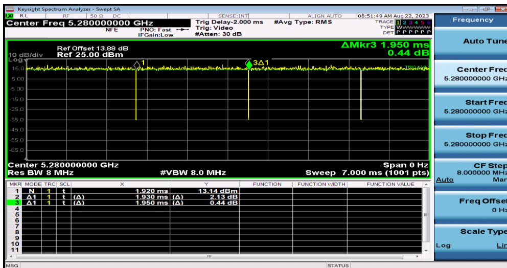
NTNV-11AC20SISO-Ant1-5280
