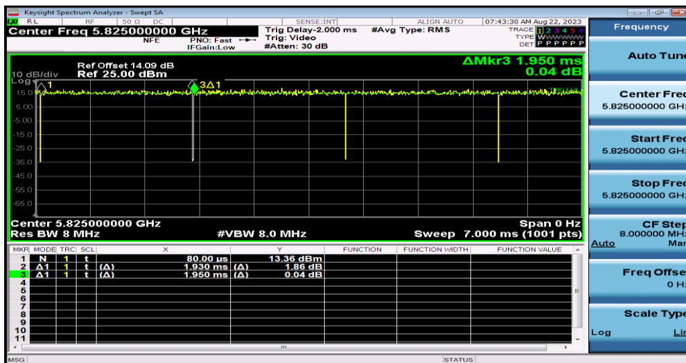
NTNV-11AC20SISO-Ant1-5825
