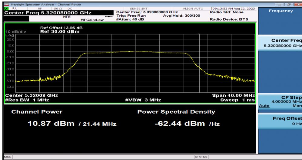
11AC20SISO-Ant1-5320
