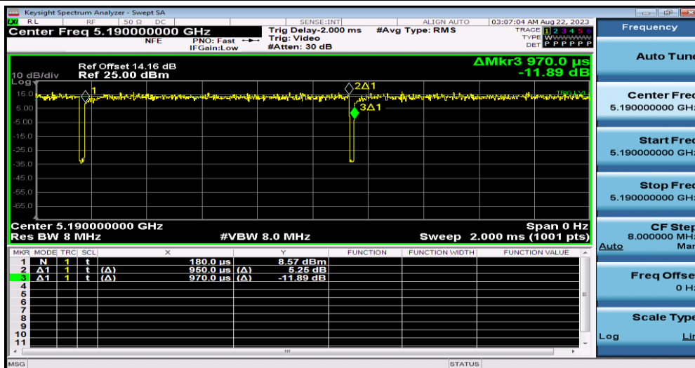
NTNV-11AC40SISO-Ant1-5190
