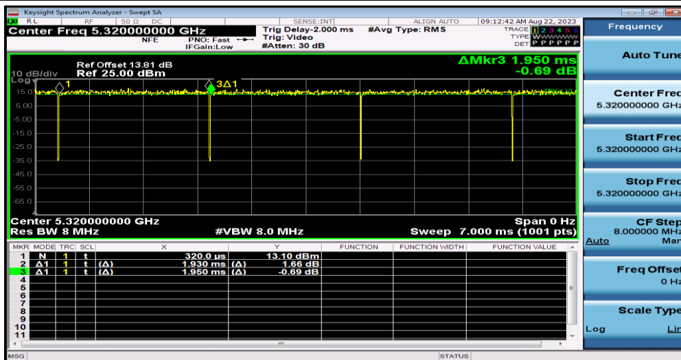
NTNV-11AC20SISO-Ant1-5320
