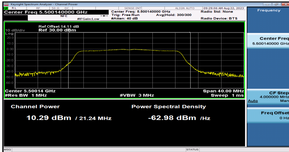
11AC20SISO-Ant1-5500
