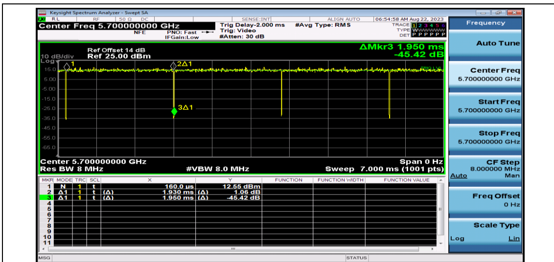
NTNV-11AC20SISO-Ant1-5700
