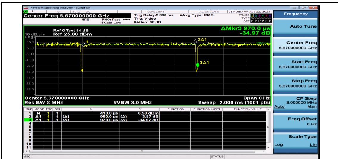
NTNV-11AC40SISO-Ant1-5670
