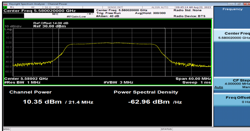
11AC20SISO-Ant1-5580
