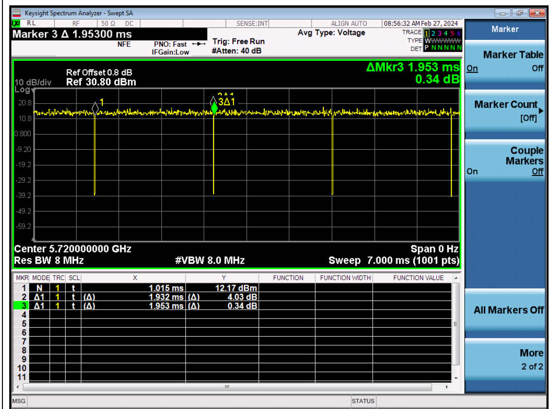
NTNV-11AC20SISO-Ant1-5720
