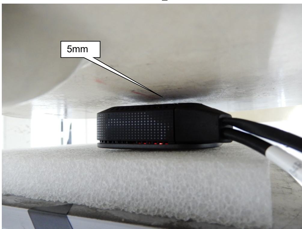
EUT Back_5mm
