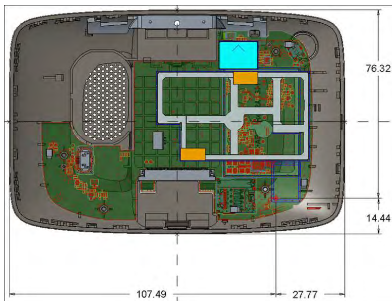
Fig.11 antenna location
