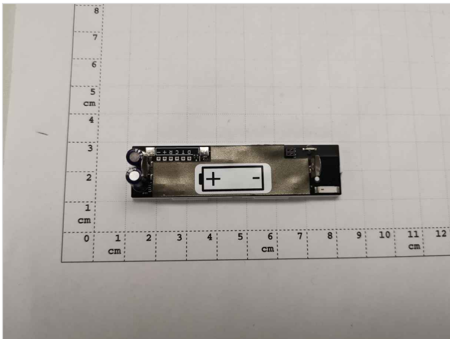
Photograph 4: EUT Inside view (battery removed)
