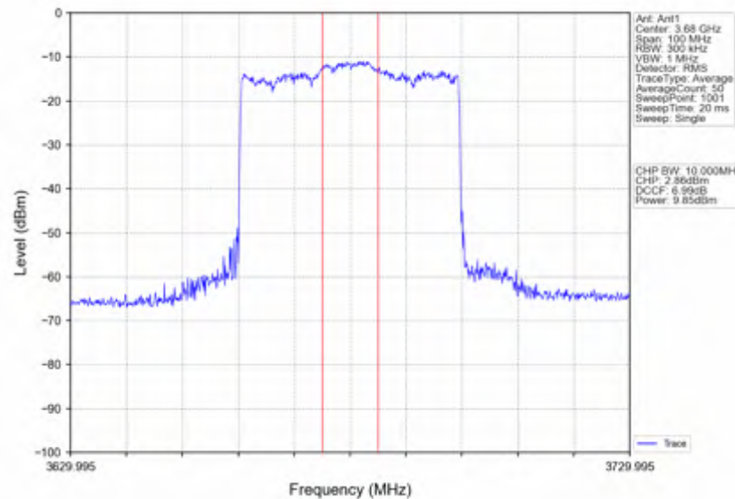
n78d_15kHz_SISO_NTNV_40MHz_CP-OFDM QPSK_3679.995MHz_Inner_Full
