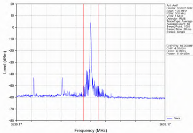
n78d_15kHz_SISO_NTNV_40MHz_DFT-s-OFDM_16_QAM_3570MHz_Inner_1RB_Right
