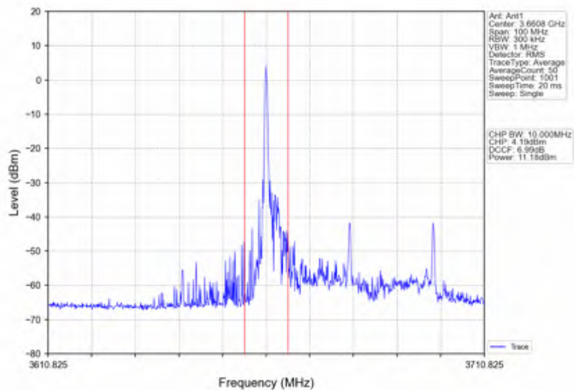
n78d_15kHz_SISO_NTNV_40MHz_CP-OFDM QPSK_3679.995MHz_Inner_1RB_Right
