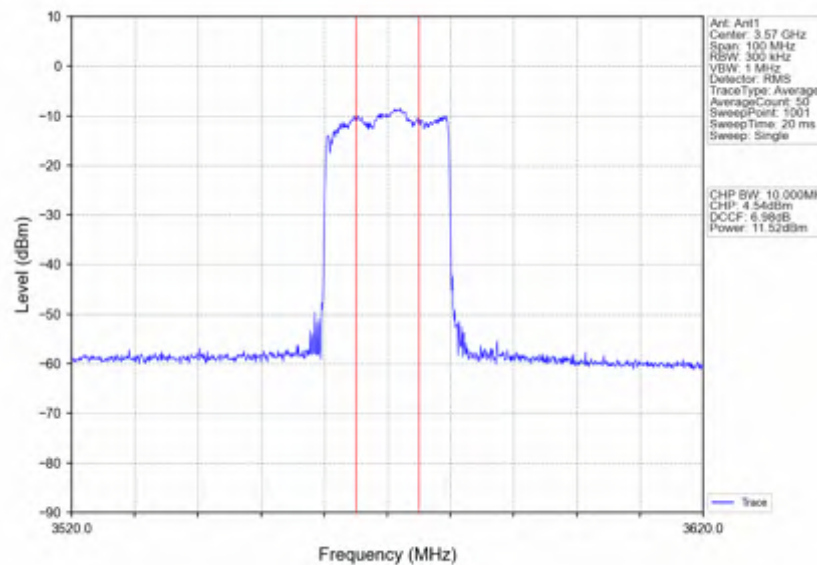
n78d_15kHz_SISO_NTNV_40MHz_CP-OFDM 16 QAM_3570MHz_Inner_Full
