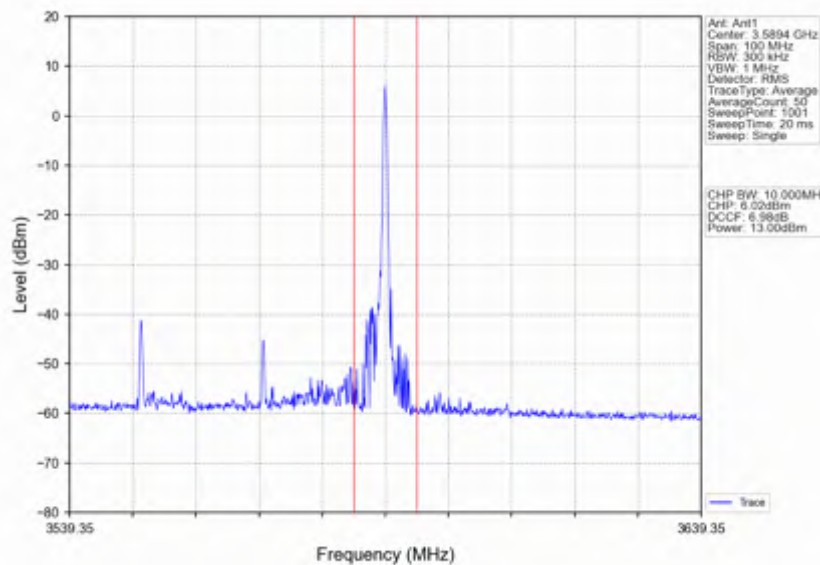
n78d_15kHz_SISO_NTNV_40MHz_CP-OFDM 256 QAM_3570MHz_Edge_1RB_Right
