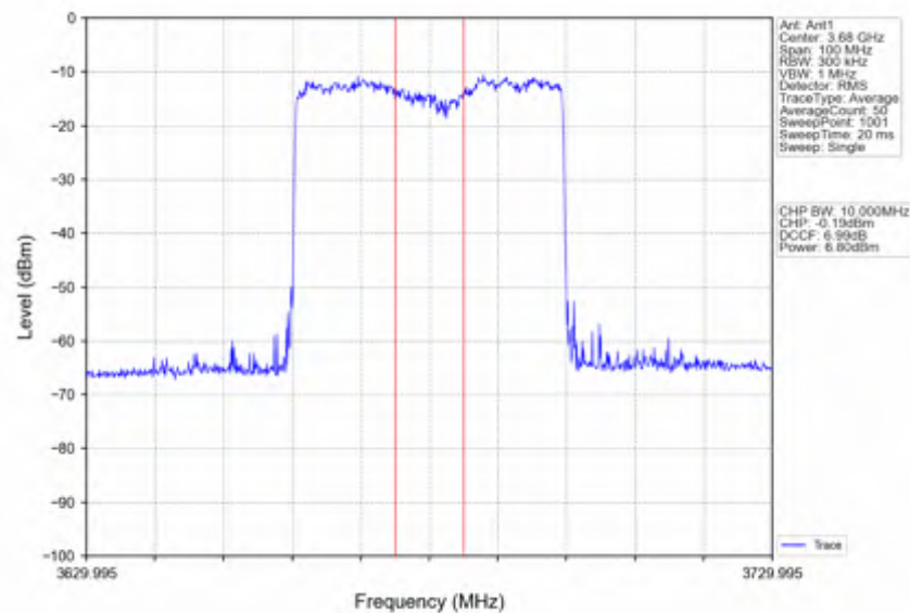
n78d_15kHz_SISO_NTNV_40MHz_DFT-s-OFDM_16_QAM_3679.995MHz_Inner_Full
