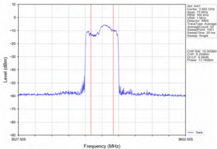
n78d_15kHz_SISO_NTNV_30MHz_CP-OFDM 64 QAM_3565.005MHz_Inner_Full
