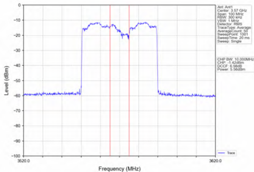
n78d_15kHz_SISO_NTNV_40MHz_CP-OFDM 16 QAM_3570MHz_Inner_Full
