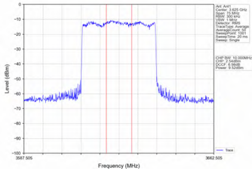
n78d_15kHz_SISO_NTNV_30MHz_DFT-s-OFDM QPSK_3625.005MHz_Inner_Full
