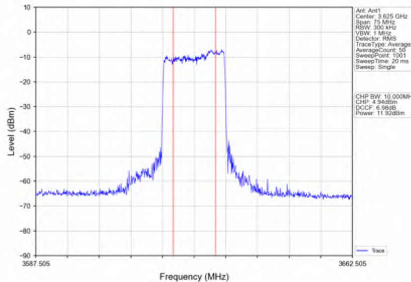
n78d_15kHz_SISO_NTNV_30MHz_DFT-s-OFDM QPSK_3625.005MHz_Inner_Full
