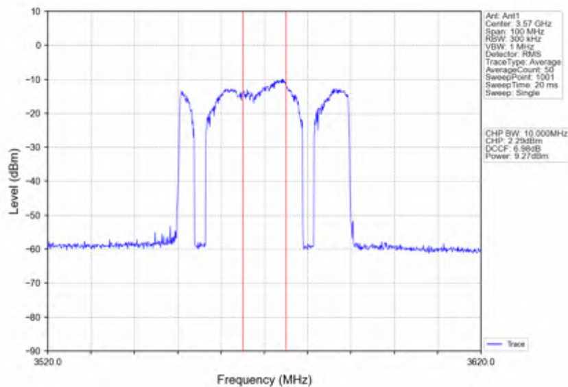
n78d_15kHz_SISO_NTNV_40MHz_DFT-s-OFDM 64 QAM_3570MHz_Inner_Full
