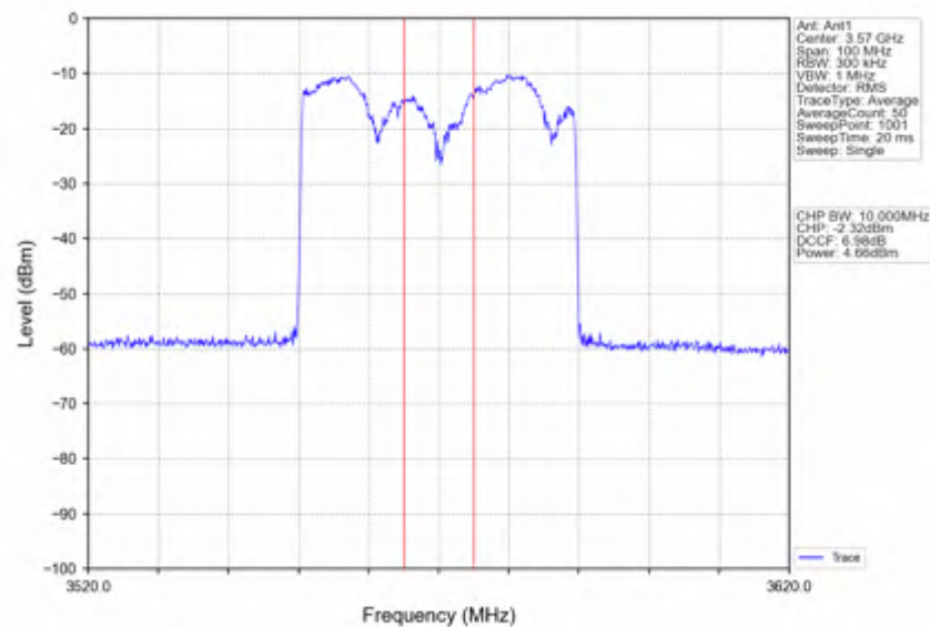
n78d 15kHz SISO NTNv 40MHz CP-OFDM 256 QAM 3570MHz Inner Full
