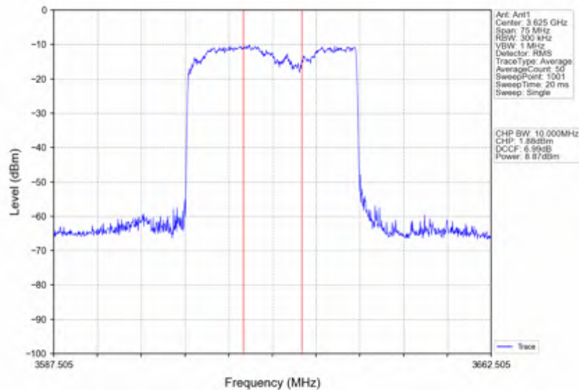
n78d_15kHz_SISO_NTNV_30MHz_CP-OFDM 64 QAM_3625.005MHz_Inner_Full
