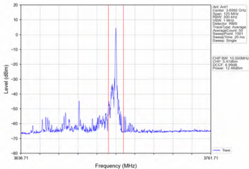
n78d_15kHz_SISO_NTNV_50MHz_DFT-s-OFDM PI/2 BPSK_3675MHz_Edge_1RB_Right
