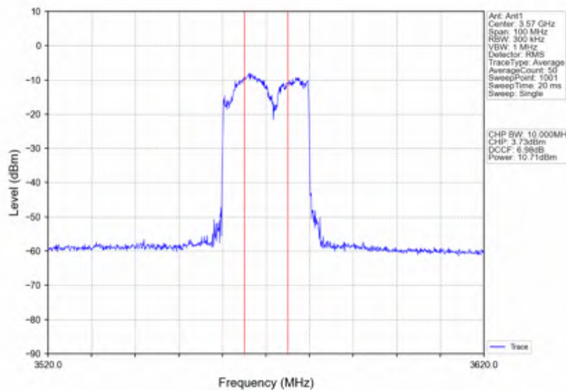
n78d_15kHz_SISO_NTNV_40MHz_DFT-s-OFDM 64 QAM_3570MHz_Inner_Full
