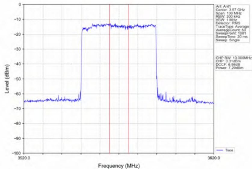
n78d_15kHz_SISO_NTNV_40MHz_DFT-s-OFDM PI/2 BPSK_3570MHz_Inner_Full
