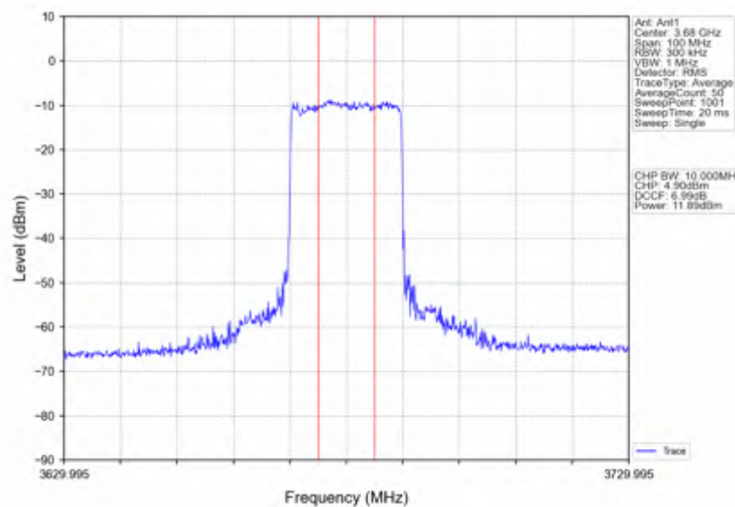
n78d 15kHz SISO NTNV 40MHz CP-OFDM 64 QAM 3679.995MHz Inner Full
