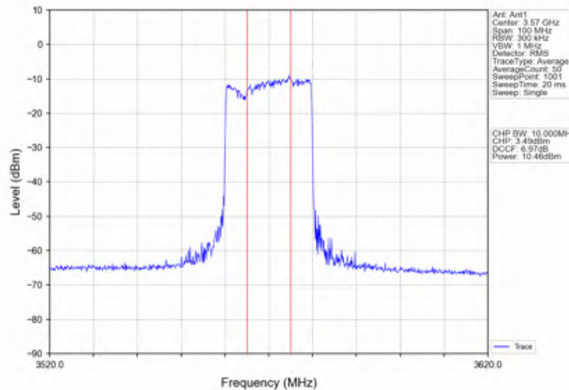
n78d_15kHz_SISO_NTNV_40MHz_DFT-s-OFDM PI/2 BPSK_3570MHz_Inner_Full
