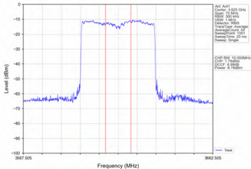
n78d_15kHz_SISO_NTNV_30MHz_CP-OFDM_16_QAM_3625.005MHz_Inner_Full
