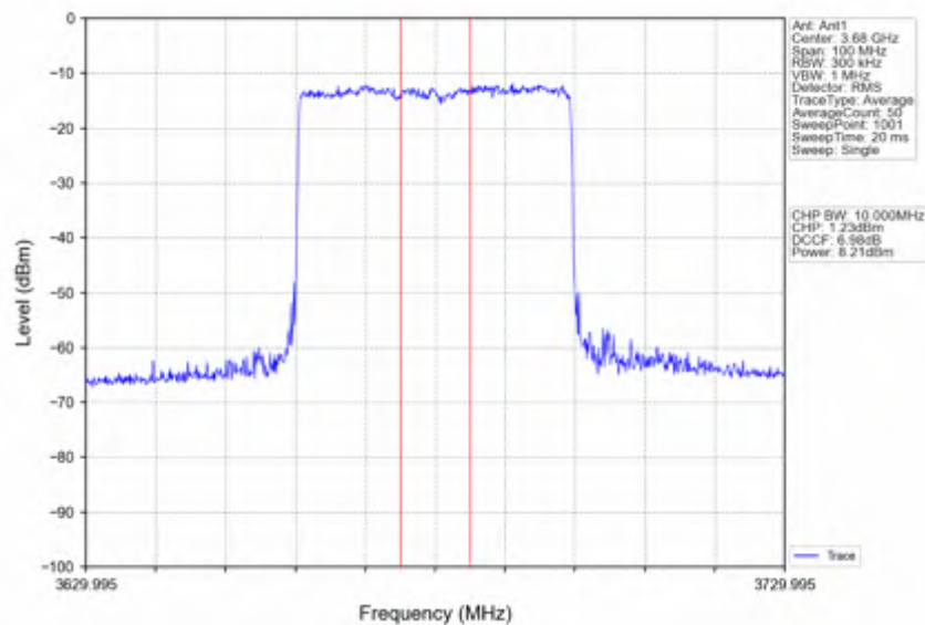
n78d_15kHz_SISO_NTNV_40MHz_CP-OFDM_16_QAM_3679.995MHz_Inner_Full
