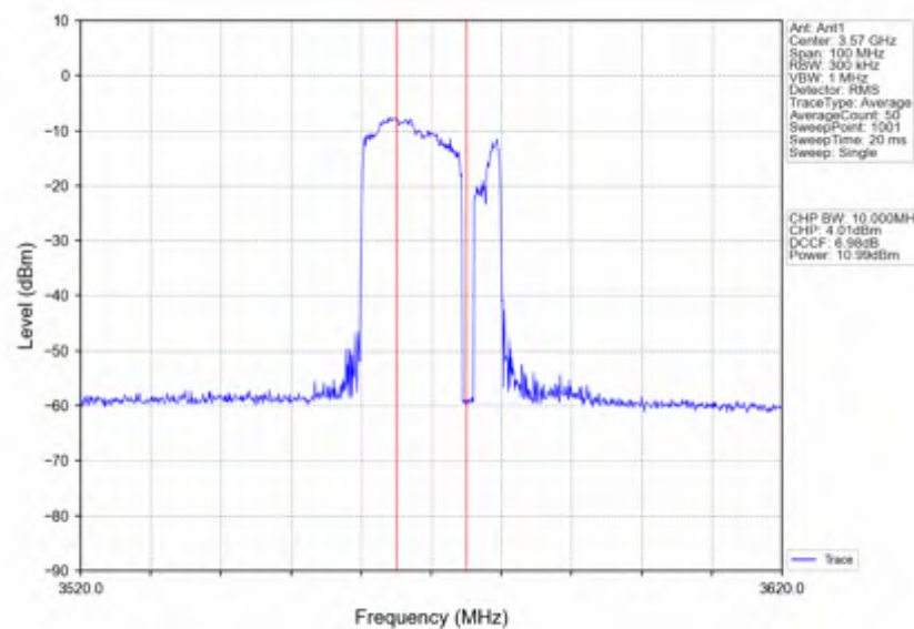
n78d 15kHz SISO NTNv 40MHz CP-OFDM 256 QAM 3570MHz Inner Full
