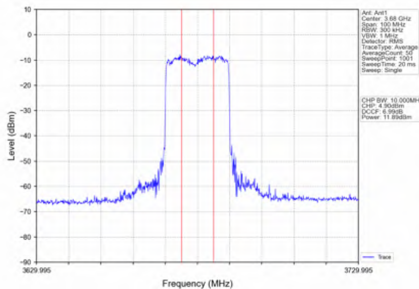
n78d_15kHz_SISO_NTNV_40MHz_DFT-s-OFDM_16_QAM_3679.995MHz_Inner_Full
