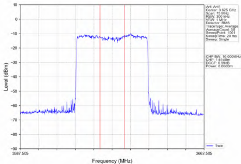
n78d_15kHz_SISO_NTNV_30MHz_DFT-s-OFDM 64 QAM_3625.005MHz_Inner_Full
