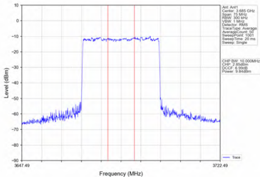
n78d_15kHz_SISO_NTNV_30MHz_CP-OFDM 256 QAM_3684.99MHz_Inner_Full
