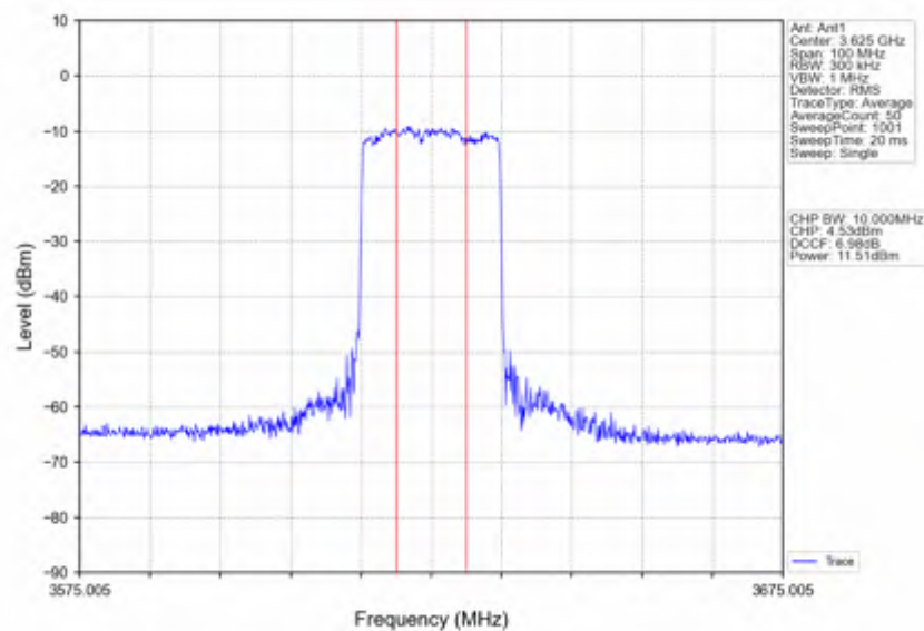
n78d_15kHz_SISO_NTNV_40MHz_CP-OFDM 64 QAM_3625.005MHz_Inner_Full
