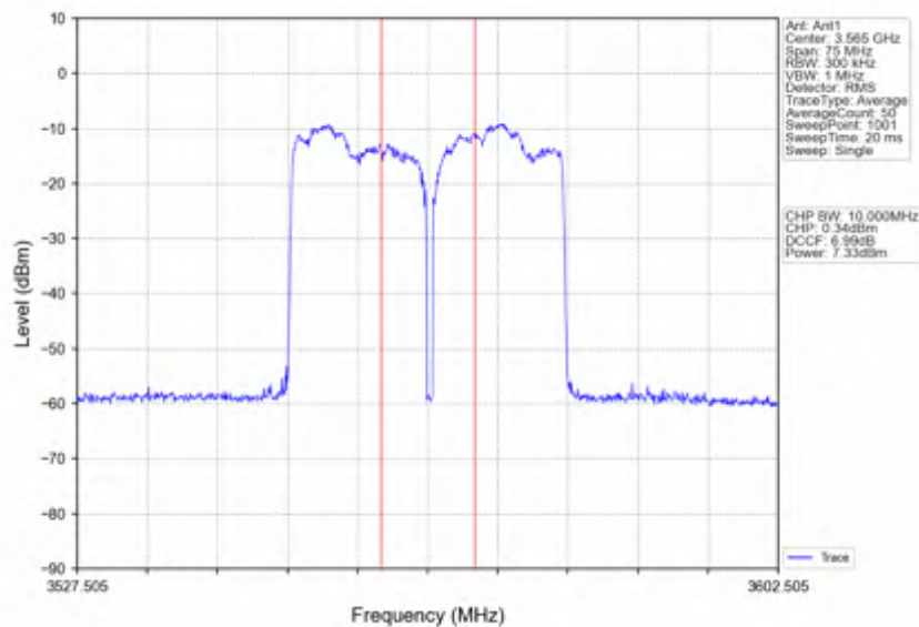
n78d_15kHz_SISO_NTNV_30MHz_CP-OFDM 64 QAM_3565.005MHz_Inner_Full
