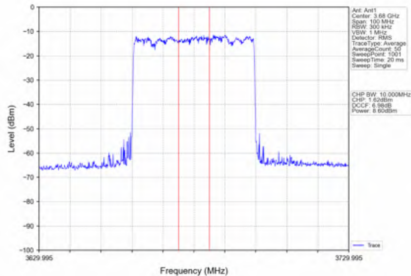
n78d_15kHz_SISO_NTNV_40MHz_DFT-s-OFDM 64 QAM_3679.995MHz_Inner_Full
