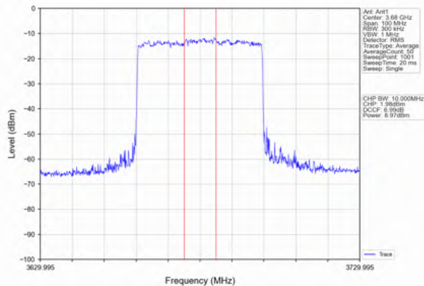
n78d 15kHz SISO NTNV 40MHz CP-OFDM 64 QAM 3679.995MHz Inner Full
