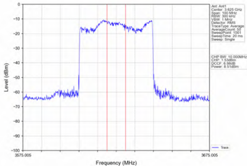
n78d_15kHz_SISO_NTNV_40MHz_DFT-s-OFDM QPSK_3625.005MHz_Inner_Full
