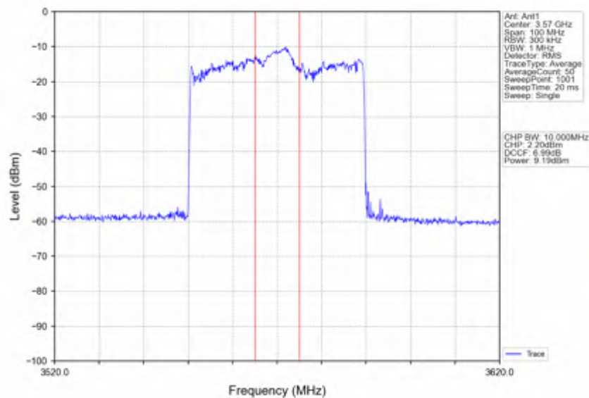
n78d_15kHz_SISO_NTNV_40MHz_DFT-s-OFDM_256_QAM_3570MHz_Inner_Full
