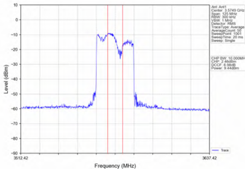
n78d 15kHz SISO NTNV 50MHz DFT-s-OFDM QPSK 3575.01MHz Inner Full
