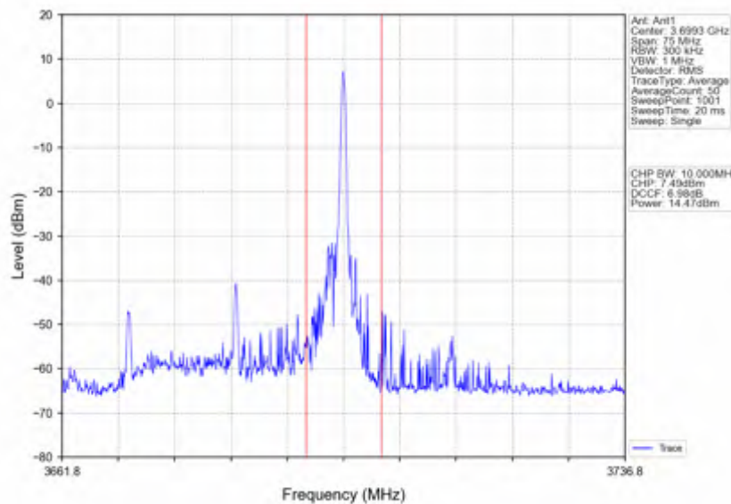
n78d_15kHz_SISO_NTV_30MHz_CP-OFDM QPSK_3684.99MHz_Edge_1RB_Right
