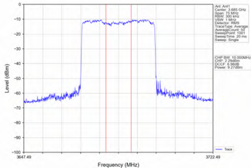
n78d_15kHz_SISO_NTNV_30MHz_CP-OFDM 16 QAM 3684.99MHz_Inner_Full
