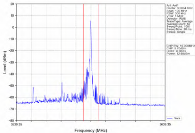
n78d_15kHz_SISO_NTNV_40MHz_DFT-s-OFDM_256_QAM_3570MHz_Edge_1RB_Right
