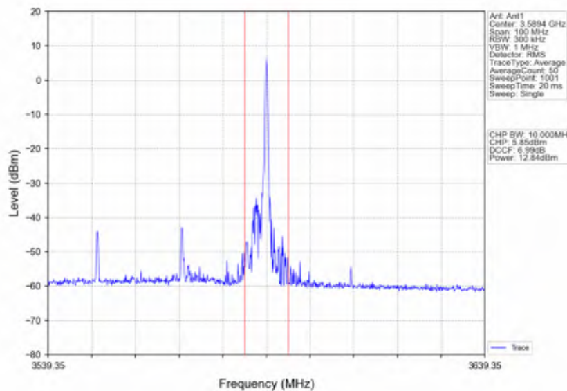
n78d_15kHz_SISO_NTNV_40MHz_DFT-s-OFDM 64 QAM_3570MHz_Edge_1RB_Right
