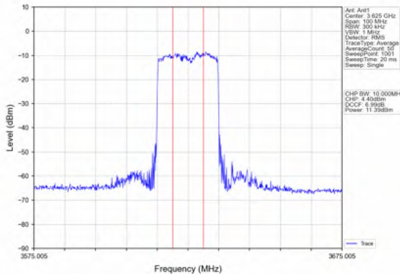
n78d_15kHz_SISO_NTNV_40MHz_DFT-s-OFDM QPSK_3625.005MHz_Inner_Full
