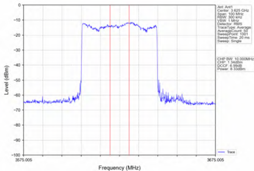
n78d 15kHz SISO NTNV 40MHz CP-OFDM 16 QAM 3625.005MHz Inner Full
