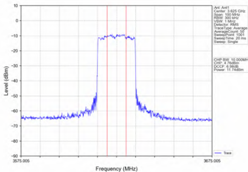
n78d 15kHz SISO NTNV 40MHz CP-OFDM 16 QAM 3625.005MHz Inner Full
