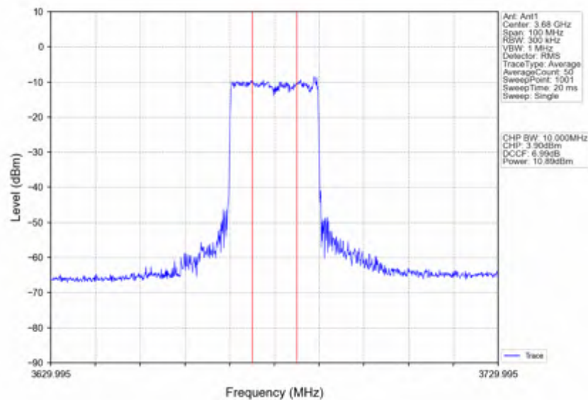
n78d_15kHz_SISO_NTNV_40MHz_DFT-s-OFDM QPSK_3679.995MHz_Inner_Full
