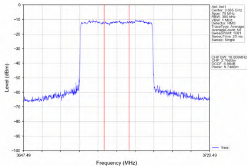
n78d_15kHz_SISO_NTNV_30MHz_CP-OFDM QPSK_3684.99MHz_Inner_Full
