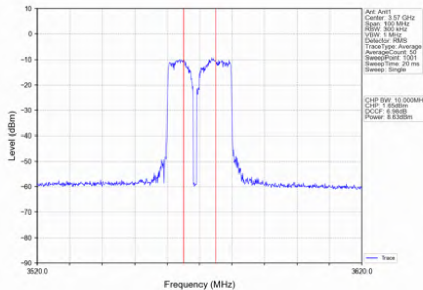
n78d_15kHz_SISO_NTNV_40MHz_DFT-s-OFDM_QPSK_3570MHz_Inner_Full
