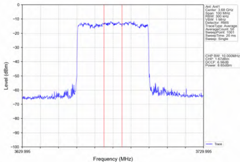
n78d_15kHz_SISO_NTNV_40MHz_DFT-s-OFDM QPSK_3679.995MHz_Inner_Full
