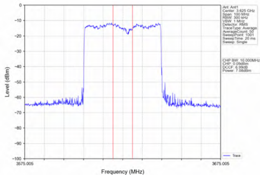
n78d_15kHz_SISO_NTNV_40MHz_CP-OFDM 64 QAM_3625.005MHz_Inner_Full
