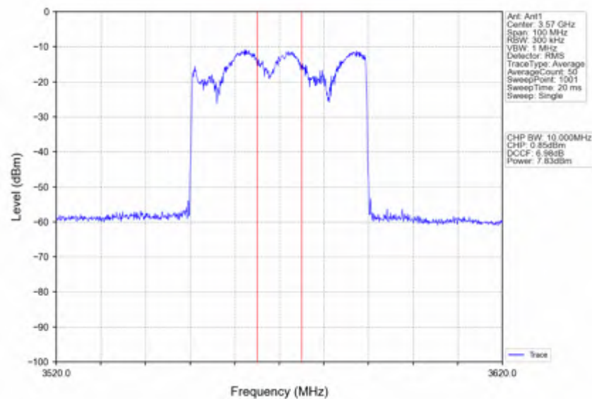
n78d_15kHz_SISO_NTNV_40MHz_DFT-s-OFDM_QPSK_3570MHz_Inner_Full
