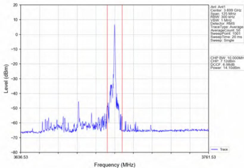
n78d_15kHz_SISO_NTNV_50MHz_DFT-s-OFDM_PI/2_BPSK_3675MHz_Inner_1RB_Right
