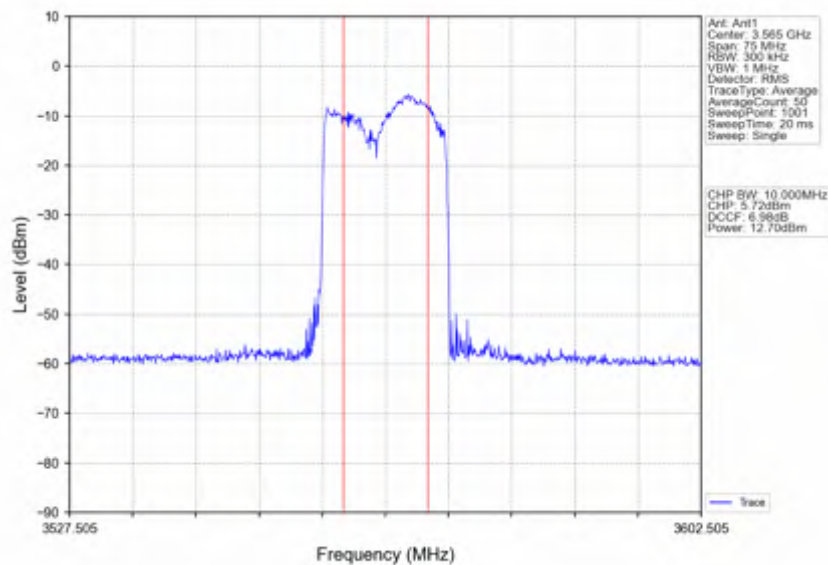
n78d_15kHz_SISO_NTNV_30MHz_DFT-s-OFDM 256 QAM_3565.005MHz_Inner_Full
