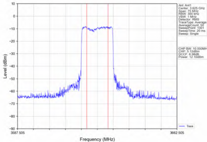
n78d_15kHz_SISO_NTNV_30MHz_CP-OFDM 64 QAM_3625.005MHz_Inner_Full
