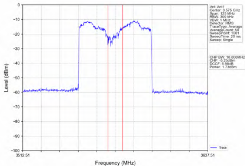
n78d 15kHz SISO NTNV 50MHz DFT-s-OFDM QPSK 3575.01MHz Inner Full
