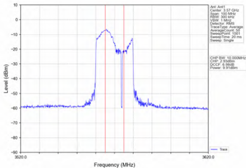
n78d_15kHz_SISO_NTNV_40MHz_CP-OFDM_QPSK_3570MHz_Inner_Full
