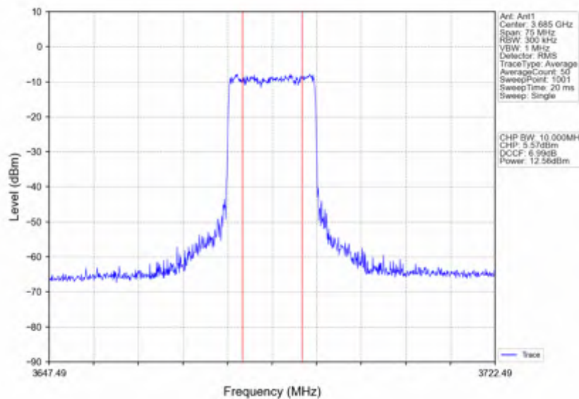
n78d_15kHz_SISO_NTNV_30MHz_DFT-s-OFDM_256_QAM_3684.99MHz_Inner_Full
