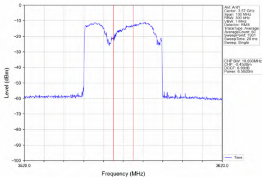
n78d_15kHz_SISO_NTNV_40MHz_CP-OFDM 64 QAM_3570MHz_Inner_Full
