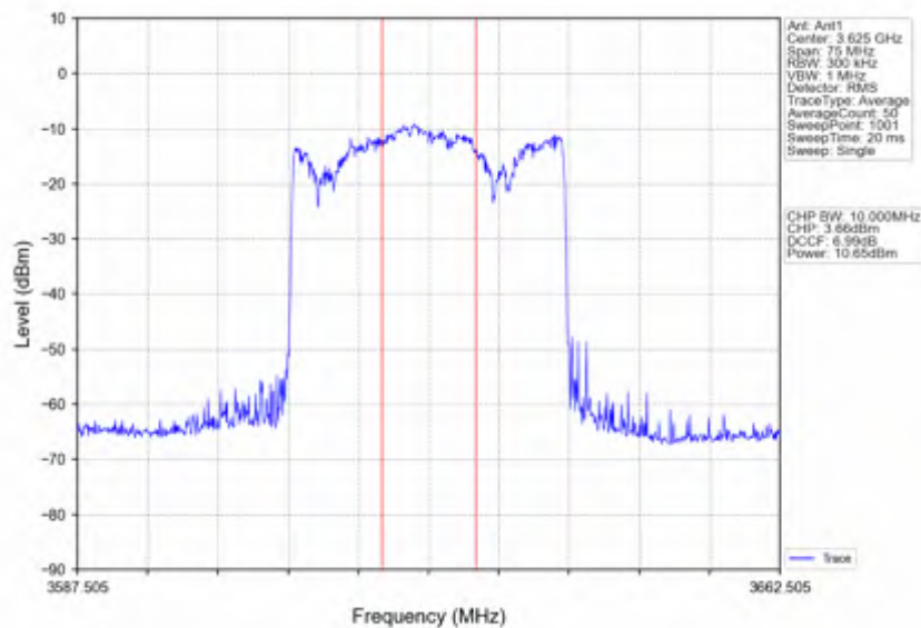
n78d 15kHz SISO NTNV 30MHz DFT-s-OFDM 16 QAM 3625.005MHz Inner Full
