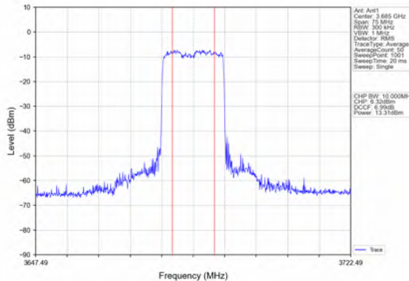
n78d_15kHz_SISO_NTNV_30MHz_CP-OFDM 16 QAM 3684.99MHz_Inner_Full
