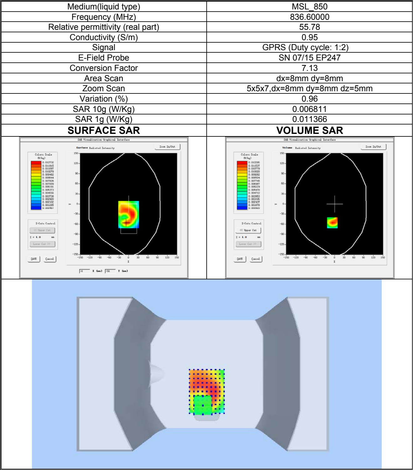
Plot 2: GPRS850MHz, Middle channel (Body-worn, Back Surface) Product Description: Smart Phone Test Date: 2019-05-07
