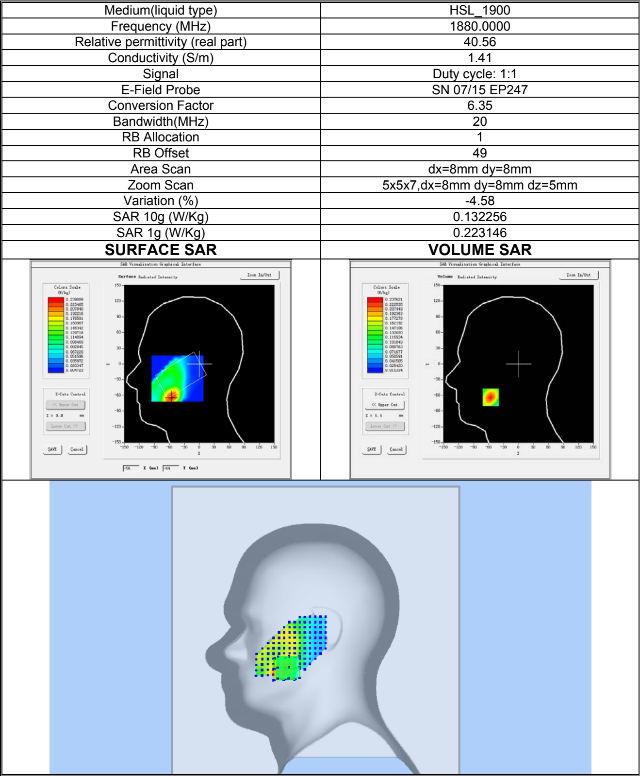
Plot 15:LTE BAND2, Middle channel (Right Head Cheek) Product Description:Smart phone Test Date: 2019-05-07
