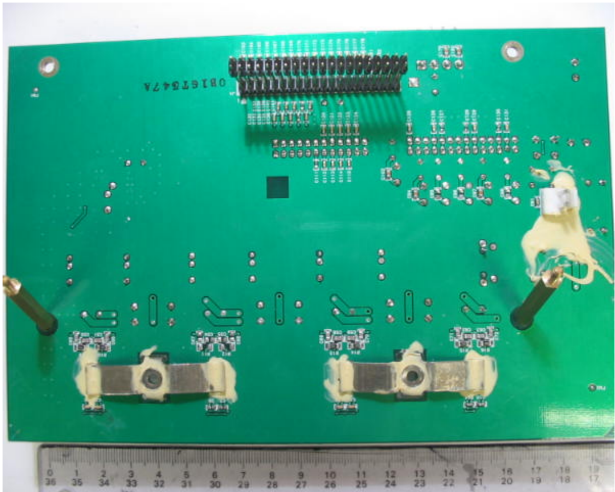
EUT PCB Trace Side
