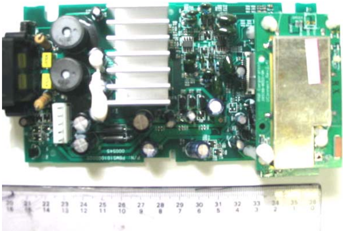
EUT PCB Component Side
