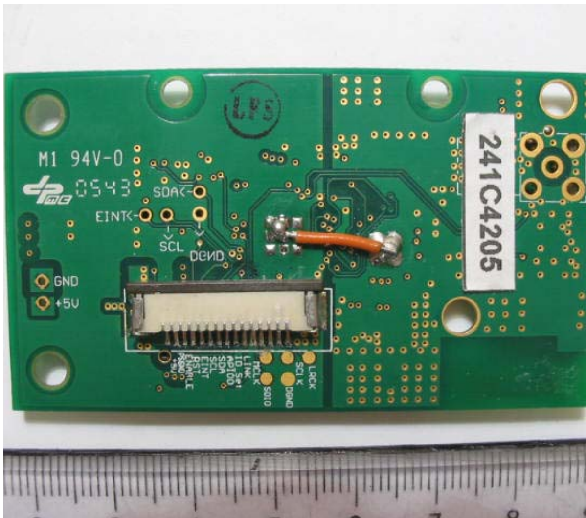
EUT PCB Trace Side
