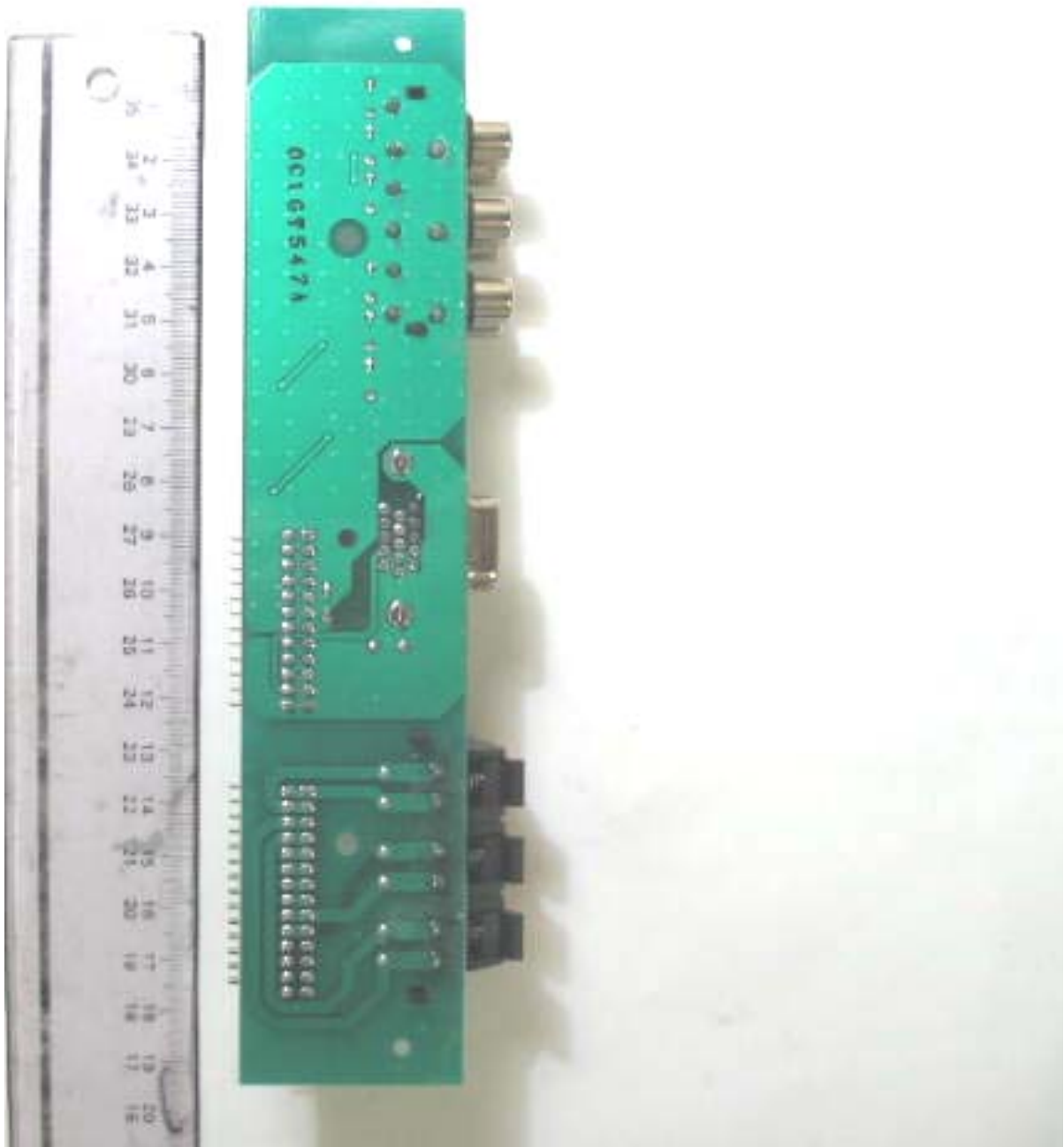
EUT PCB Trace Side
