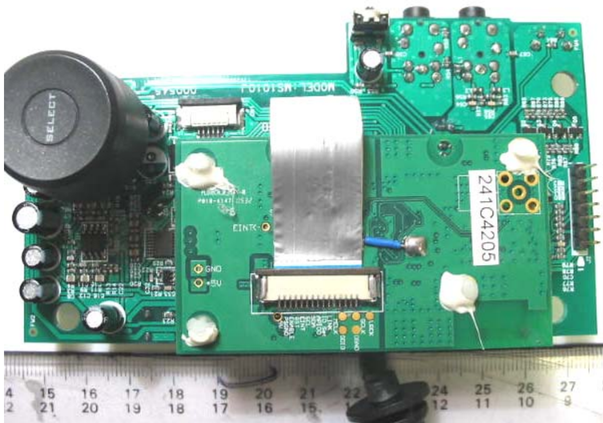
EUT PCB Component Side
