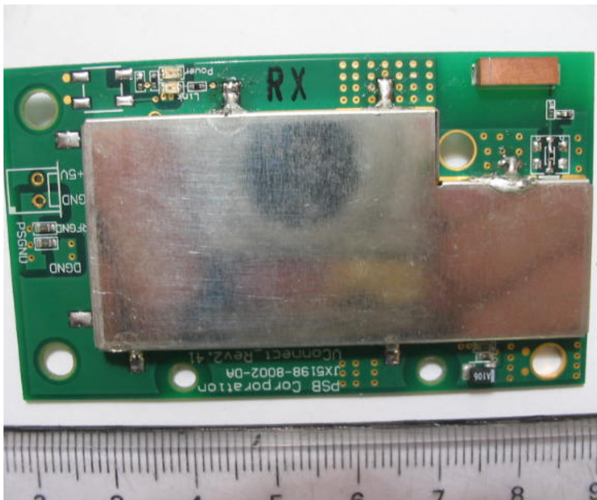
EUT PCB Component Side
