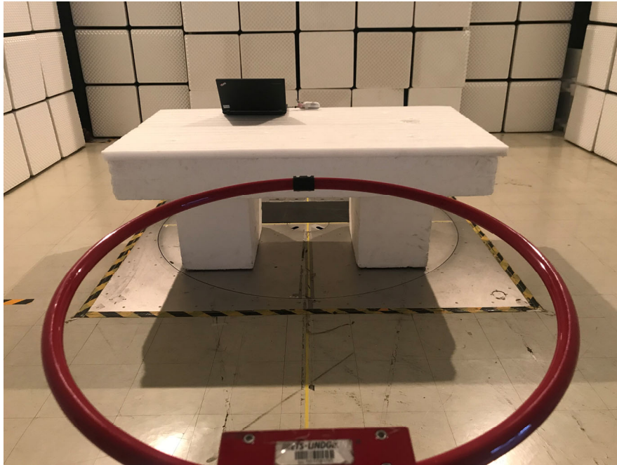
Radiated Emissions-parallel view (Below 30 MHz)
