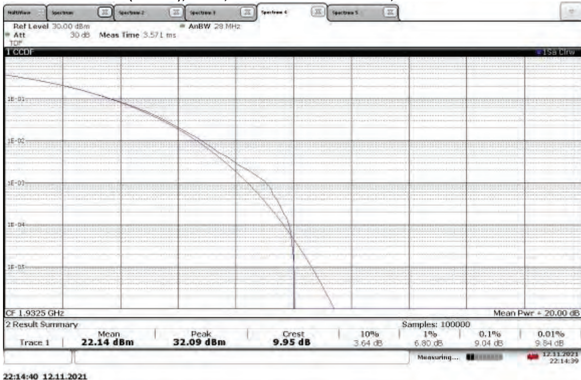
TM1.1-QPSK_5 MHz Bandwidth Slot 0 (Band 2), ANT1, Low Channel 1932.5 MHz, PAPR = 9.95 dB
