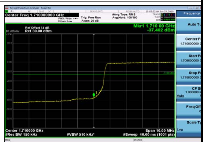
LowRange_FDD04_15MHz_1717.5_fullRB _Low_Q16
