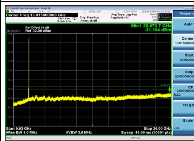
FDD07_MidRange_20MHz_30MHz~26GHz
