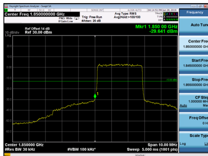
LowRange_FDD02_3MHz_1851.5_fullRB _Low_QPSK
