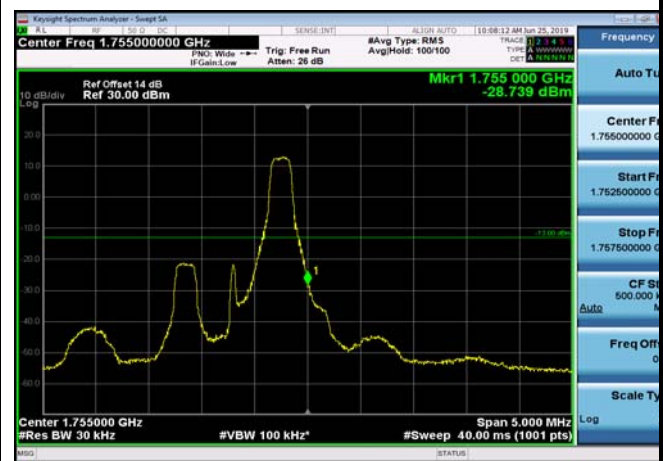
HighRange_FDD04_1.4MHz_1754.3_OneRB _high_Q16
