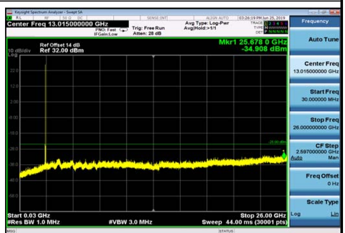
FDD07_MidRange_15MHz_30MHz~26GHz
