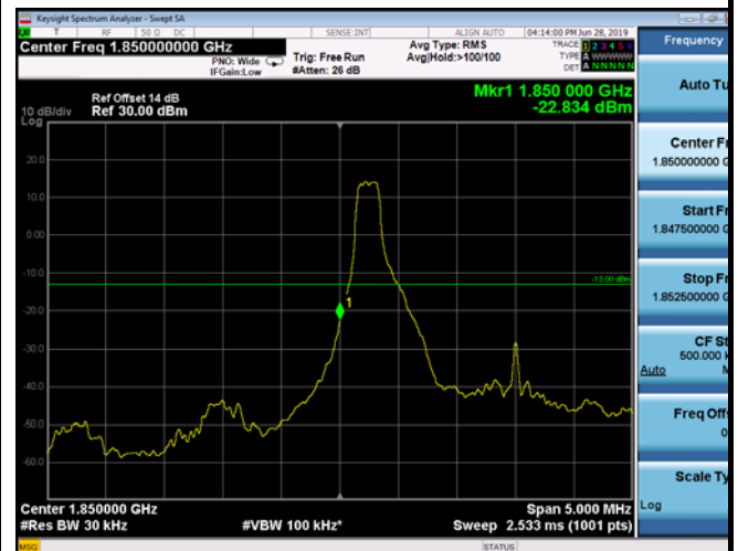
LowRange_FDD02_3MHz_1851.5_fullRB _Low_Q16
