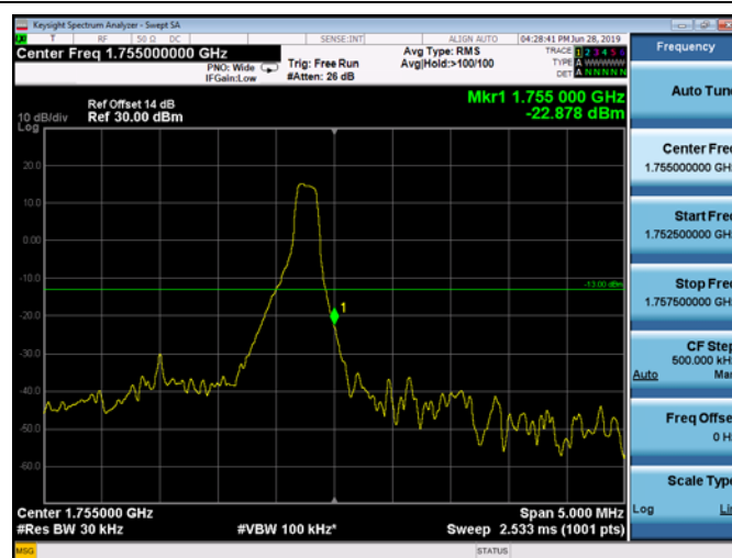
HighRange_FDD04_3MHz_1753.5_OneRB _high_QPSK
