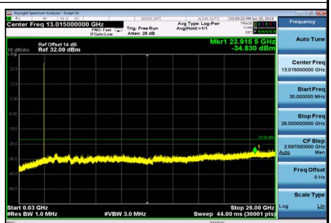
FDD07_HighRange_5MHz_30MHz~26GHz
