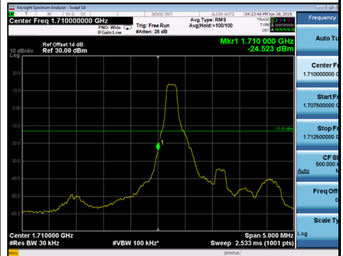
LowRange_FDD04_1.4MHz_1710.7_fullRB _Low_Q16
