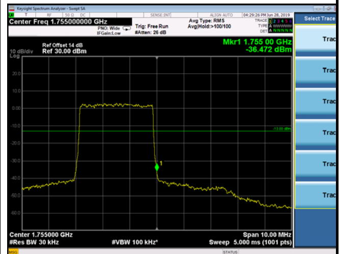
HighRange_ FDD04_5MHz_1752.5_OneRB _high_Q16
