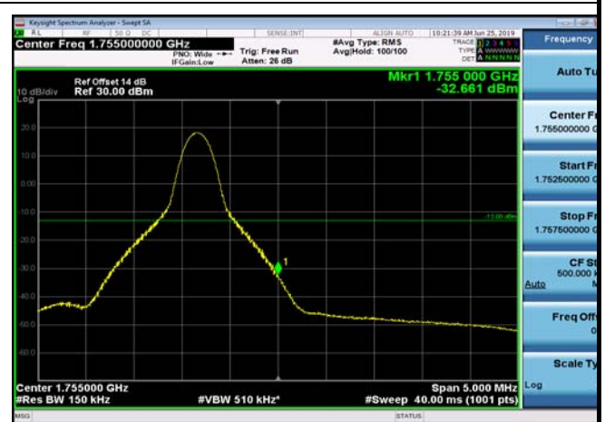
HighRange_FDD04_15MHz_1747.5_fullRB _High_Q16
