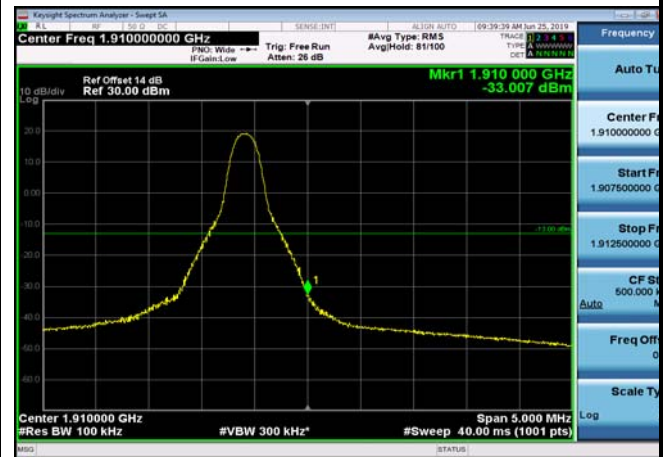
HighRange_FDD02_10MHz_1905_fullIRB _High_Q16
