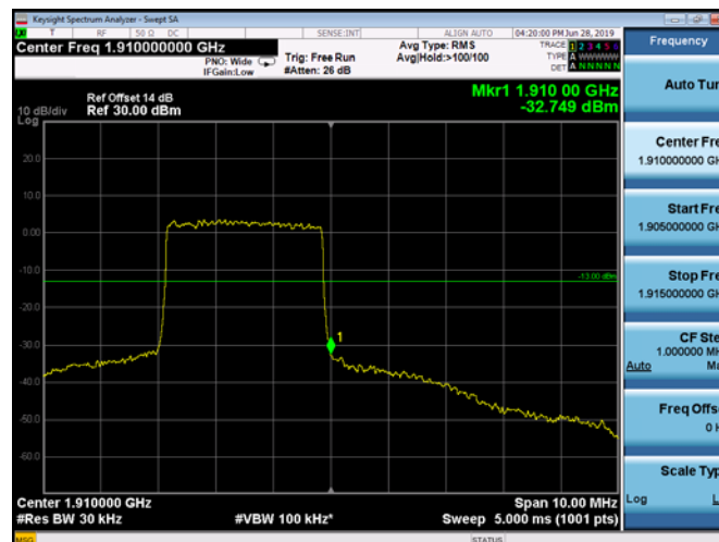
HighRange_FDD02_3MHz_1908.5_fullIRB _High_QPSK
