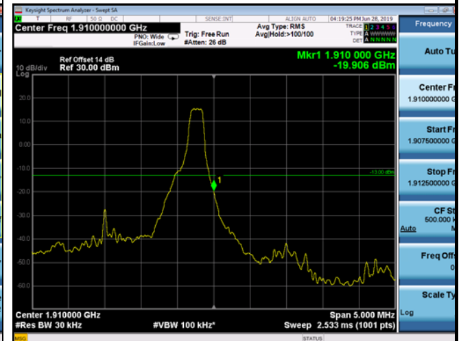
HighRange_FDD02_3MHz_1908.5_fullIRB _High_Q16
