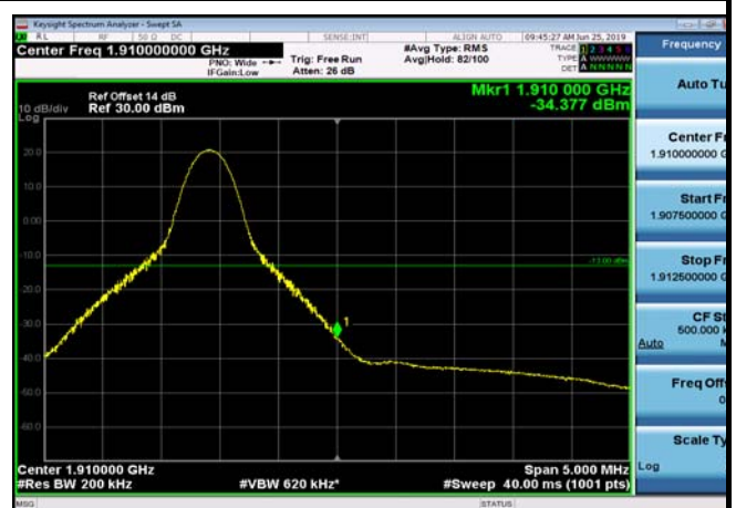
HighRange_FDD02_20MHz_1900_fullRB _High_Q16
