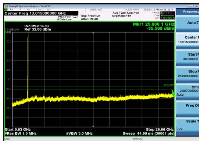
FDD07_MidRange_10MHz_30MHz~26GHz
