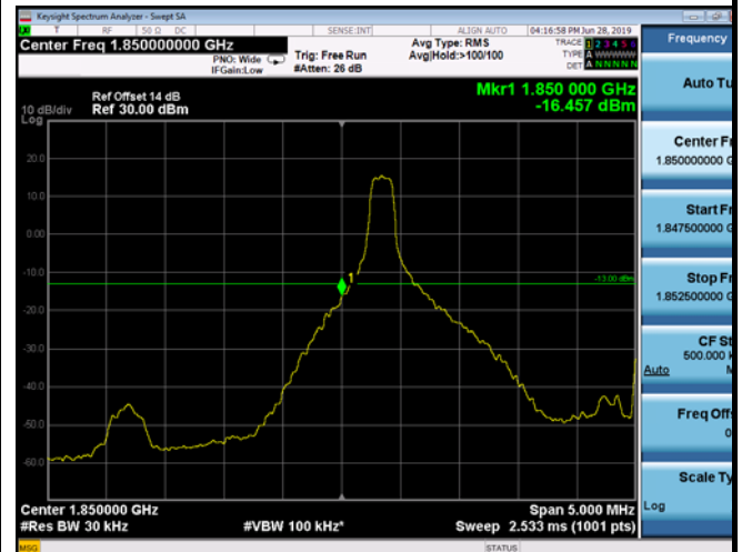
LowRange_FDD02_5MHz_1852.5_fullRB _Low_Q16
