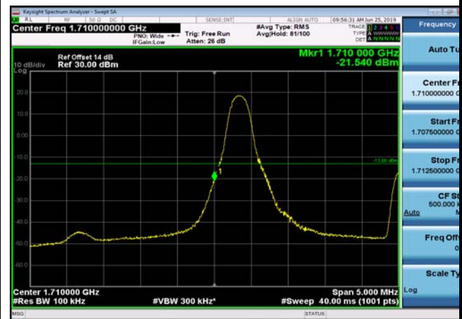
LowRange_FDD04_5MHz_1712.5_fullRB _Low_Q16
