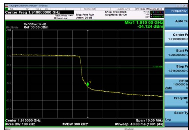
HighRange_FDD02_15MHz_1902.5_OneRB _high_Q16
