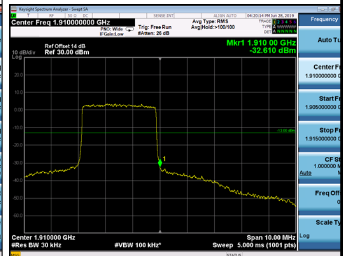
HighRange_FDD02_3MHz_1908.5_fullIRB _High_Q16
