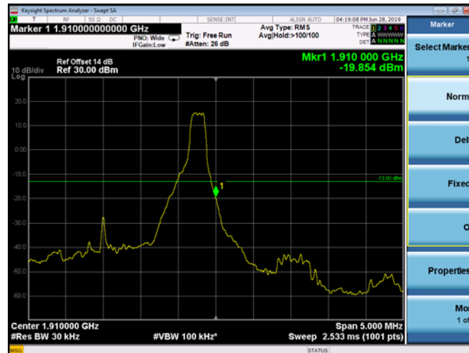
HighRange_FDD02_3MHz_1908.5_fullIRB _High_QPSK
