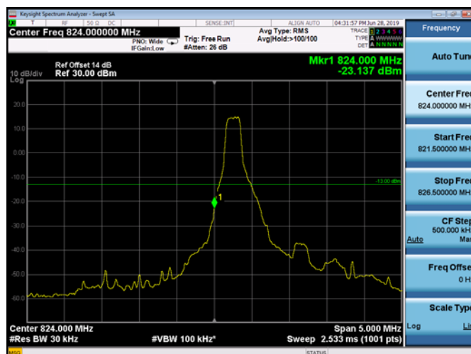
LowRange_FDD05_1.4MHz_824.7_OneRB _low_QPSK
