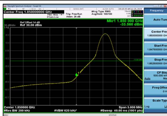
LowRange_FDD02_20MHz_1860_fullIRB _Low_QPSK
