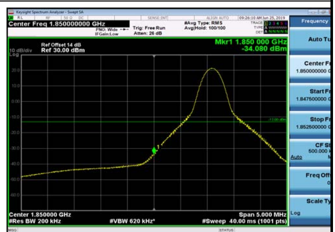
LowRange_FDD02_20MHz_1860_fullIRB _Low_Q16
