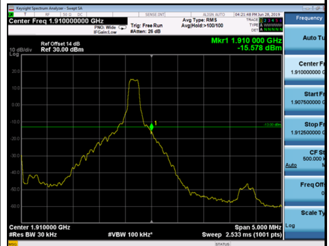
HighRange_FDD02_5MHz_1907.5_fullIRB _High_Q16
