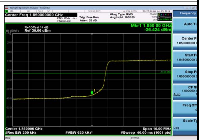
LowRange_FDD02_20MHz_1860_fullIRB _Low_Q16
