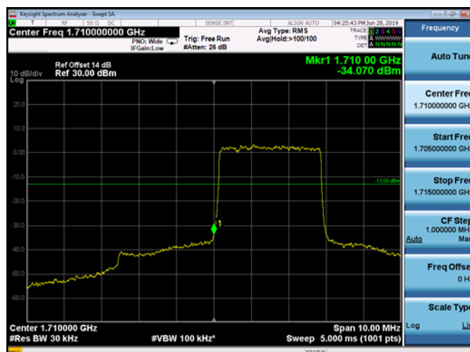
LowRange_FDD04_3MHz_1711.5_fullRB _Low_QPSK
