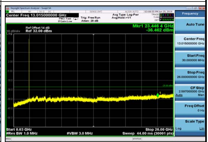
FDD07_MidRange_5MHz_30MHz~26GHz
