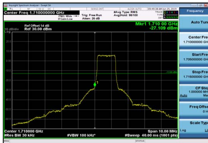
LowRange_FDD04_1.4MHz_1710.7_fullRB _Low_QPSK
