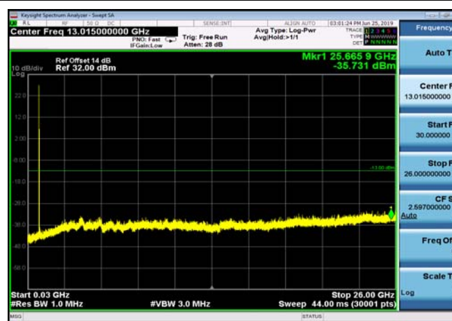
FDD07_HighRange_10MHz_30MHz~26GHz
