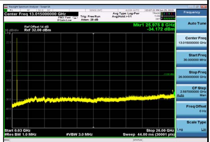
FDD07_HighRange_15MHz_30MHz~26GHz
