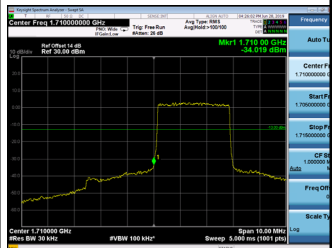
LowRange_FDD04_3MHz_1711.5_fullRB _Low_Q16
