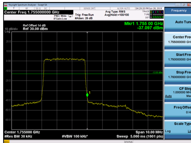
HighRange_ FDD04_5MHz_1752.5_OneRB _high_QPSK
