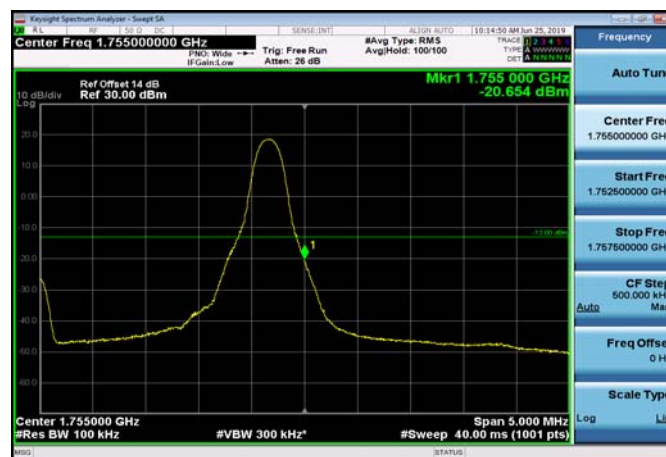
HighRange_ FDD04_5MHz_1752.5_OneRB _high_QPSK
