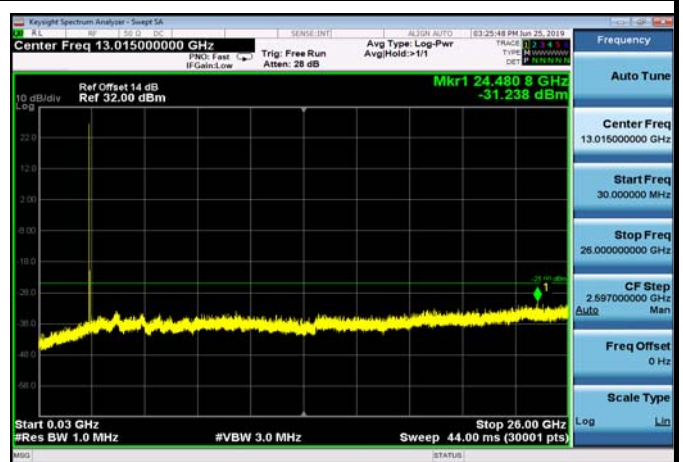
FDD07_LowRange_5MHz_30MHz~26GHz
