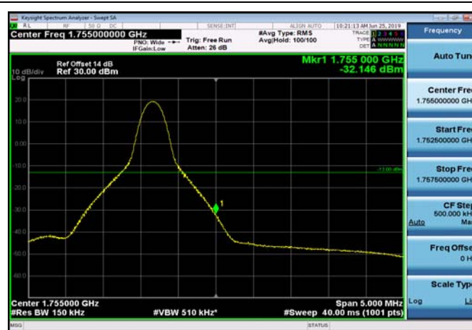
HighRange_FDD04_15MHz_1747.5_fullRB _High_QPSK
