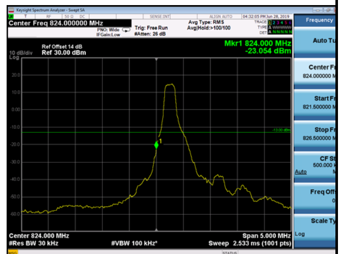
LowRange_FDD05_1.4MHz_824.7_OneRB _low_Q16
