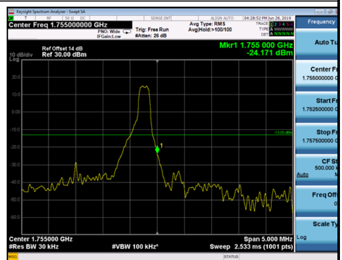
HighRange_FDD04_3MHz_1753.5_OneRB _high_Q16
