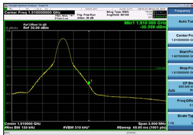
HighRange_FDD02_15MHz_1902.5_OneRB _high_QPSK
