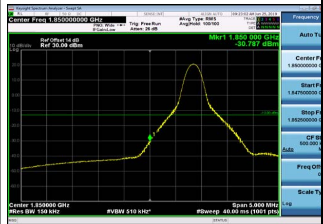
LowRange_FDD02_15MHz_1857.5_OneRB _low_Q16
