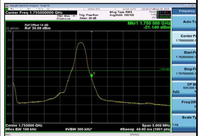
HighRange_ FDD04_5MHz_1752.5_OneRB _high_Q16
