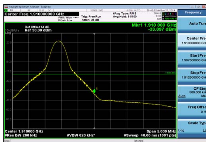
HighRange_FDD02_20MHz_1900_fullRB _High_QPSK
