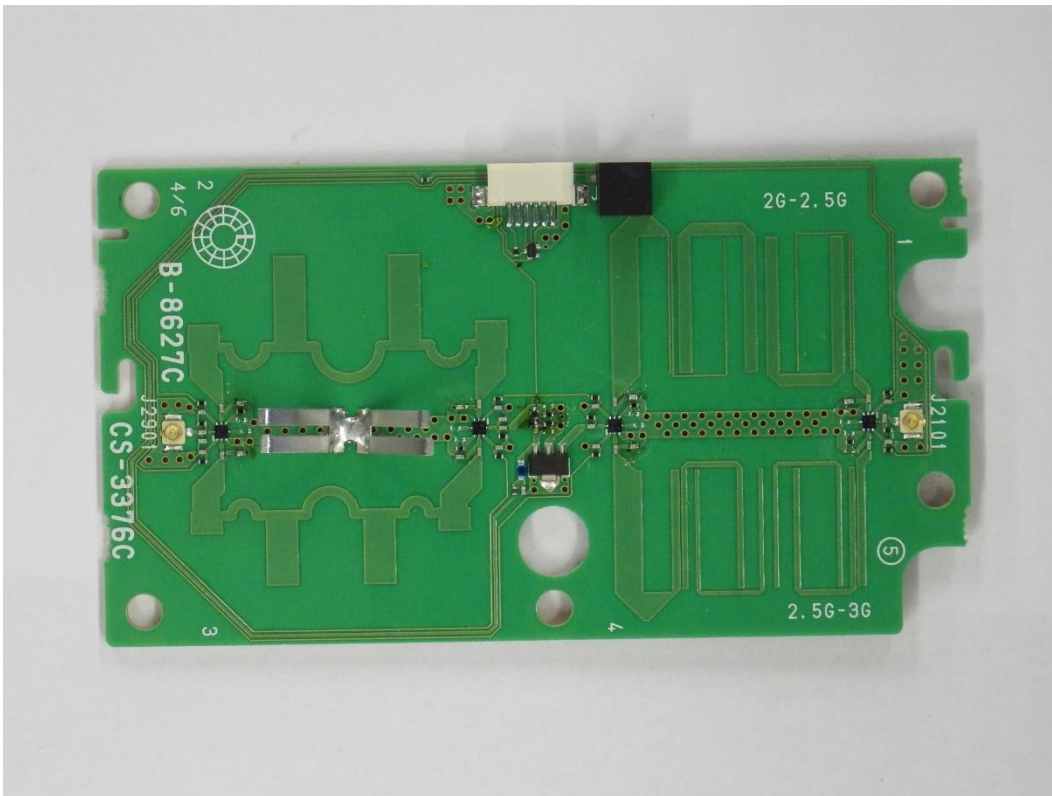
CONV-BPF_SIDE_A
