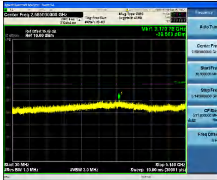
11N20ISO_Ant1_5220_5360-40000
