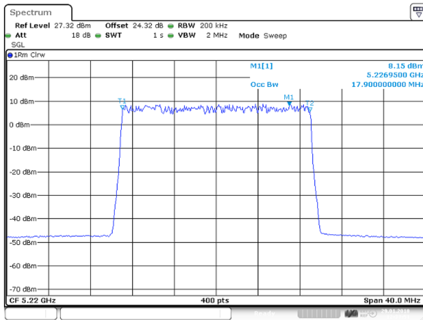
Figure 35 Occupied Bandwidth – 16QAM (5220.0 MHz) (20MHz Channel BW)
