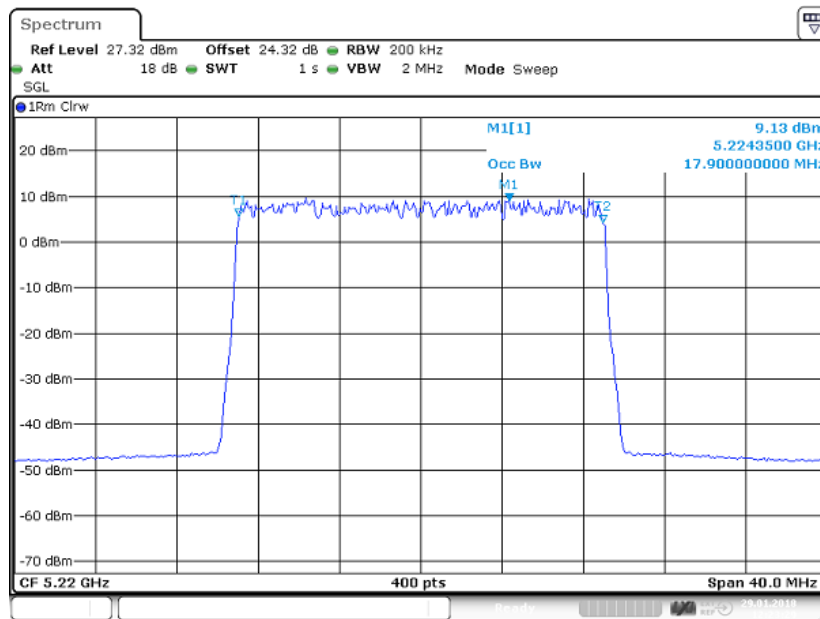
Figure 31 Occupied Bandwidth – 16QAM (5220.0 MHz) (20MHz Channel BW)
