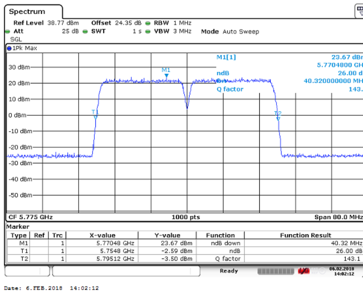
Figure 70 Occupied Bandwidth – 64QAM (5765.0/ 5785.0 MHz) (20MHz Channel BW)
