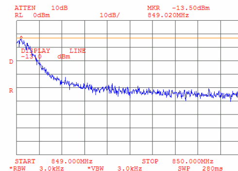
Plot 7.2.11 Bandedge emission measurements in 849 - 850 MHz range at high carrier frequency
