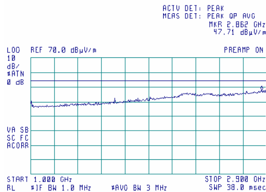
Plot 7.4.12 Radiated emission measurements from 1000 to 2900 MHz at the high carrier frequency
