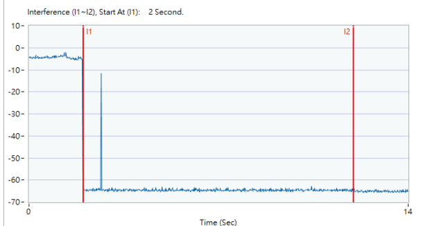
Contention Based Protocol - UNII 7, EUT-6695(BW20), SG-6695(-1)
