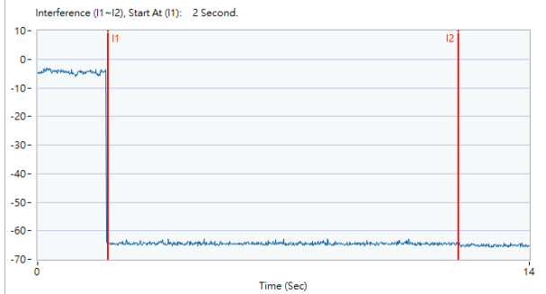
Contention Based Protocol - UNII 7, EUT-6695(BW20), SG-6695
