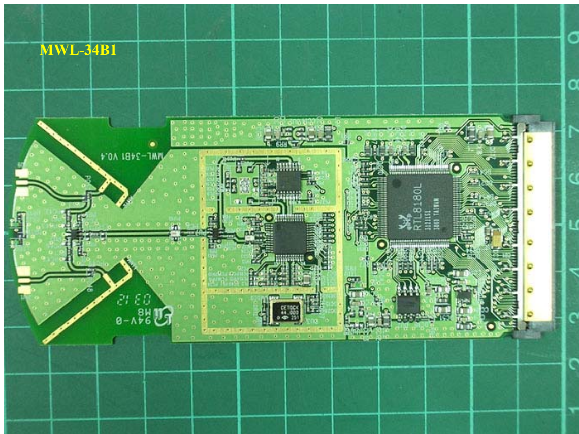
Photo 1: Inner view
