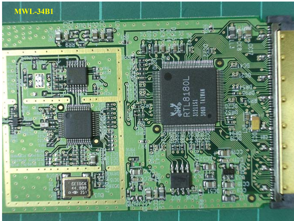
Photo 2: Inner view
