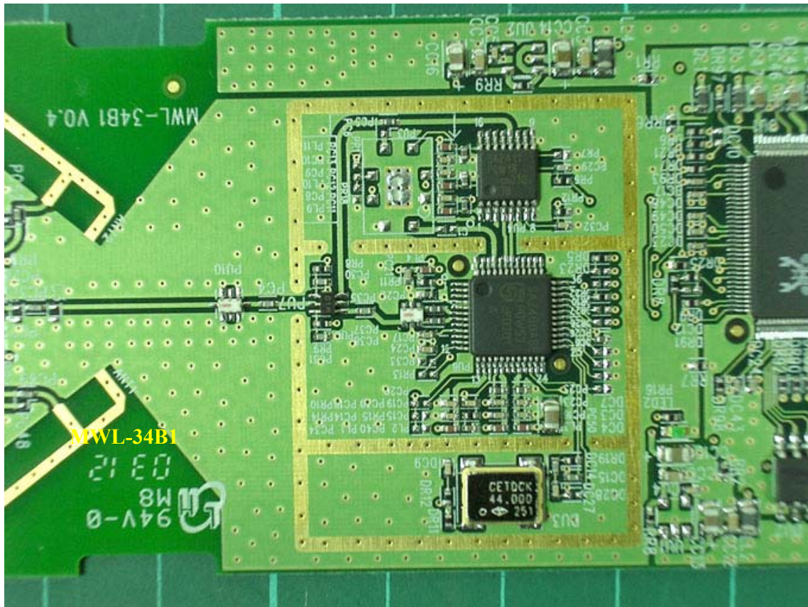
Photo 3: Inner view
