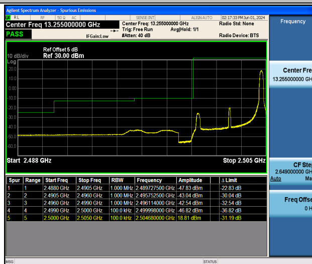
Band7_5MHz_QPSK_20775_1RB#24
