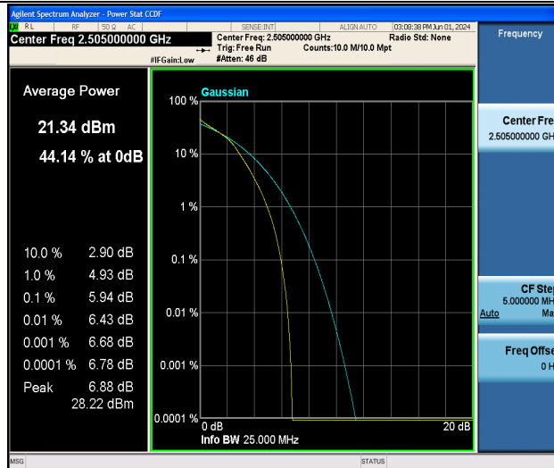
Band7-10MHz-16QAM-20800-50RB#0-PASS
