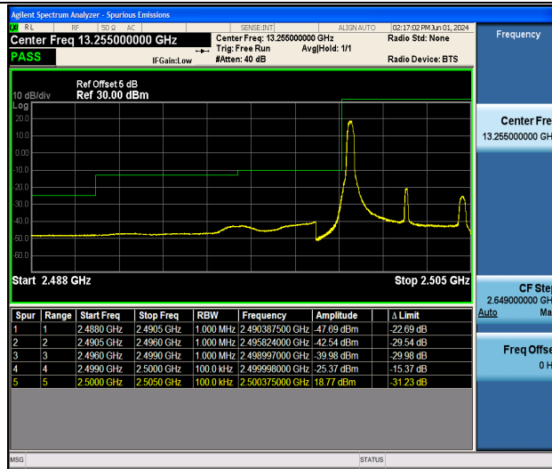
Band7_5MHz_QPSK_20775_1RB#0
