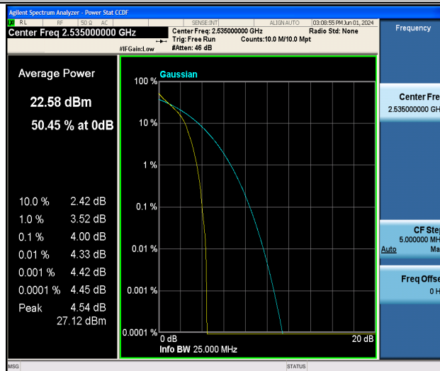
Band7-10MHz-QPSK-21100-1RB#0-PASS
