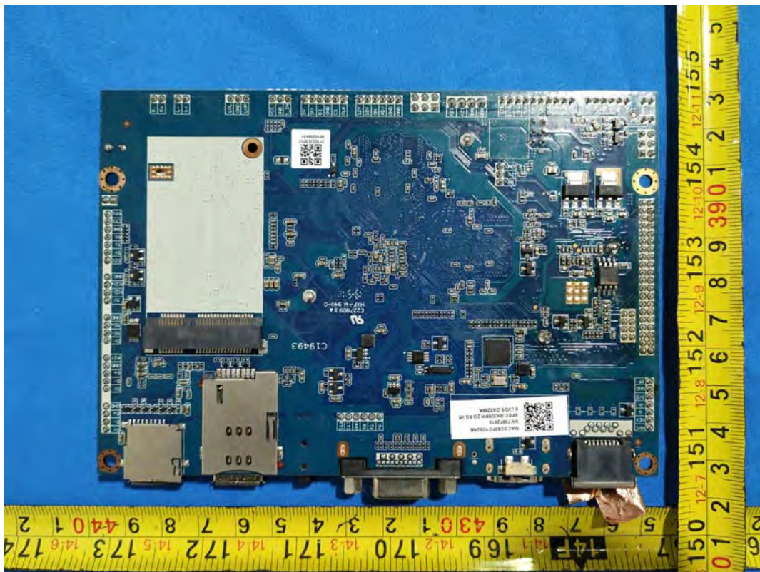
RF Board bottom
