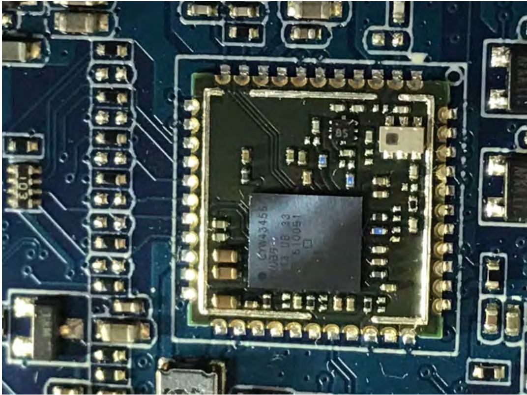
RF Module unshielded
