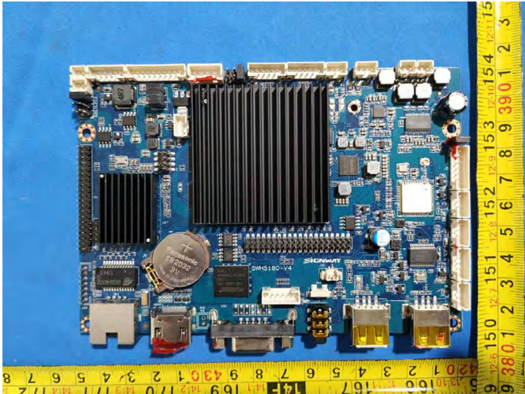
RF Board top unshielded
