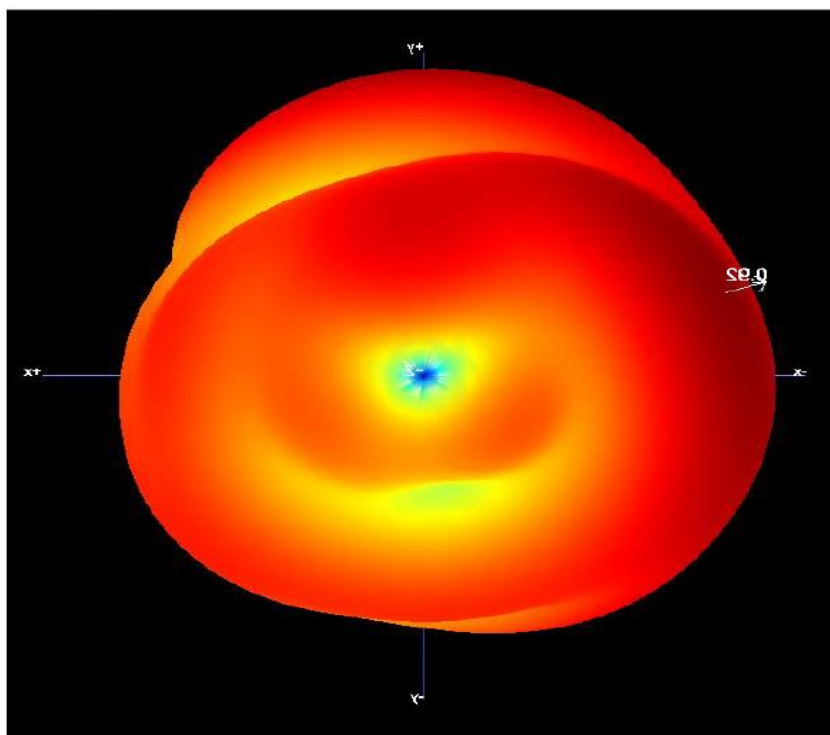
3D Pattern for 2400MHz
