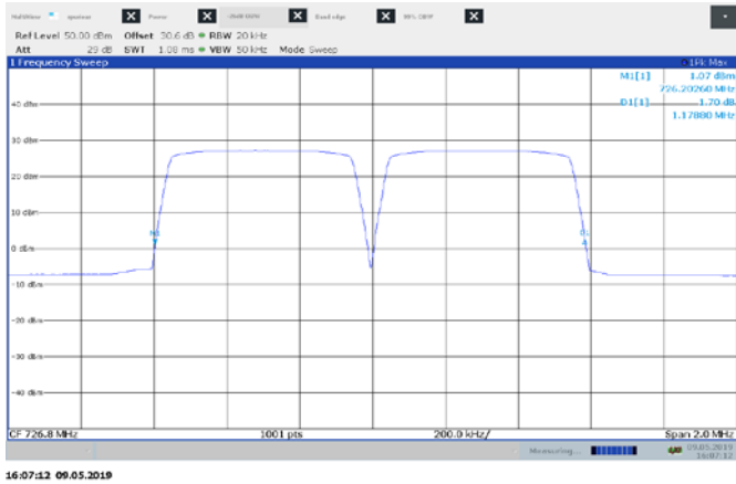
Figure 8.5-7: 26 dB bandwidth for two carrier high channel
