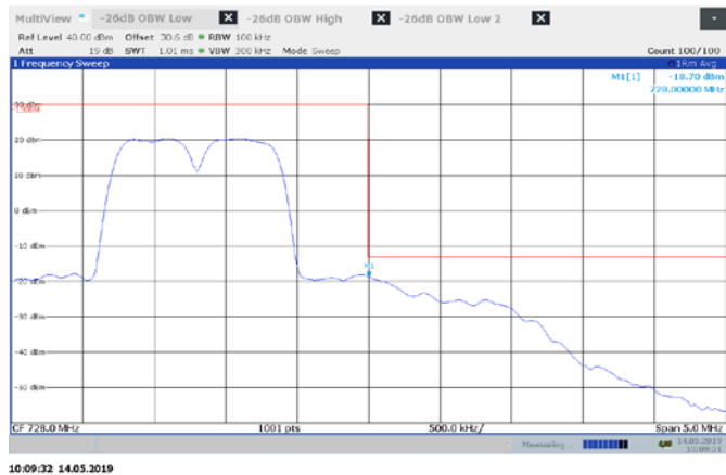
Figure 8.2-11: Upper band edge for two carrier
