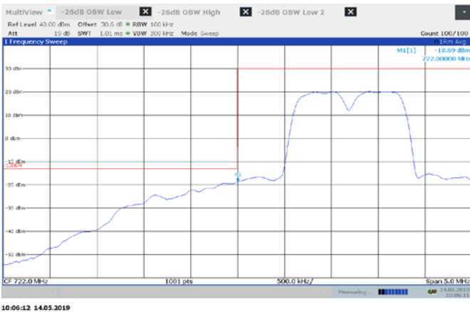
Figure 8.2-10: Lower band edge for two carrier
