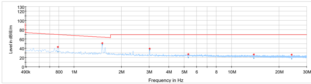
Radiates Emission from 490kHz to 30MHz
