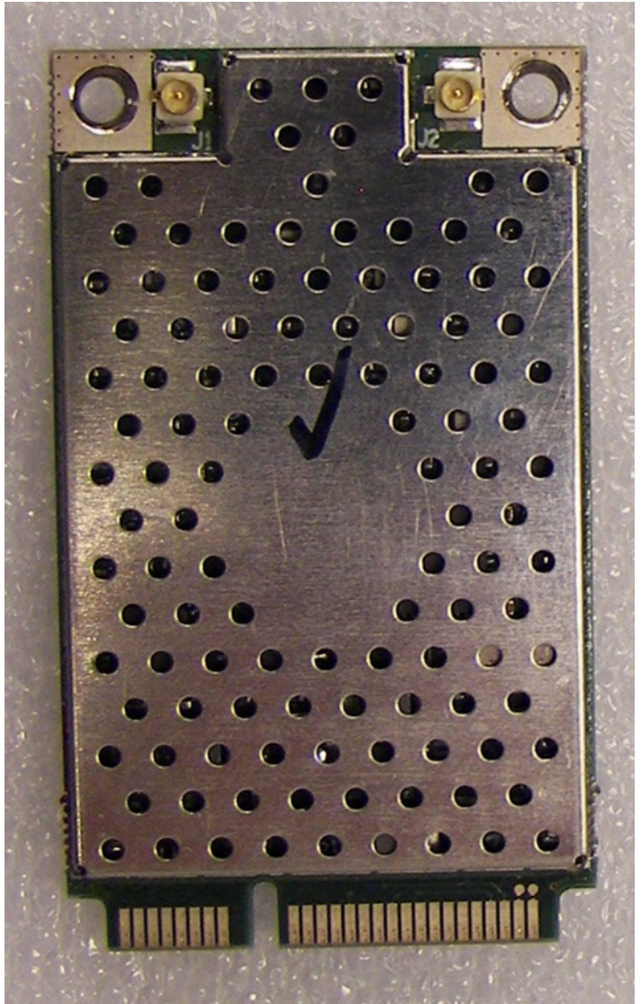
IM11 RFID Module (front)
