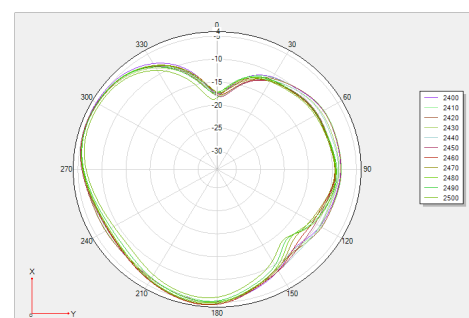
◎ 2D Gain Pattern Theta 90
