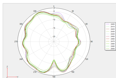
◎ 2D Gain Pattern Theta 60
