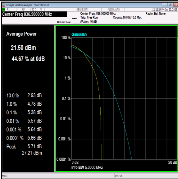
Band5-5MHz-64QAM-20525-1RB#0-PASS
