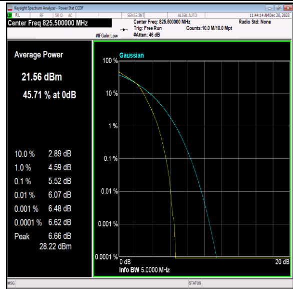
Band5-3MHz-16QAM-20415-15RB#0-PASS
