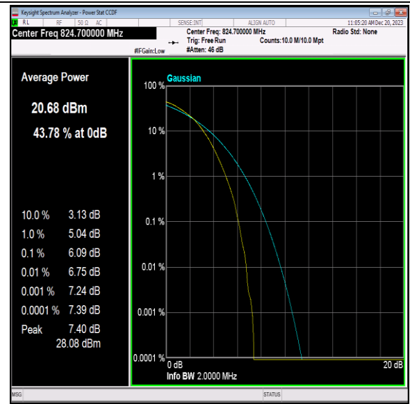
Band5-1.4MHz-64QAM-20407-6RB#0-PASS
