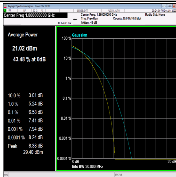
Band2-20MHz-64QAM-18700-100RB#0-PASS
