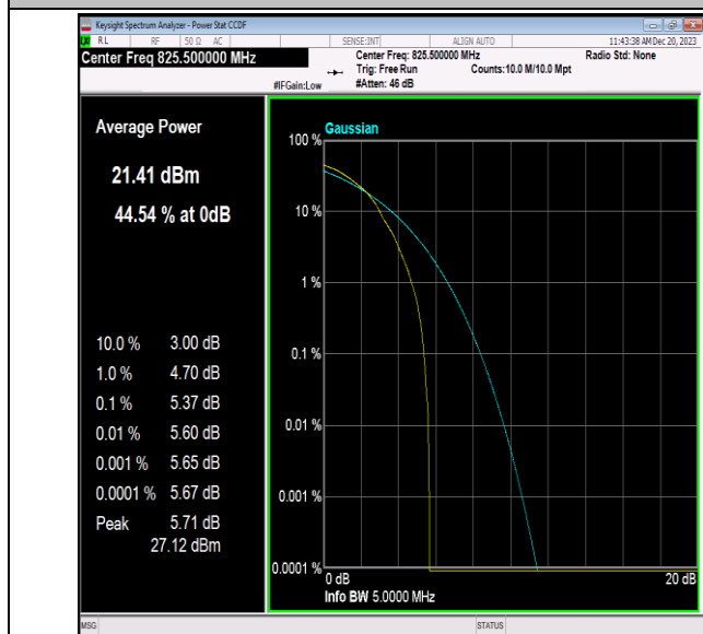
Band5-3MHz-64QAM-20415-1RB#0-PASS
