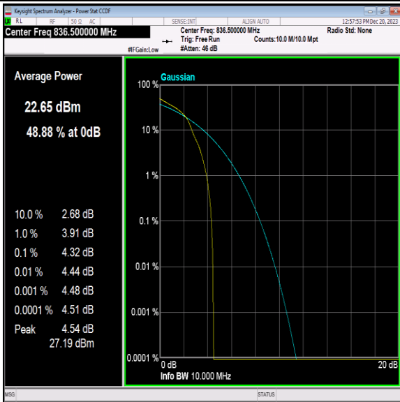
Band5-10MHz-16QAM-20525-1RB#0-PASS
