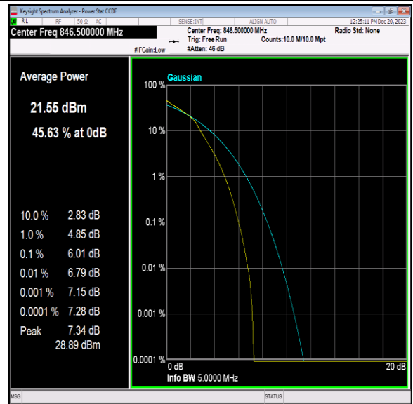
Band5-5MHz-16QAM-20625-25RB#0-PASS
