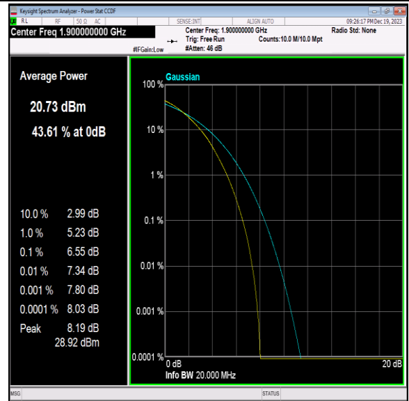
Band2-20MHz-64QAM-19100-100RB#0-PASS
