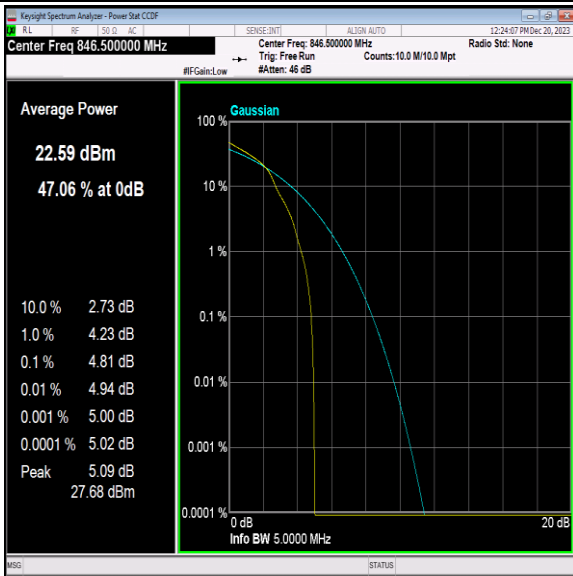
Band5-5MHz-16QAM-20625-1RB#0-PASS
