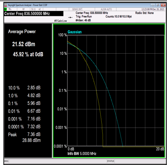
Band5-5MHz-16QAM-20525-25RB#0-PASS
