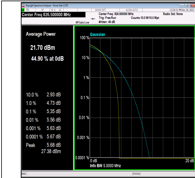
Band5-5MHz-64QAM-20425-1RB#0-PASS
