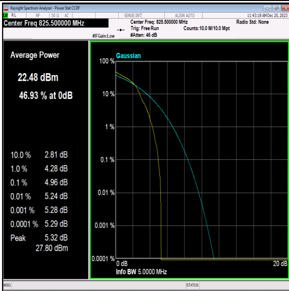
Band5-3MHz-16QAM-20415-1RB#0-PASS
