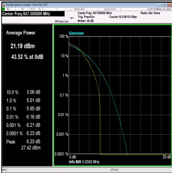
Band5-3MHz-64QAM-20635-1RB#0-PASS
