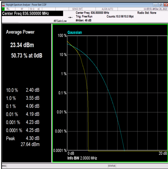
Band5-1.4MHz-QPSK-20525-1RB#0-PASS
