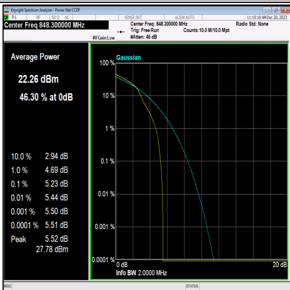
Band5-1.4MHz-16QAM-20643-1RB#0-PASS
