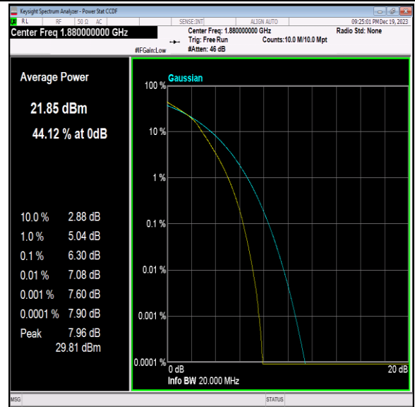
Band2-20MHz-16QAM-18900-100RB#0-PASS
