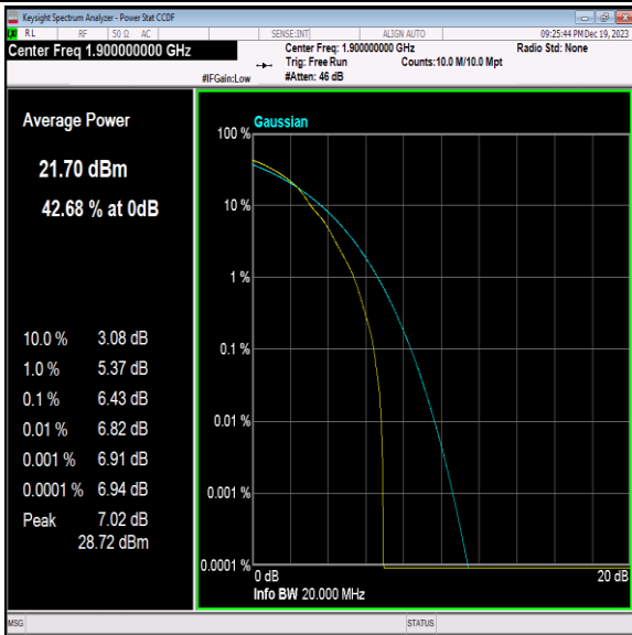
Band2-20MHz-64QAM-19100-1RB#0-PASS
