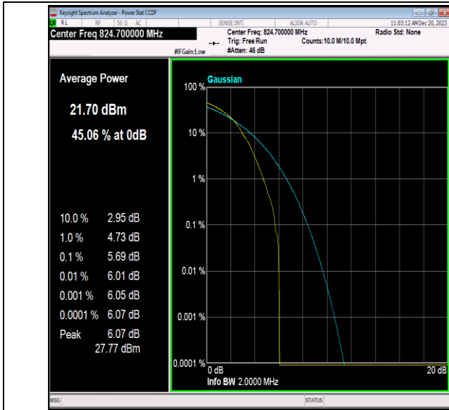
Band5-1.4MHz-64QAM-20407-1RB#0-PASS
