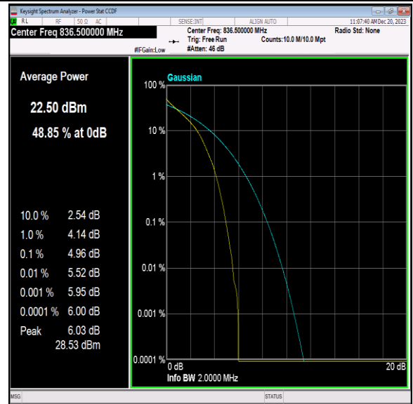
Band5-1.4MHz-QPSK-20525-6RB#0-PASS
