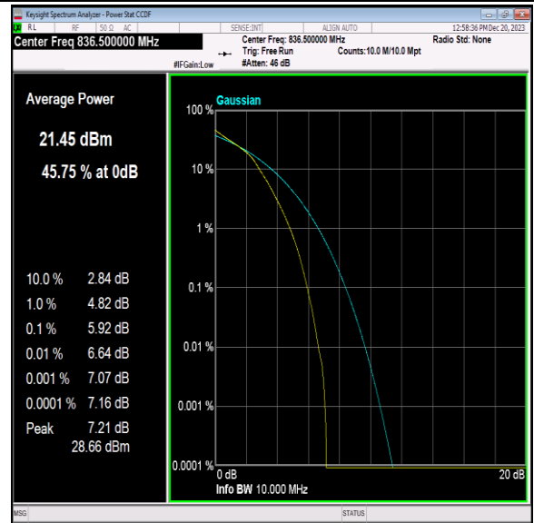
Band5-10MHz-16QAM-20525-50RB#0-PASS
