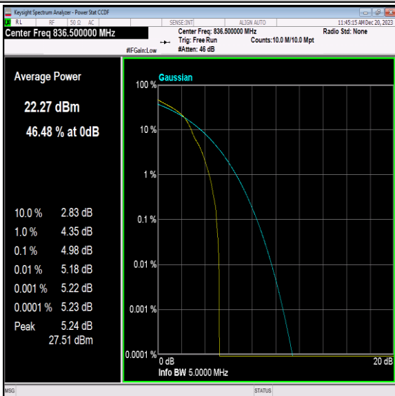
Band5-3MHz-16QAM-20525-1RB#0-PASS
