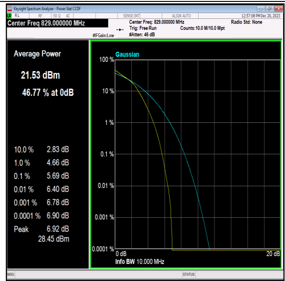
Band5-10MHz-16QAM-20450-50RB#0-PASS
