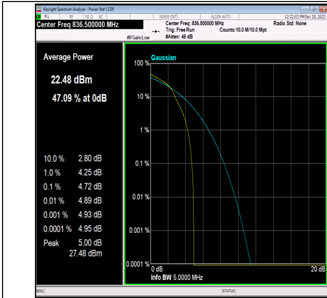
Band5-5MHz-16QAM-20525-1RB#0-PASS
