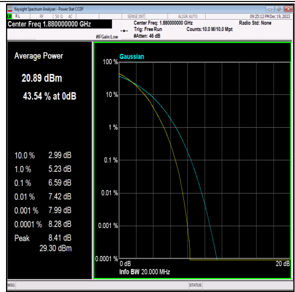
Band2-20MHz-64QAM-18900-100RB#0-PASS
