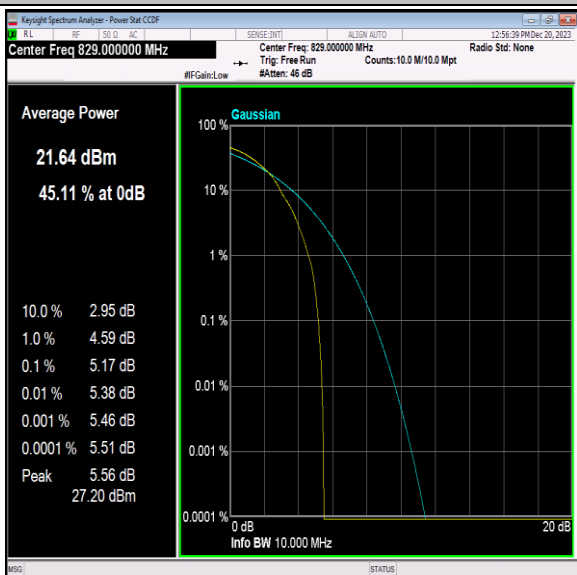
Band5-10MHz-64QAM-20450-1RB#0-PASS
